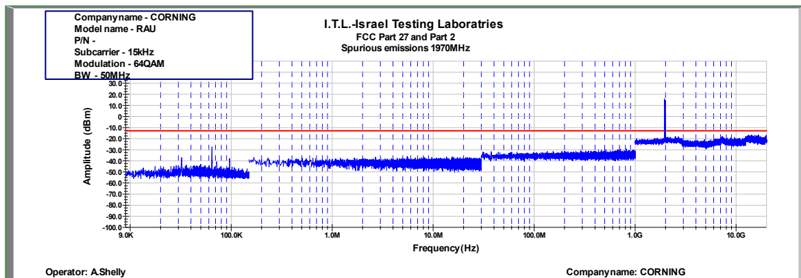
Figure 920: Spurious Emissions at Antenna Terminal 64QAM 50MHz B.W.; 1970.0MHz, 15kHz
