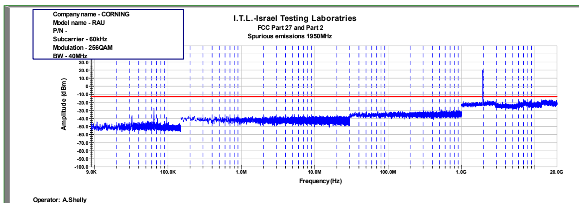
Figure 981: Spurious Emissions at Antenna Terminal 256QAM 40MHz B.W.; 1950.0MHz, 60kHz
