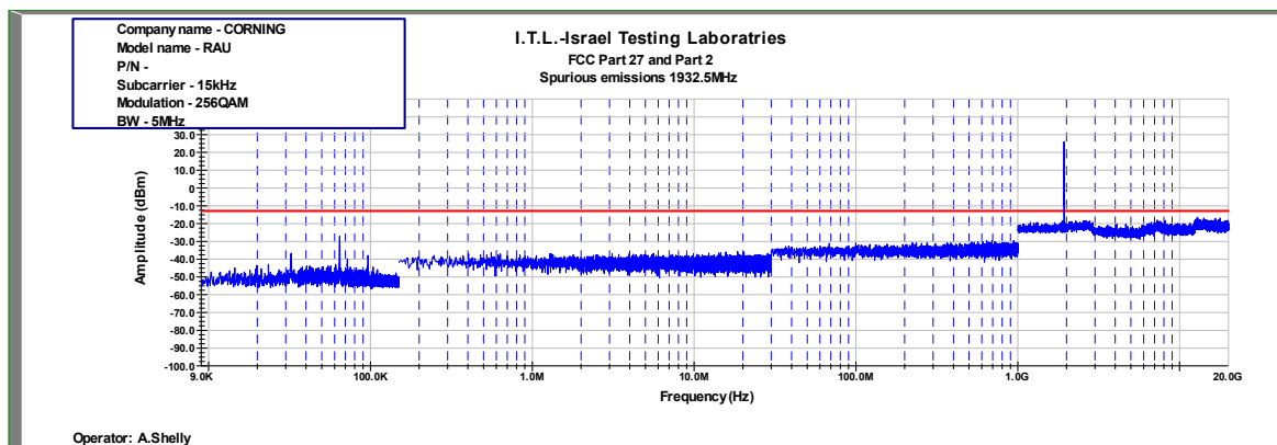
Figure 933: Spurious Emissions at Antenna Terminal 256QAM 5MHz B.W.; 1932.5MHz, 15kHz
