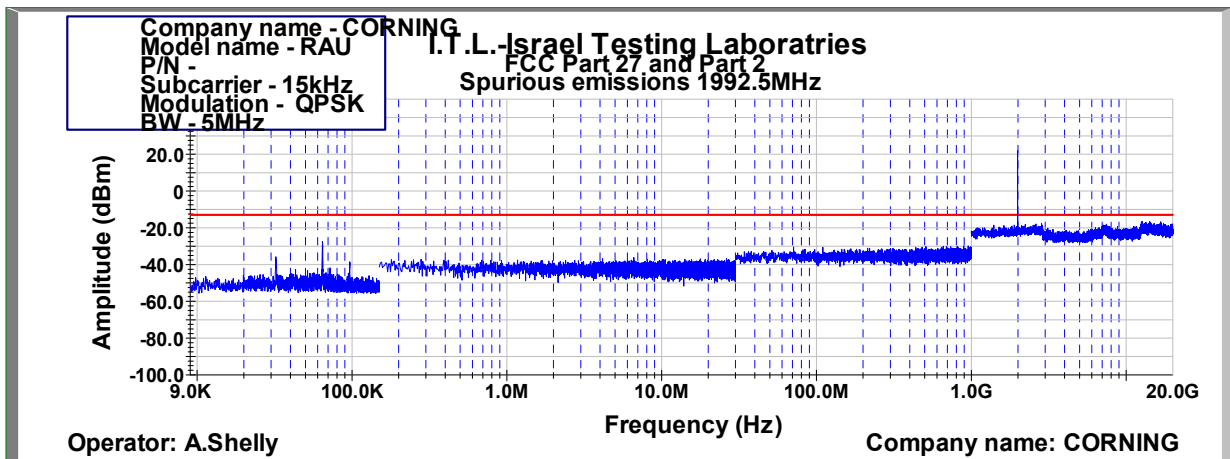
Figure 1001: Spurious Emissions at Antenna Terminal QPSK 5MHz B.W.; 1992.5MHz, 15kHz
