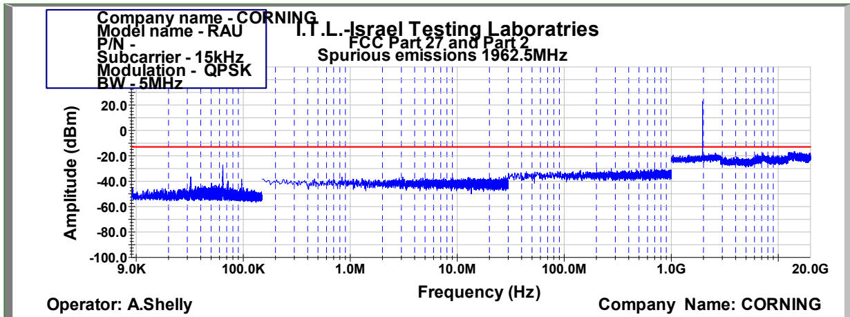
Figure 1000: Spurious Emissions at Antenna Terminal QPSK 5MHz B.W.; 1962.5MHz, 15kHz
