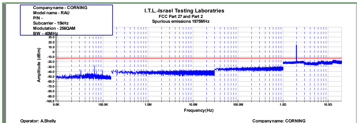
Figure 977: Spurious Emissions at Antenna Terminal 256QAM 40MHz B.W.; 1975.0MHz, 15kHz
