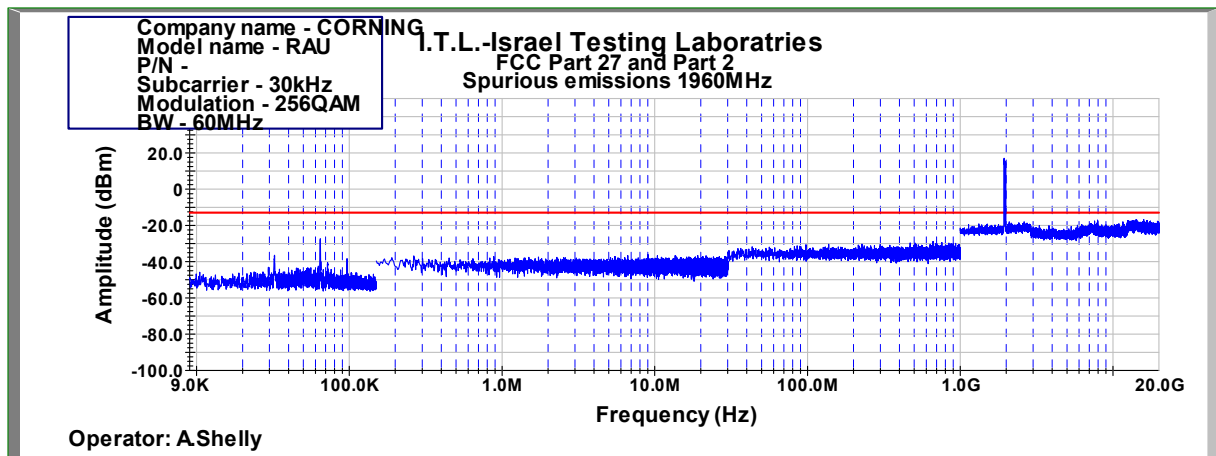
Figure 993: Spurious Emissions at Antenna Terminal 256QAM 60MHz B.W.; 1960.0MHz, 30kHz
