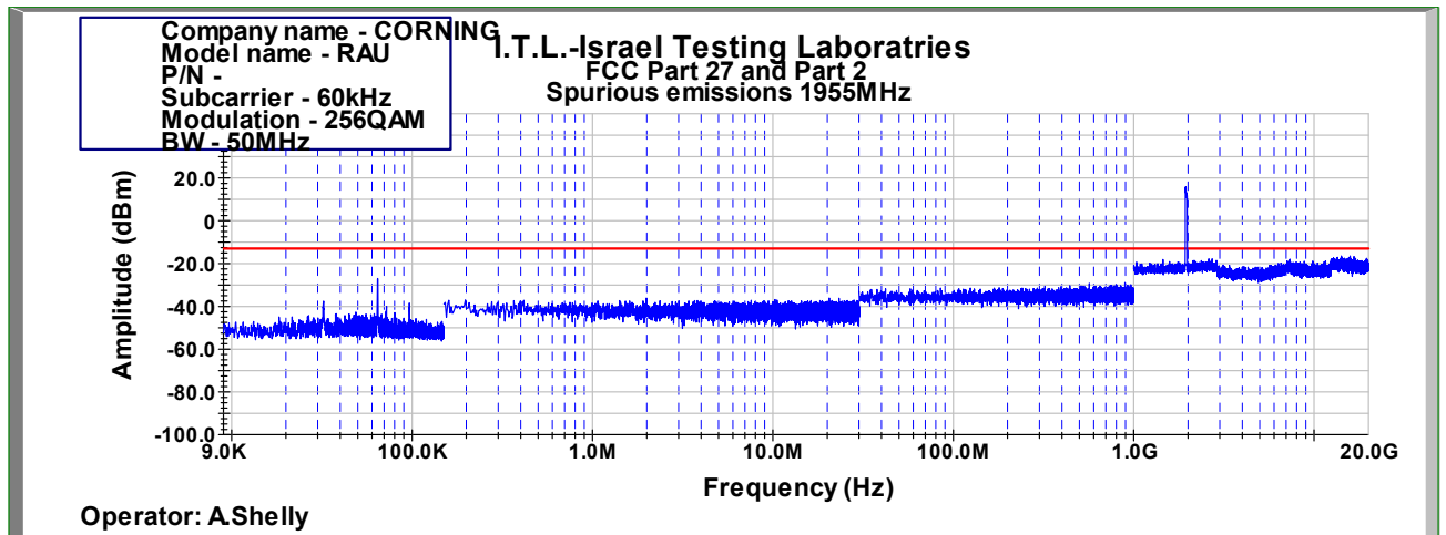
Figure 990: Spurious Emissions at Antenna Terminal 256QAM 50MHz B.W.; 1955.0MHz, 60kHz
