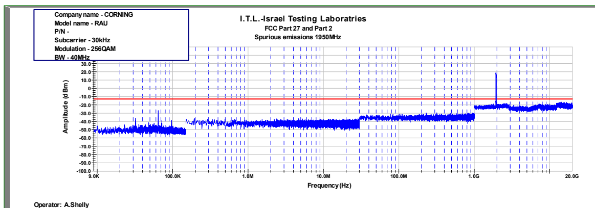
Figure 978: Spurious Emissions at Antenna Terminal 256QAM 40MHz B.W.; 1950.0MHz, 30kHz
