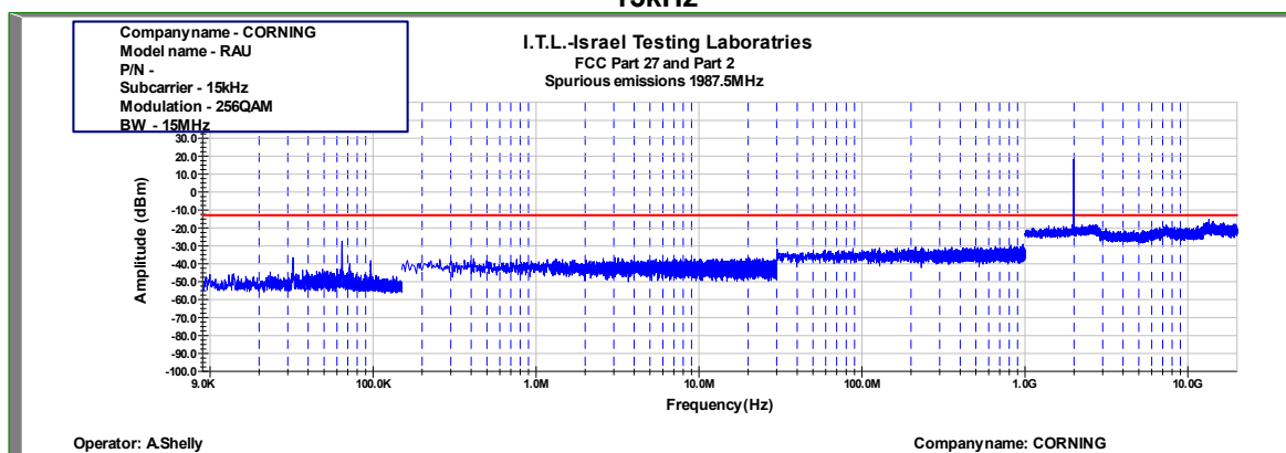
Figure 950: Spurious Emissions at Antenna Terminal 256QAM 15MHz B.W.; 1987.5MHz, 15kHz
