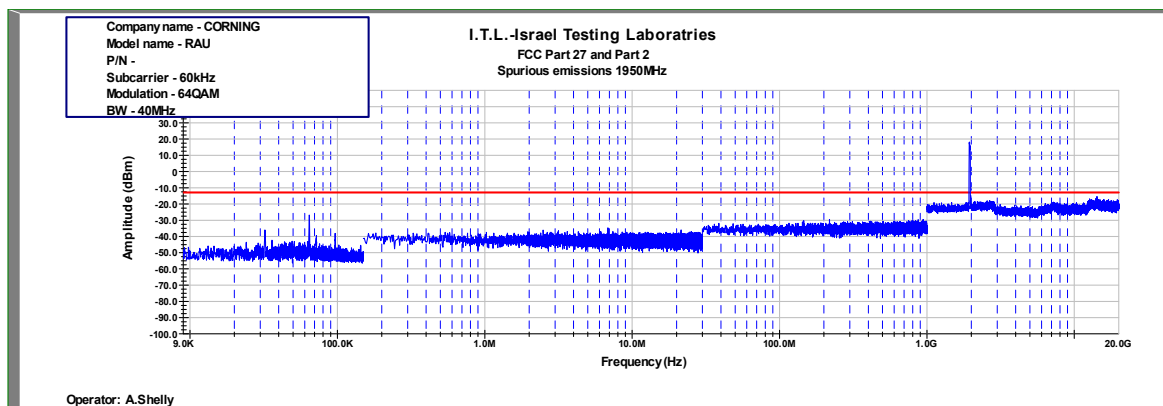
Figure 915: Spurious Emissions at Antenna Terminal 64QAM 40MHz B.W.; 1950.0MHz, 60kHz
