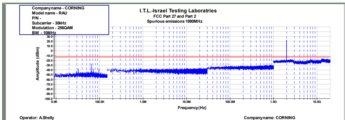
Figure 944: Spurious Emissions at Antenna Terminal 256QAM 10MHz B.W.; 1990.0MHz, 30kHz
