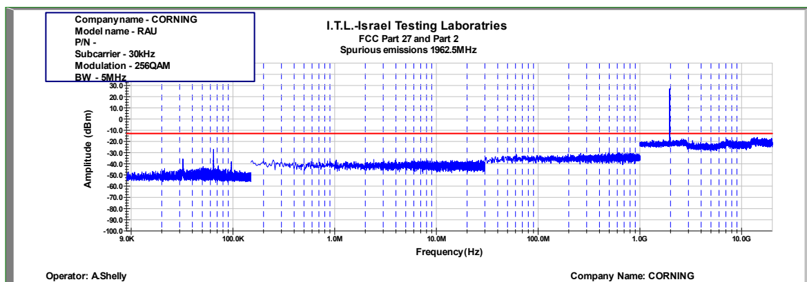
Figure 937: Spurious Emissions at Antenna Terminal 256QAM 5MHz B.W.; 1962.5MHz, 30kHz
