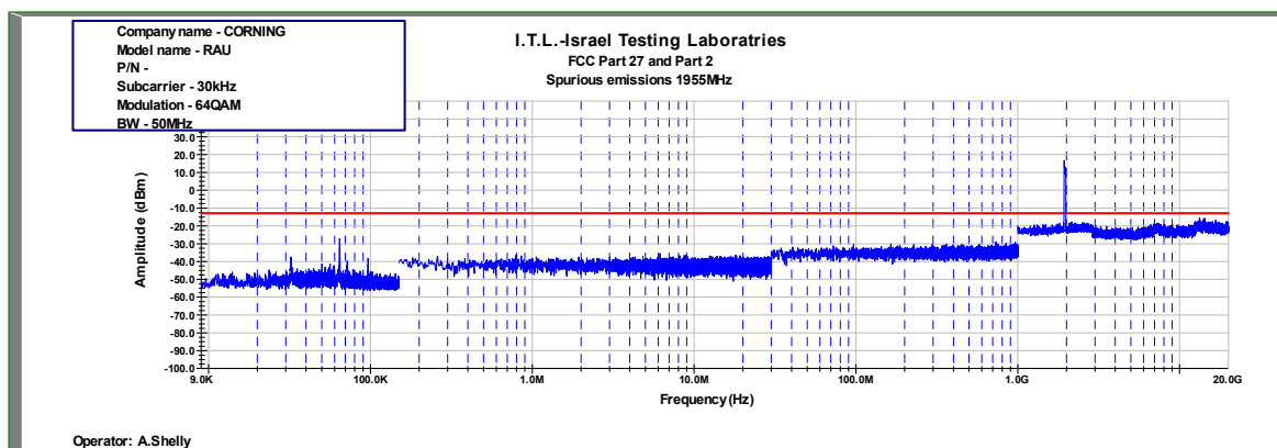
Figure 921: Spurious Emissions at Antenna Terminal 64QAM 50MHz B.W.; 1955.0MHz, 30kHz
