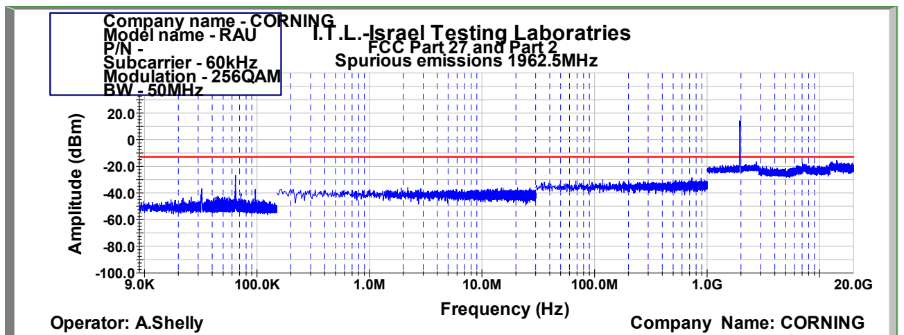
Figure 991: Spurious Emissions at Antenna Terminal 256QAM 50MHz B.W.; 1962.5MHz, 60kHz
