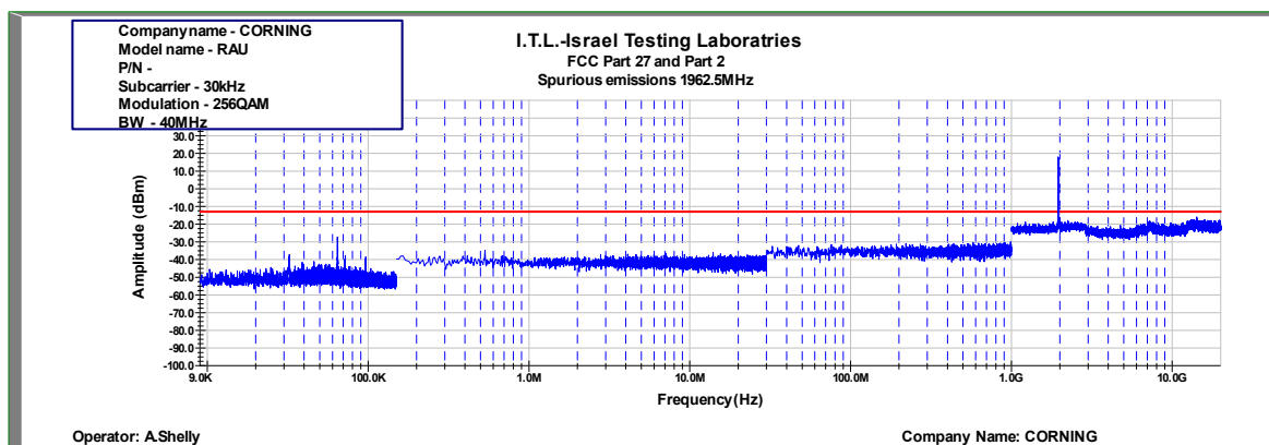
Figure 979: Spurious Emissions at Antenna Terminal 256QAM 40MHz B.W.; 1962.5MHz, 30kHz
