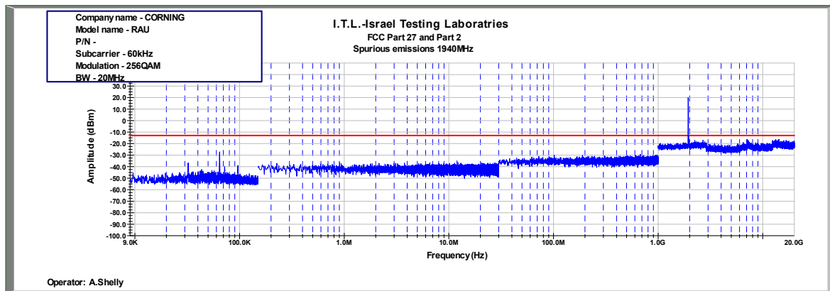
Figure 963: Spurious Emissions at Antenna Terminal 256QAM 20MHz B.W.; 1940.0MHz, 60kHz
