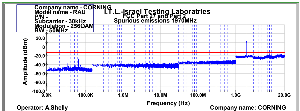
Figure 989: Spurious Emissions at Antenna Terminal 256QAM 50MHz B.W.; 1970.0MHz, 30kHz
