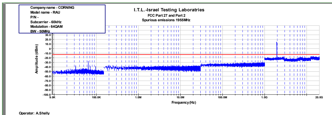
Figure 924: Spurious Emissions at Antenna Terminal 64QAM 50MHz B.W.; 1955.0MHz, 60kHz
