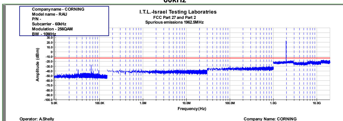
Figure 946: Spurious Emissions at Antenna Terminal 256QAM 10MHz B.W.; 1962.5MHz, 60kHz
