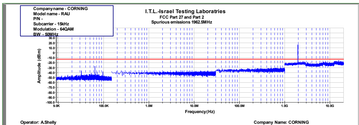
Figure 919: Spurious Emissions at Antenna Terminal 64QAM 50MHz B.W.; 1962.50MHz, 15kHz
