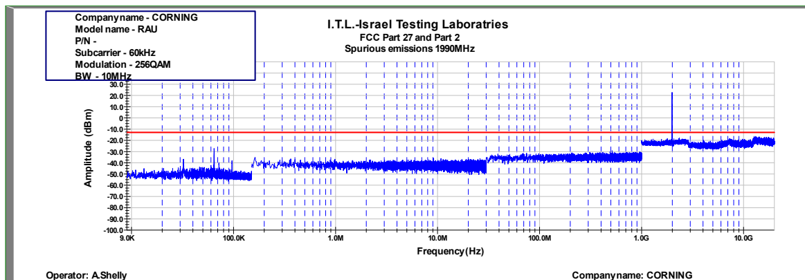
Figure 947: Spurious Emissions at Antenna Terminal 256QAM 10MHz B.W.; 1990.0MHz, 60kHz
