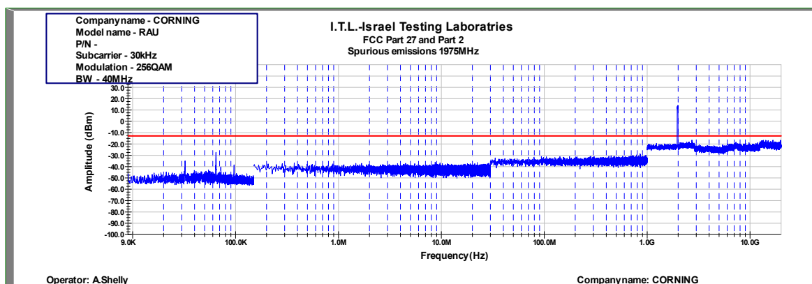
Figure 980: Spurious Emissions at Antenna Terminal 256QAM 40MHz B.W.; 1975.0MHz, 30kHz
