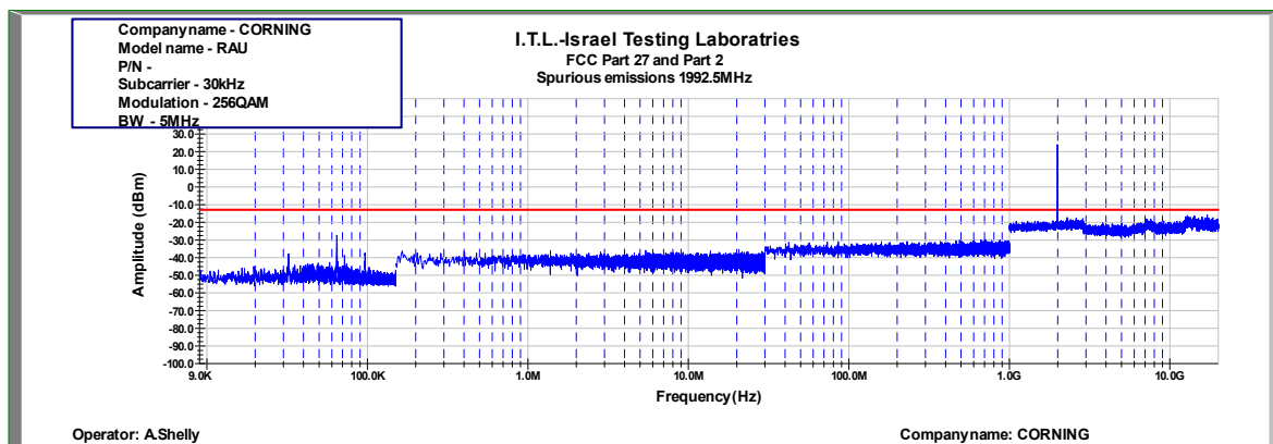
Figure 938: Spurious Emissions at Antenna Terminal 256QAM 5MHz B.W.; 1992.5MHz, 30kHz
