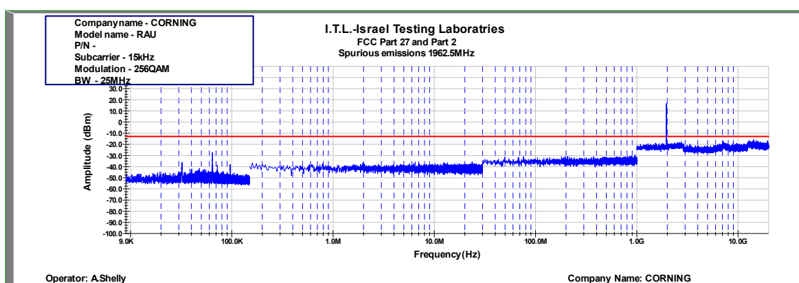
Figure 967: Spurious Emissions at Antenna Terminal 256QAM 25MHz B.W.; 1962.5MHz, 15kHz
