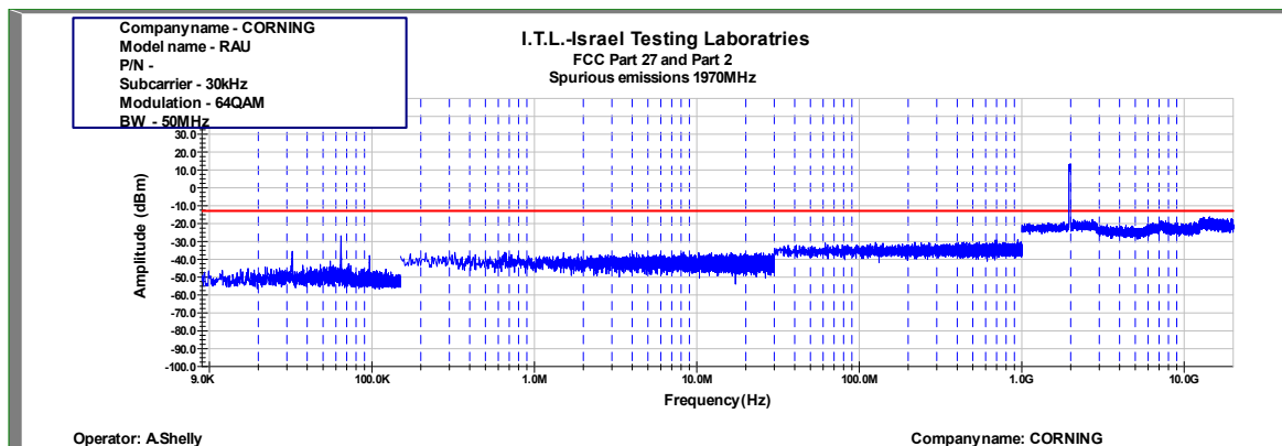
Figure 923: Spurious Emissions at Antenna Terminal 64QAM 50MHz B.W.; 1970.0MHz, 30kHz
