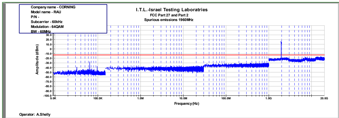
Figure 930: Spurious Emissions at Antenna Terminal 64QAM 60MHz B.W.; 1960.0MHz, 60kHz
