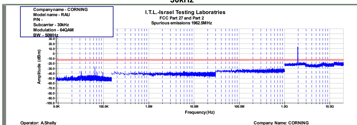
Figure 922: Spurious Emissions at Antenna Terminal 64QAM 50MHz B.W.; 1962.5MHz, 30kHz
