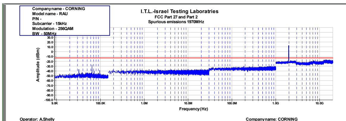
Figure 986: Spurious Emissions at Antenna Terminal 256QAM 50MHz B.W.; 1970.0MHz, 15kHz
