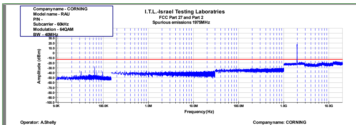
Figure 917: Spurious Emissions at Antenna Terminal 64QAM 40MHz B.W.; 1975.0MHz, 60kHz
