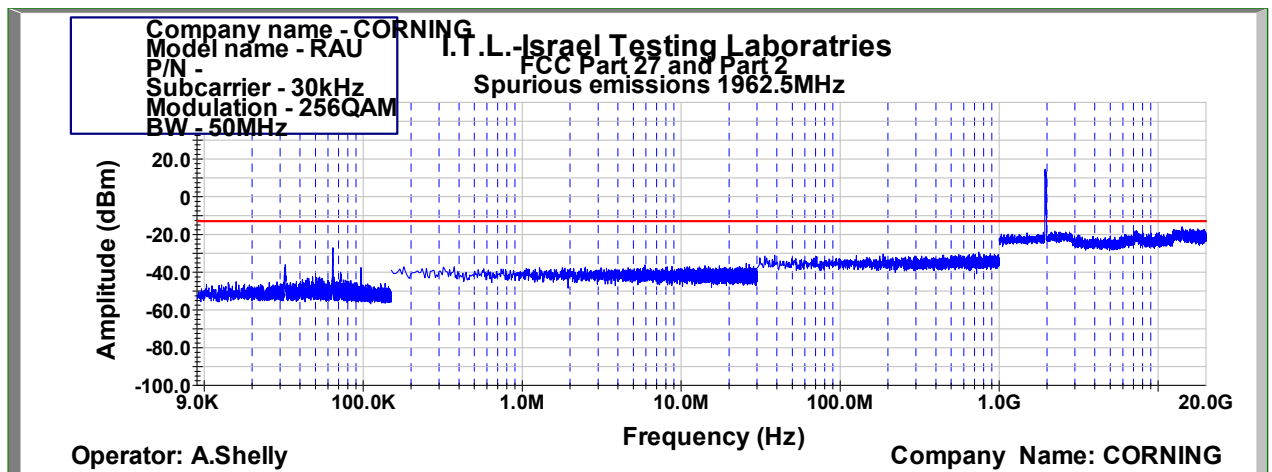
Figure 988: Spurious Emissions at Antenna Terminal 256QAM 50MHz B.W.; 1962.5MHz, 30kHz
