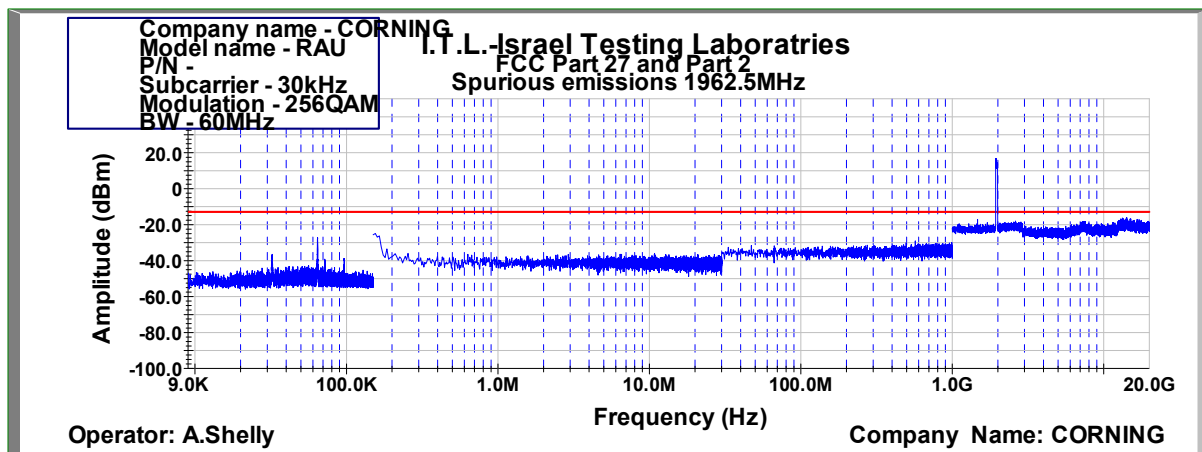
Figure 994: Spurious Emissions at Antenna Terminal 256QAM 60MHz B.W.; 1962.5MHz, 30kHz
