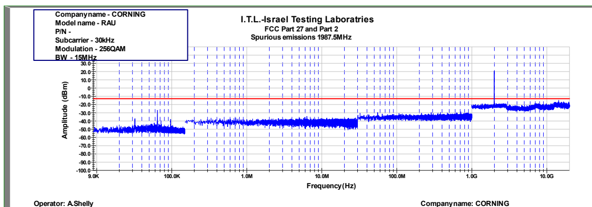
Figure 953: Spurious Emissions at Antenna Terminal 256QAM 15MHz B.W.; 1987.5MHz, 30kHz
