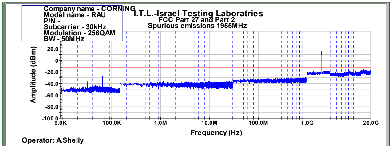
Figure 987: Spurious Emissions at Antenna Terminal 256QAM 50MHz B.W.; 1955.0MHz, 30kHz
