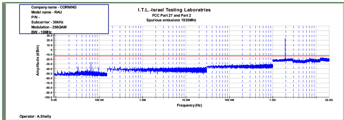
Figure 942: Spurious Emissions at Antenna Terminal 256QAM 10MHz B.W.; 1935.0MHz, 30kHz
