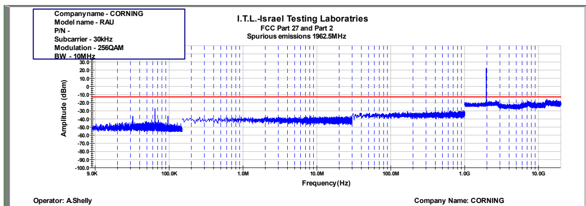
Figure 943: Spurious Emissions at Antenna Terminal 256QAM 10MHz B.W.; 1962.5MHz, 30kHz
