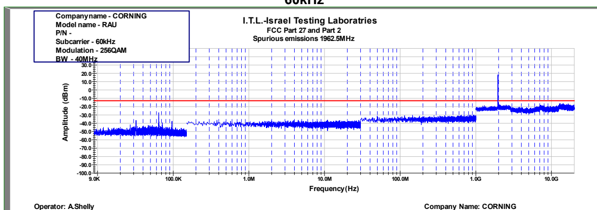
Figure 982: Spurious Emissions at Antenna Terminal 256QAM 40MHz B.W.; 1962.5MHz, 60kHz
