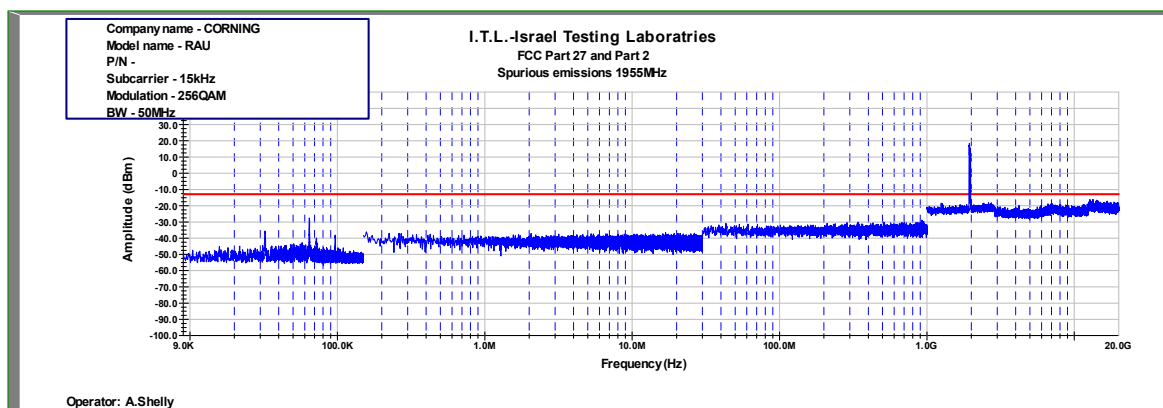
Figure 984: Spurious Emissions at Antenna Terminal 256QAM 50MHz B.W.; 1955.0MHz, 15kHz
