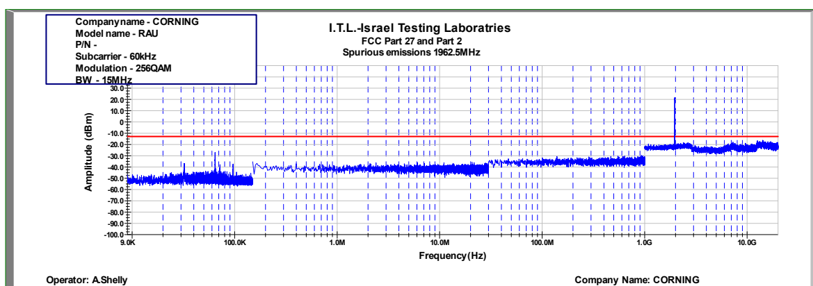
Figure 955: Spurious Emissions at Antenna Terminal 256QAM 15MHz B.W.; 1962.5MHz, 60kHz
