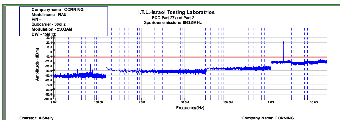
Figure 952: Spurious Emissions at Antenna Terminal 256QAM 15MHz B.W.; 1962.5MHz, 30kHz
