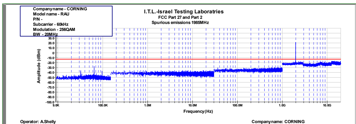
Figure 965: Spurious Emissions at Antenna Terminal 256QAM 20MHz B.W.; 1985.0MHz, 60kHz
