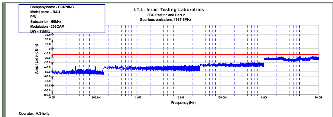
Figure 954: Spurious Emissions at Antenna Terminal 256QAM 15MHz B.W.; 1937.5MHz, 60kHz
