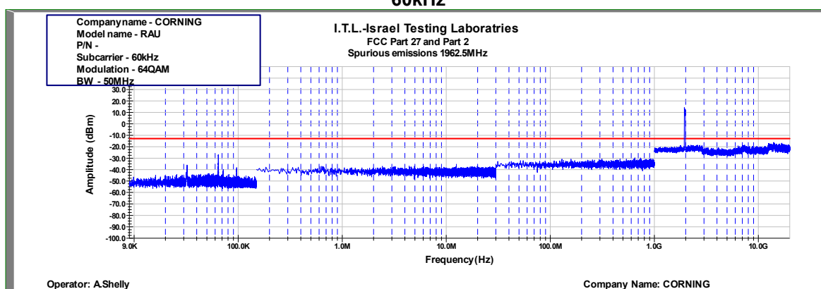
Figure 925: Spurious Emissions at Antenna Terminal 64QAM 50MHz B.W.; 1962.50MHz, 60kHz
