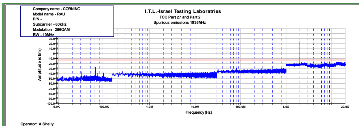
Figure 945: Spurious Emissions at Antenna Terminal 256QAM 10MHz B.W.; 1935.0MHz, 60kHz
