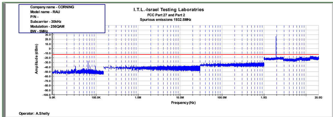
Figure 936: Spurious Emissions at Antenna Terminal 256QAM 5MHz B.W.; 1932.5MHz, 30kHz
