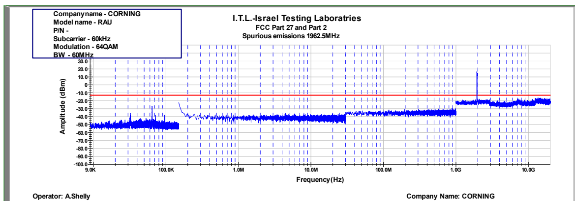
Figure 931: Spurious Emissions at Antenna Terminal 64QAM 60MHz B.W.; 1962.5MHz, 60kHz
