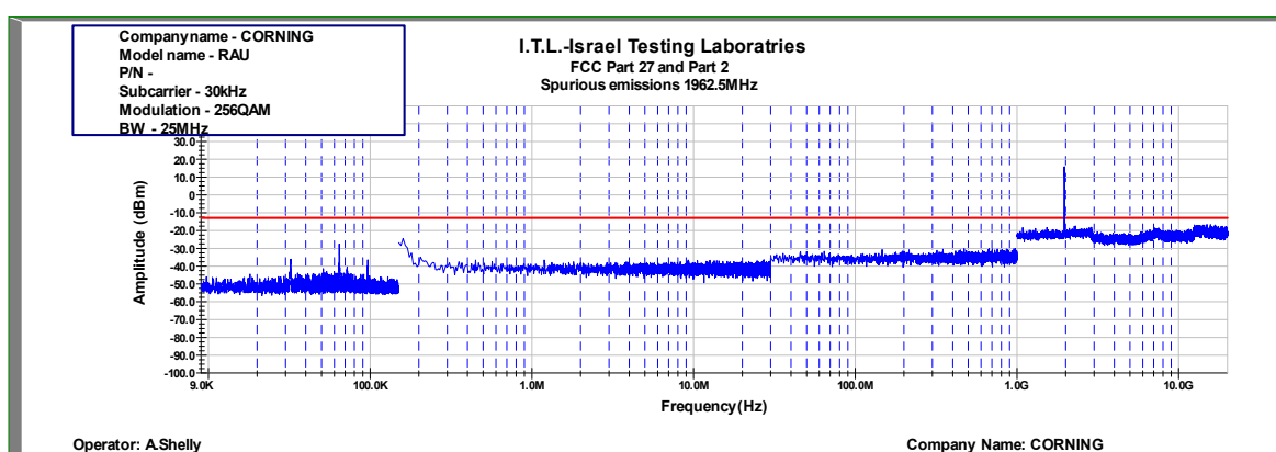
Figure 970: Spurious Emissions at Antenna Terminal 256QAM 25MHz B.W.; 1962.5MHz, 30kHz
