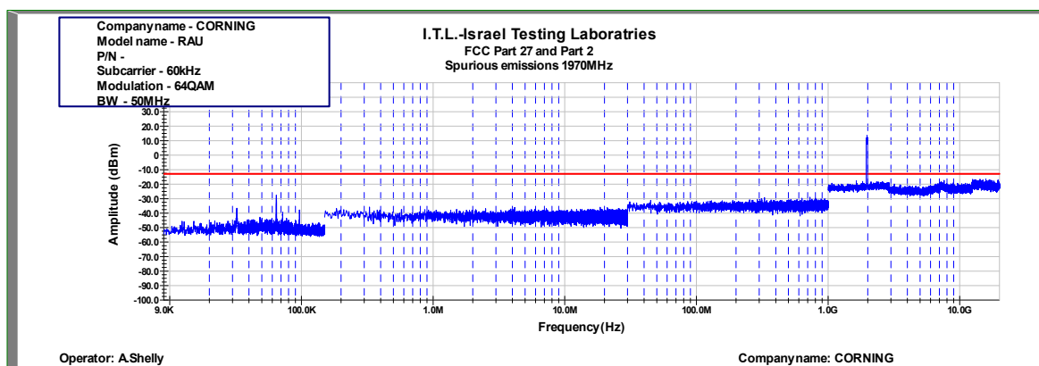
Figure 926: Spurious Emissions at Antenna Terminal 64QAM 50MHz B.W.; 1970.0MHz, 60kHz
