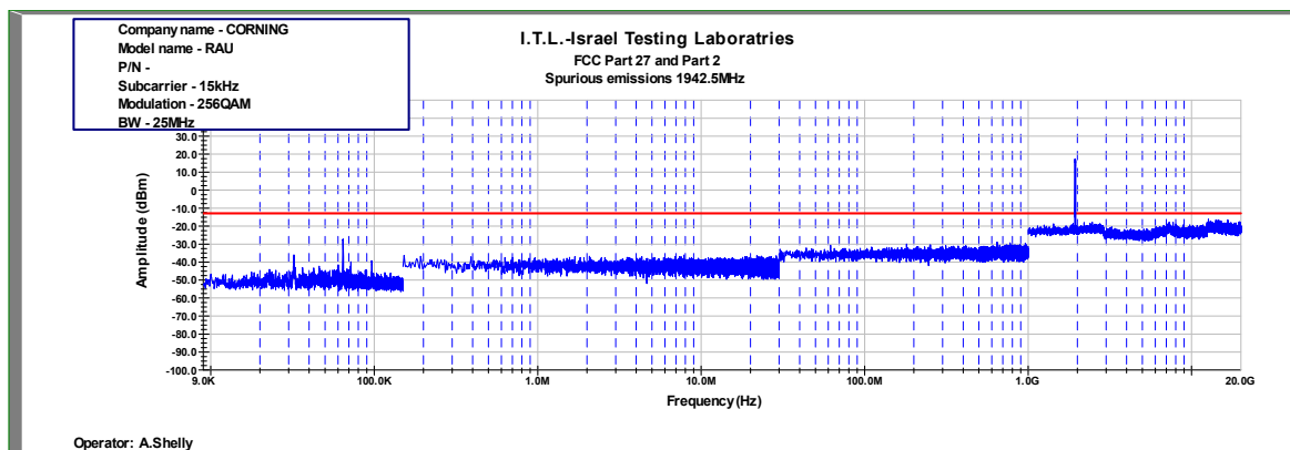
Figure 966: Spurious Emissions at Antenna Terminal 256QAM 25MHz B.W.; 1942.5MHz, 15kHz
