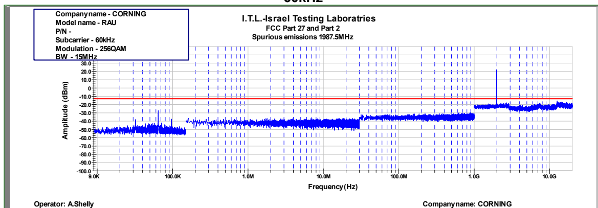
Figure 956: Spurious Emissions at Antenna Terminal 256QAM 15MHz B.W.; 1987.5MHz, 60kHz
