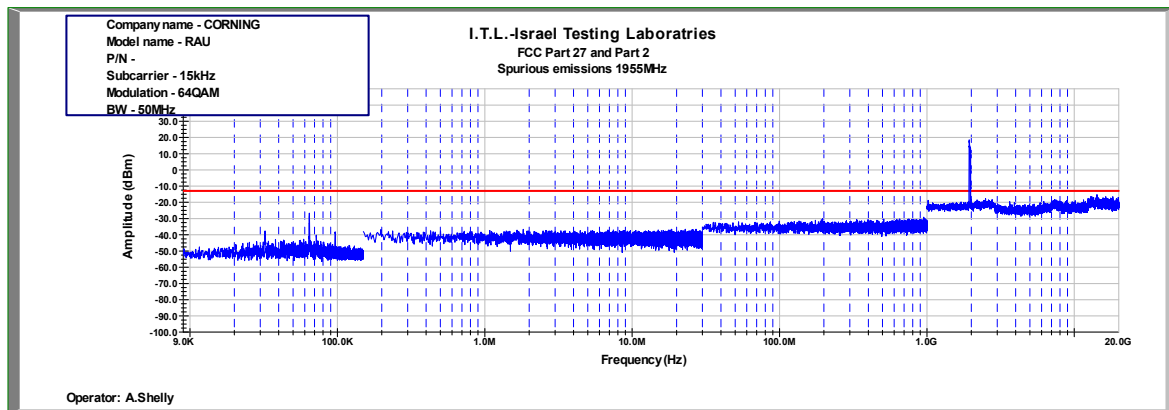
Figure 918: Spurious Emissions at Antenna Terminal 64QAM 50MHz B.W.; 1955.0MHz, 15kHz
