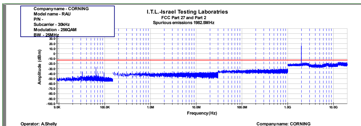
Figure 971: Spurious Emissions at Antenna Terminal 256QAM 25MHz B.W.; 1982.5MHz, 30kHz
