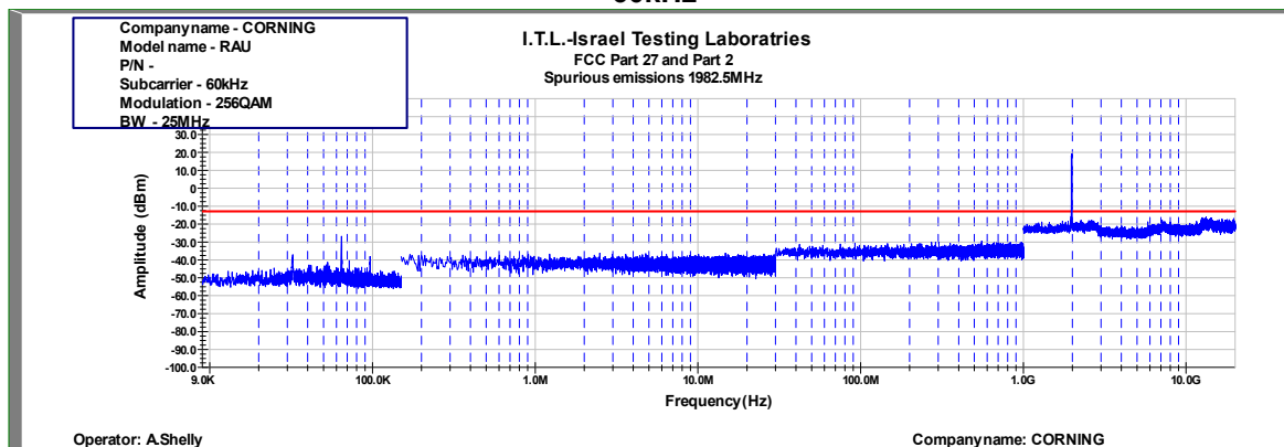
Figure 973: Spurious Emissions at Antenna Terminal 256QAM 25MHz B.W.; 1962.5MHz, 60kHz
