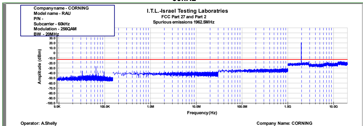
Figure 964: Spurious Emissions at Antenna Terminal 256QAM 20MHz B.W.; 1962.5MHz, 60kHz
