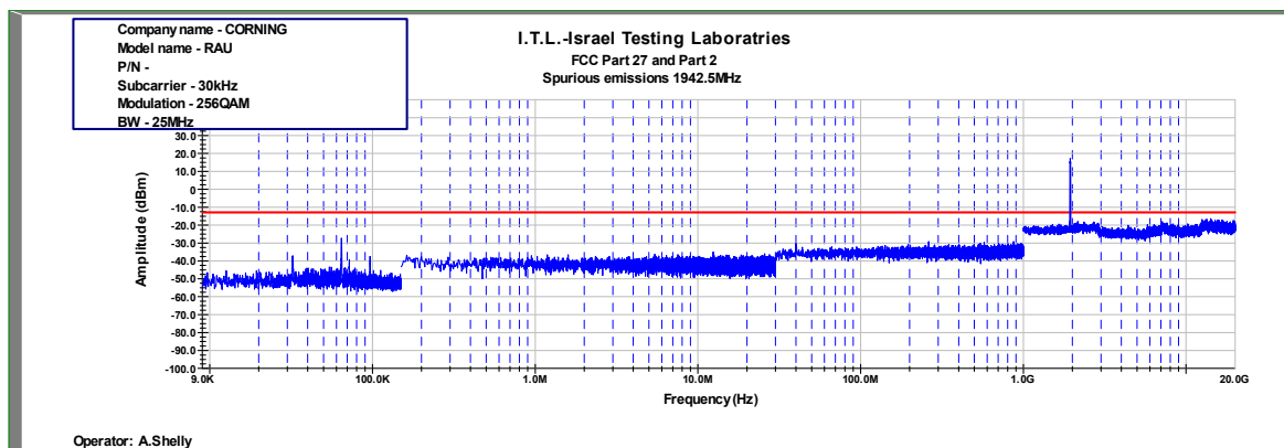
Figure 969: Spurious Emissions at Antenna Terminal 256QAM 25MHz B.W.; 1942.5MHz, 30kHz
