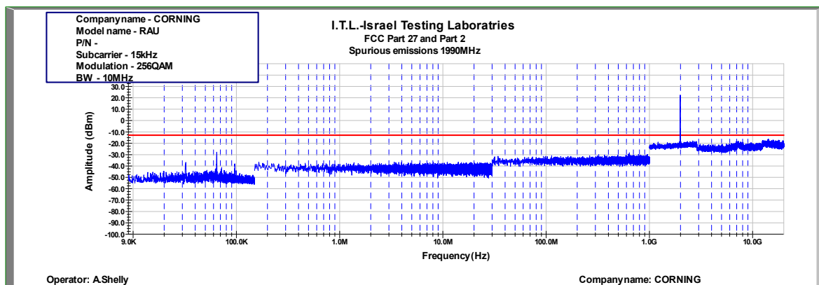
Figure 941: Spurious Emissions at Antenna Terminal 256QAM 10MHz B.W.; 1990.00MHz, 15kHz
