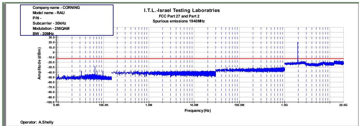
Figure 960: Spurious Emissions at Antenna Terminal 256QAM 20MHz B.W.; 1940.0MHz, 30kHz
