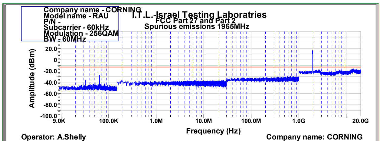
Figure 998: Spurious Emissions at Antenna Terminal 256QAM 60MHz B.W.; 1965.0MHz, 60kHz
