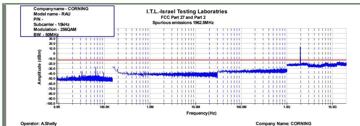
Figure 985: Spurious Emissions at Antenna Terminal 256QAM 50MHz B.W.; 1962.5MHz, 15kHz
