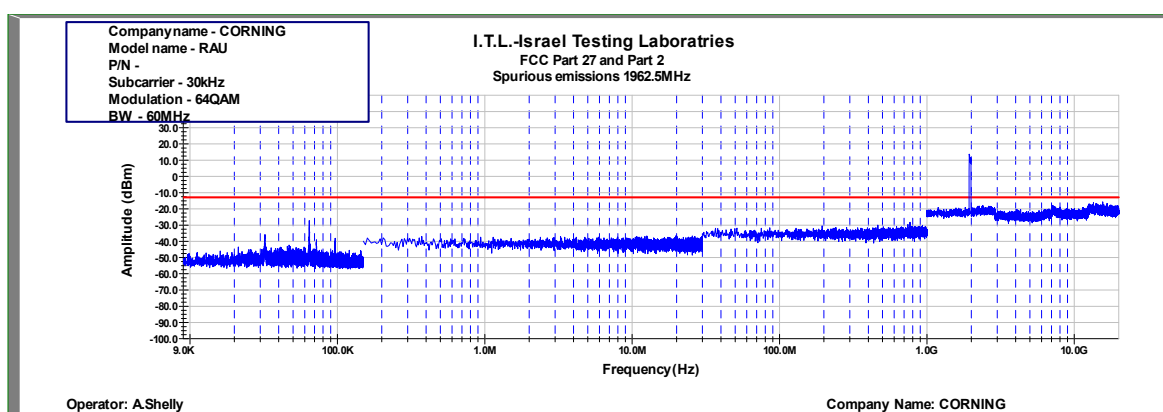
Figure 928: Spurious Emissions at Antenna Terminal 64QAM 60MHz B.W.; 1962.5MHz, 30kHz
