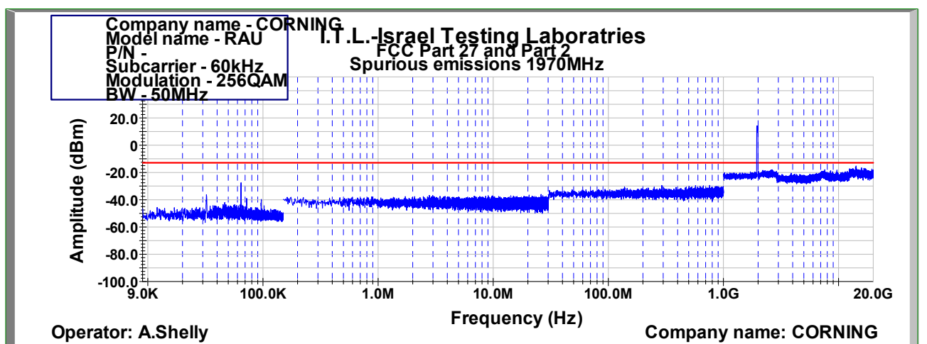
Figure 992: Spurious Emissions at Antenna Terminal 256QAM 50MHz B.W.; 1970.0MHz, 60kHz
