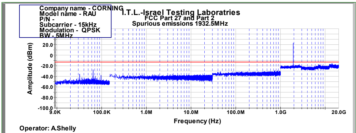
Figure 999: Spurious Emissions at Antenna Terminal QPSK 5MHz B.W.; 1932.5MHz, 15kHz
