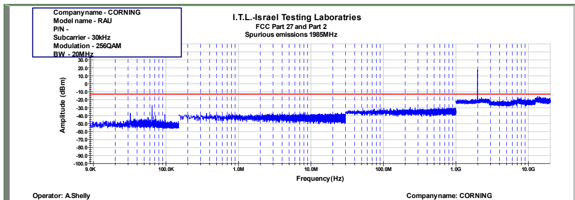
Figure 962: Spurious Emissions at Antenna Terminal 256QAM 20MHz B.W.; 1985.0MHz, 30kHz
