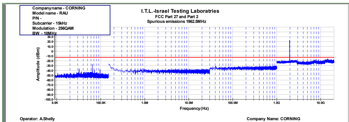
Figure 940: Spurious Emissions at Antenna Terminal 256QAM 10MHz B.W.; 1962.50MHz, 15kHz
