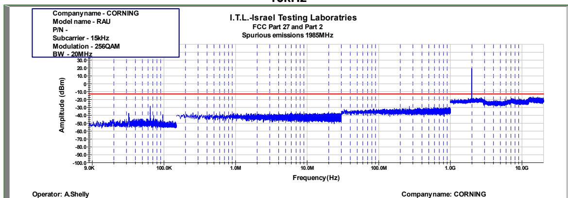
Figure 959: Spurious Emissions at Antenna Terminal 256QAM 20MHz B.W.; 1985.0MHz, 15kHz
