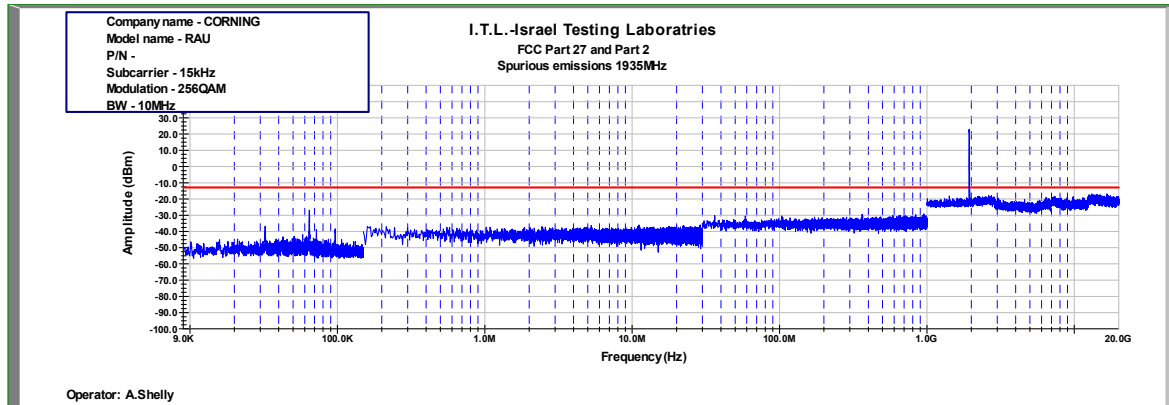
Figure 939: Spurious Emissions at Antenna Terminal 256QAM 10MHz B.W.; 1935.00MHz, 15kHz
