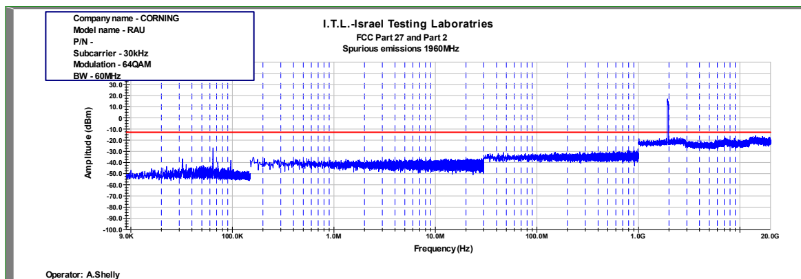
Figure 927: Spurious Emissions at Antenna Terminal 64QAM 60MHz B.W.; 1960.0MHz, 30kHz
