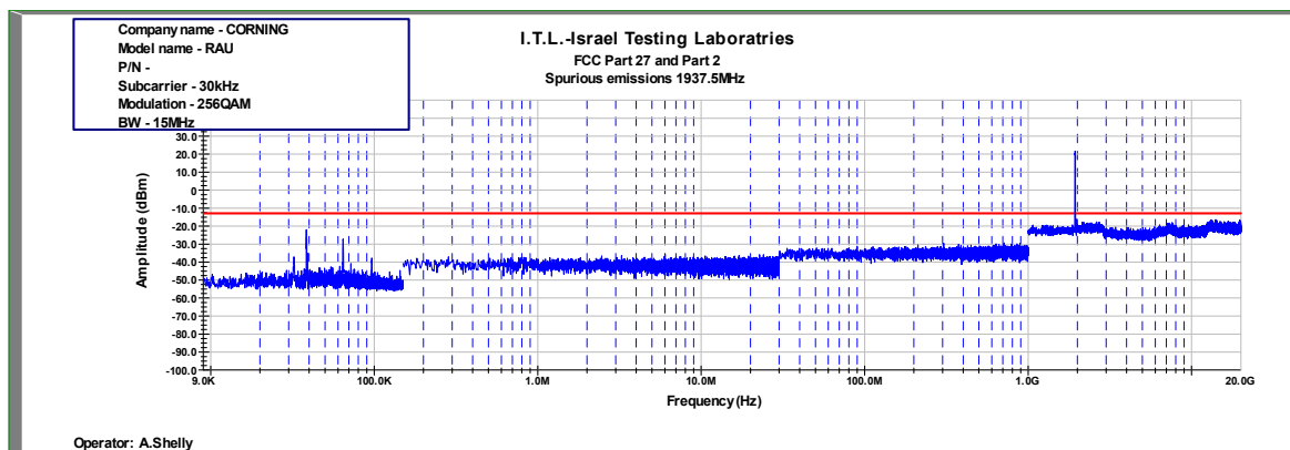
Figure 951: Spurious Emissions at Antenna Terminal 256QAM 15MHz B.W.; 1937.5MHz, 30kHz
