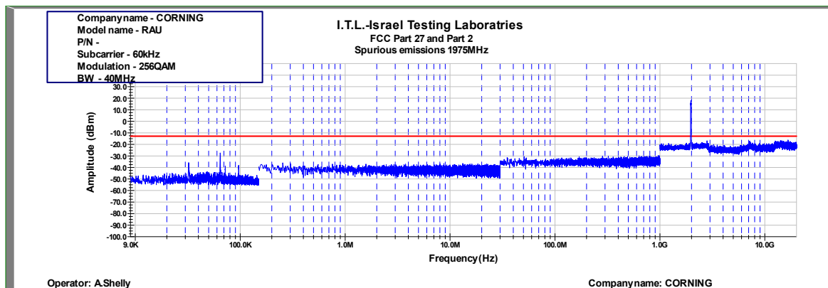
Figure 983: Spurious Emissions at Antenna Terminal 256QAM 40MHz B.W.; 1975.0MHz, 60kHz
