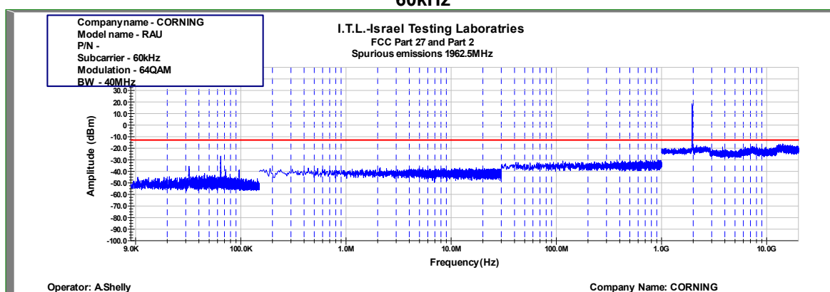
Figure 916: Spurious Emissions at Antenna Terminal 64QAM 40MHz B.W.; 1962.50MHz, 60kHz
