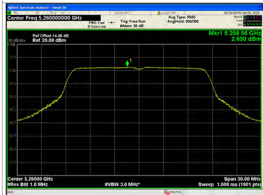
PSD NVNT a 5260MHz Ant2 SISO
