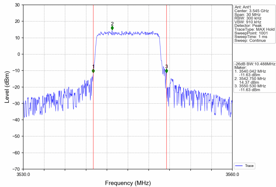
Band42a_10MHz_16QAM_HCH_3545MHz_RB_50_0_NTNV
