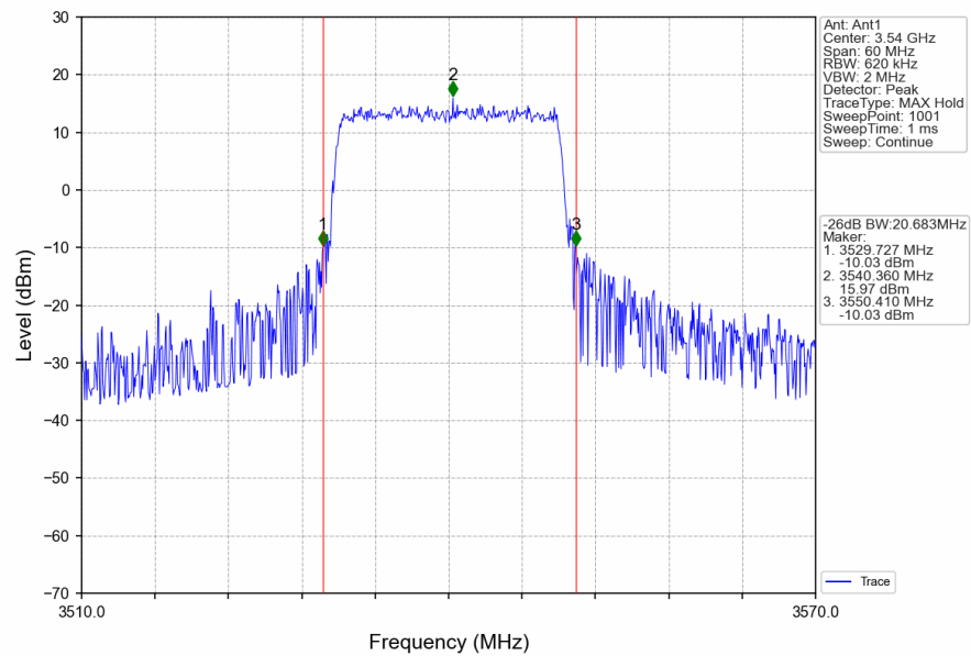
Band42a_20MHz_16QAM_HCH_3540MHz_RB_100_0_NTNV
