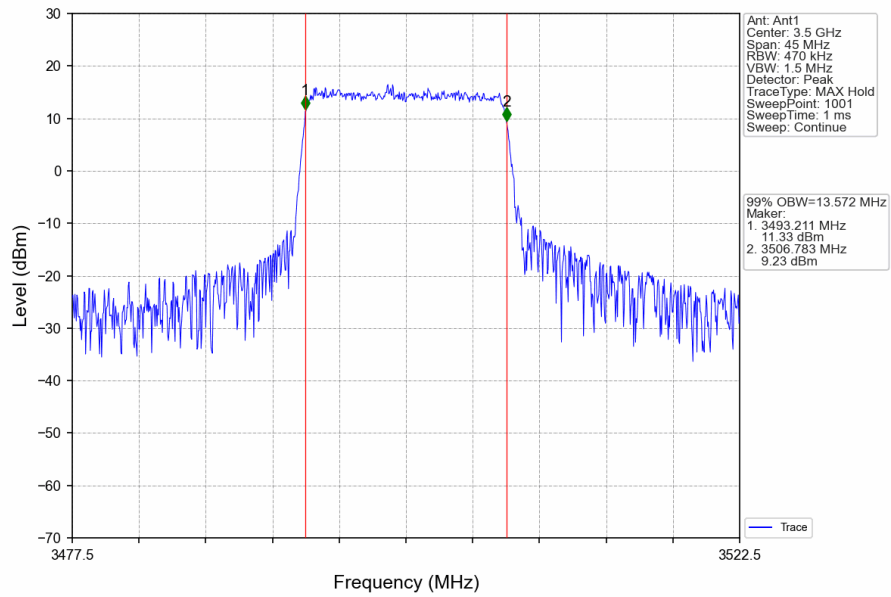
Band42a_15MHz_QPSK_MCH_3500MHz_RB_75_0_NTNV
