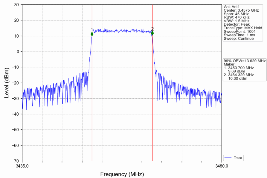
Band42a_15MHz_16QAM_LCH_3457.5MHz_RB_75_0_NTNV
