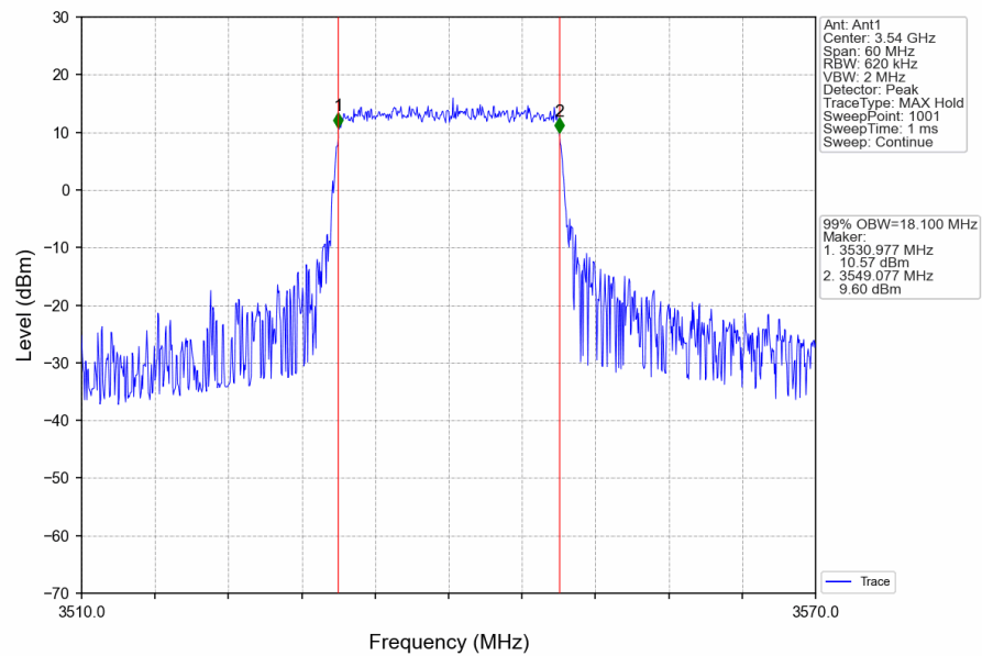
Band42a_20MHz_16QAM_HCH_3540MHz_RB_100_0_NTNV
