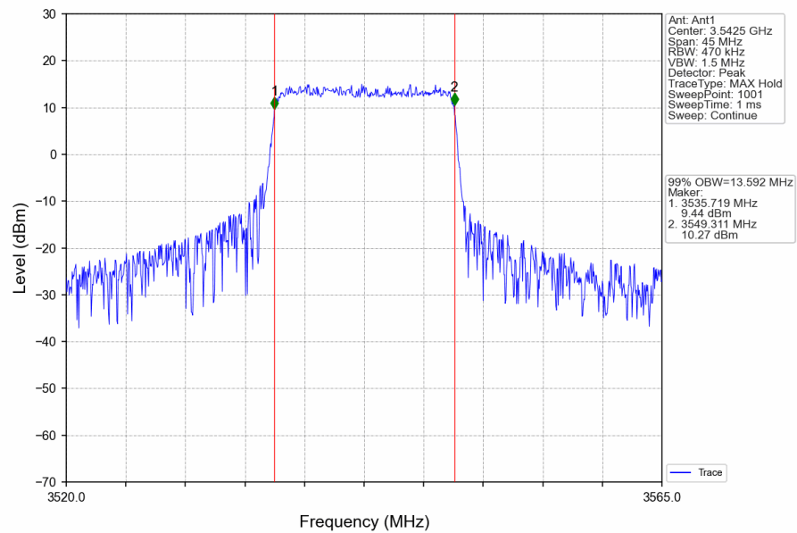
Band42a_15MHz_16QAM_HCH_3542.5MHz_RB_75_0_NTNV
