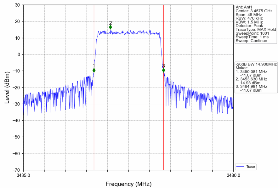
Band42a_15MHz_16QAM_LCH_3457.5MHz_RB_75_0_NTNV
