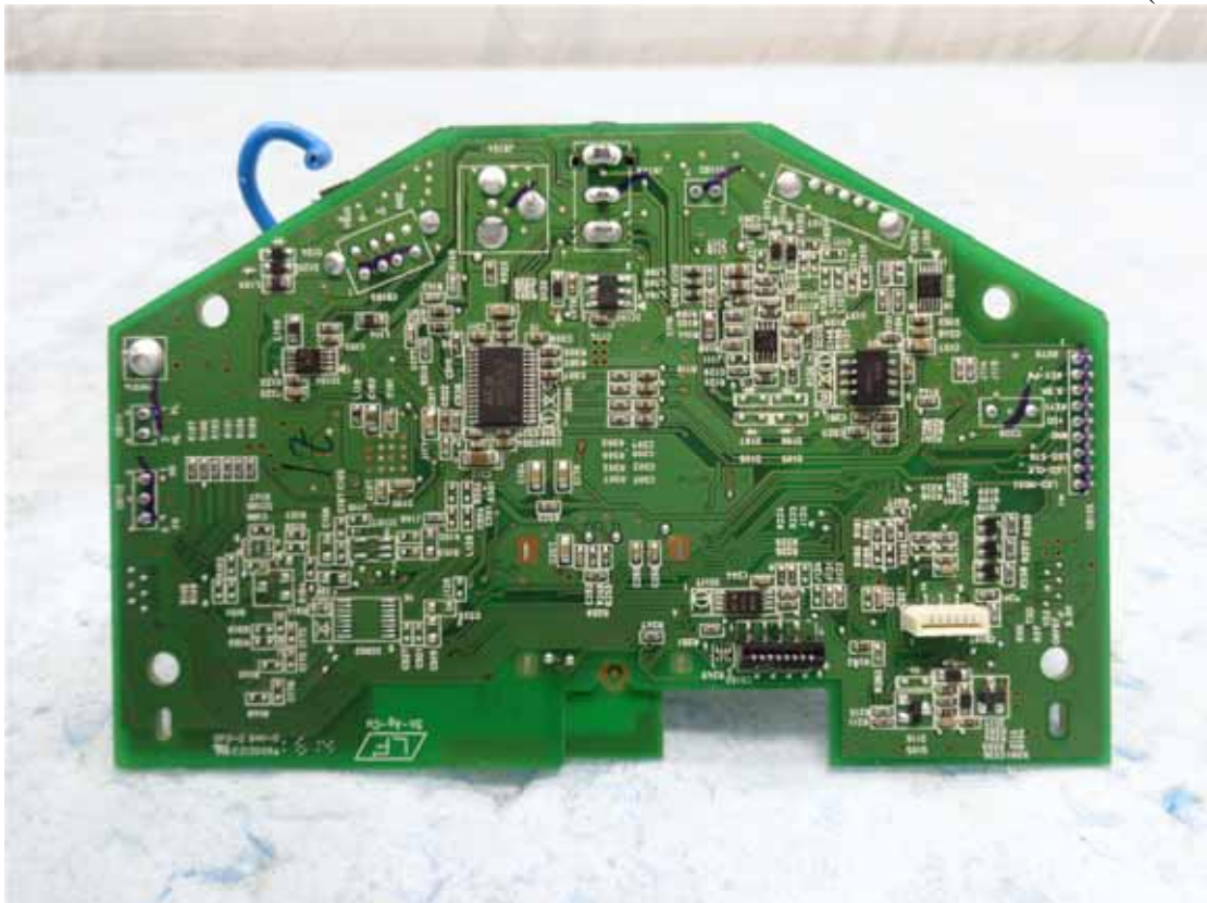
Figure 4 Main Board (Solder Side)
