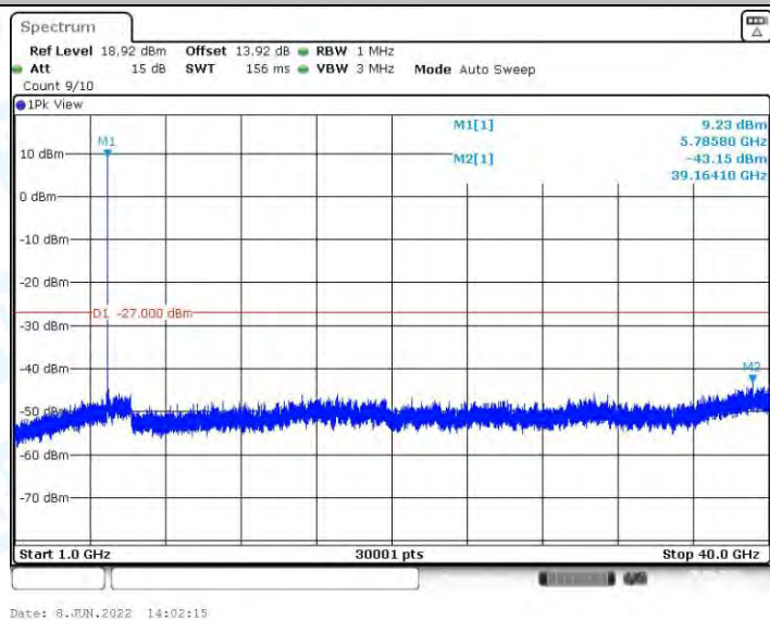
11AC20MIMO_Ant1_5785_1000~40000
