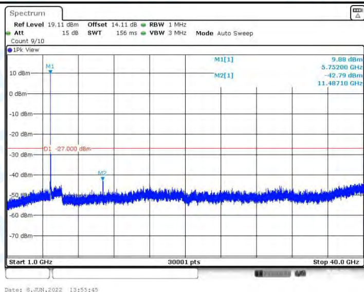
11AC20MIMO_Ant2_5745_1000~40000
