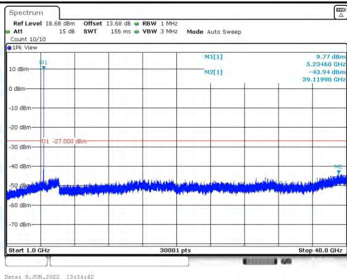
11AC20MIMO_Ant1_5240_1000~40000
