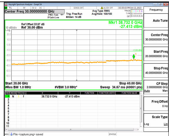
5A_n77(3700-3980MHz) (20GHz-40GHz) 30M DFT-s-OFDM BPSK Edge_1RB_Left Low
