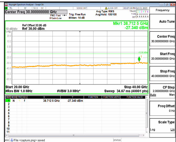
5A_n77(3700-3980MHz) (20GHz-40GHz) 15M DFT-s-OFDM QPSK Edge 1RB Left High
