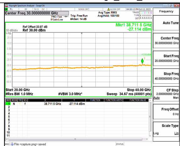
5A_n77(3700-3980MHz) (20GHz-40GHz) 40M DFT-s-OFDM BPSK Edge 1RB Right Low
