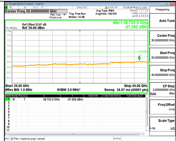
5A_n77(3700-3980MHz) (20GHz-40GHz) 30M DFT-s-OFDM QPSK Edge_1RB_Left Low
