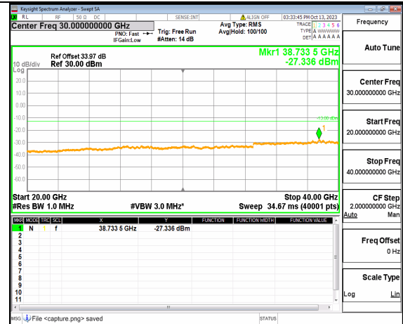
5A_n77(3700-3980MHz) (20GHz-40GHz) 30M DFT-s-OFDM BPSK Outer_Full Low
