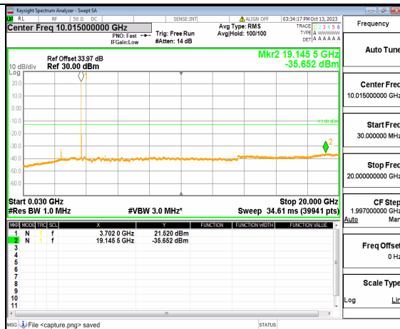
5A_n77(3700-3980MHz) (30MHz-20GHz) 30M DFT-s-OFDM BPSK Edge_1RB_Left Low
