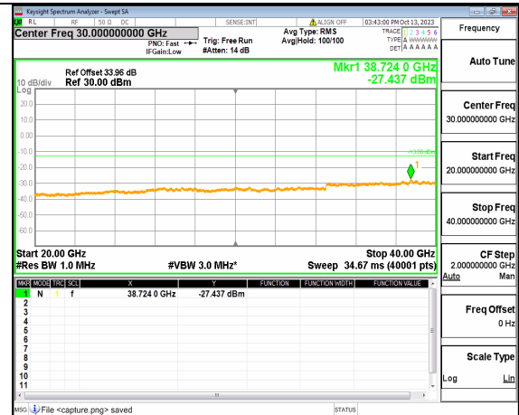
5A_n77(3700-3980MHz) (20GHz-40GHz) 30M DFT-s-OFDM BPSK Edge_1RB_Left Mid
