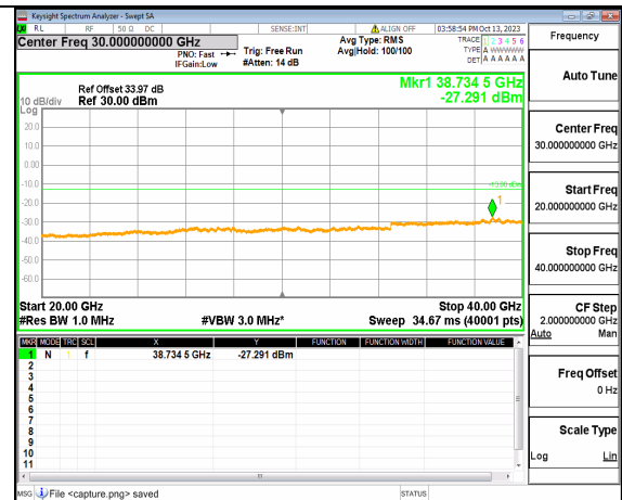
5A_n77(3700-3980MHz) (20GHz-40GHz) 40M DFT-s-OFDM BPSK Edge 1RB Left Low
