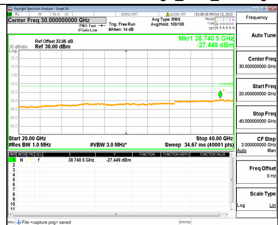
5A_n77(3700-3980MHz) (20GHz-40GHz) 15M DFT-s-OFDM QPSK Edge 1RB Right High
