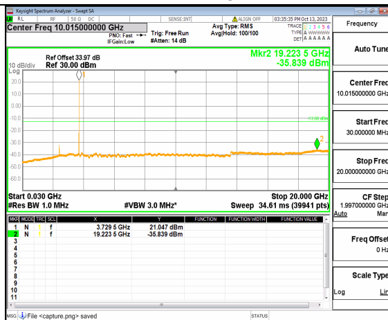
5A_n77(3700-3980MHz) (30MHz-20GHz) 30M DFT-s-OFDM BPSK Edge_1RB_Right Low
