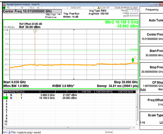
5A_n77(3700-3980MHz) (30MHz-20GHz) 15M DFT-s-OFDM QPSK Edge 1RB Left High
