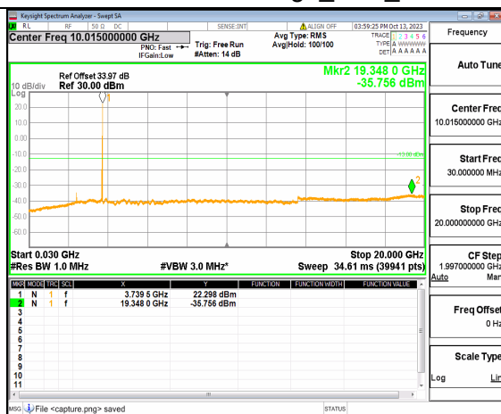
5A_n77(3700-3980MHz) (30MHz-20GHz) 40M DFT-s-OFDM BPSK Edge 1RB Right Low
