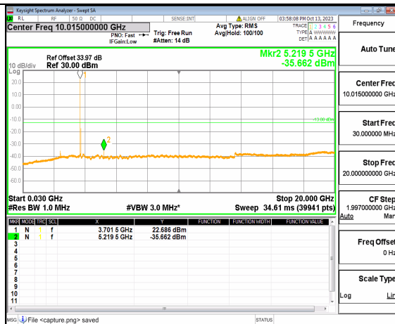
5A_n77(3700-3980MHz) (30MHz-20GHz) 40M DFT-s-OFDM BPSK Edge 1RB Left Low
