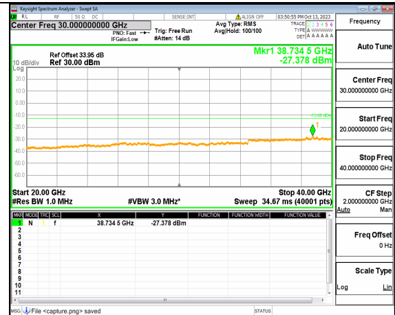
5A_n77(3700-3980MHz) (20GHz-40GHz) 30M DFT-s-OFDM BPSK Edge_1RB_Left High
