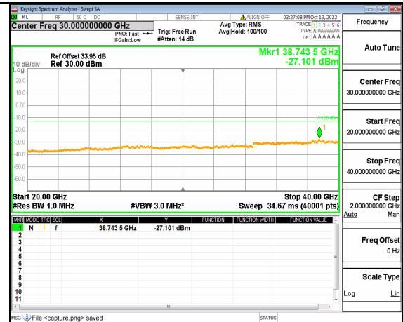
5A_n77(3700-3980MHz) (20GHz-40GHz) 20M DFT-s-OFDM BPSK Edge_1RB_Left High
