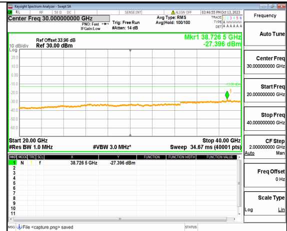
5A_n77(3700-3980MHz) (20GHz-40GHz) 30M DFT-s-OFDM QPSK Edge_1RB_Left Mid
