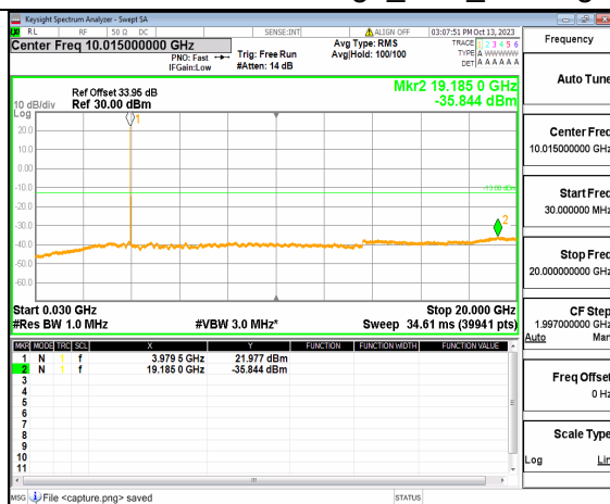
5A_n77(3700-3980MHz) (30MHz-20GHz) 15M DFT-s-OFDM QPSK Edge 1RB Right High
