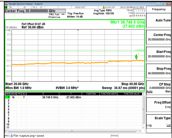
5A_n77(3700-3980MHz) (20GHz-40GHz) 20M DFT-s-OFDM BPSK Edge_1RB_Left Low
