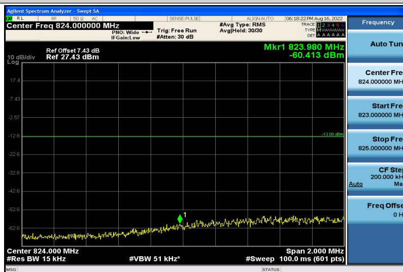
Band5-10MHz-QPSK-20450-1RB#5
