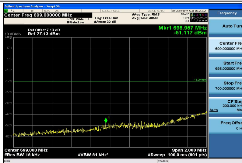
Band12-5MHz-16QAM-23035-1RB#5
