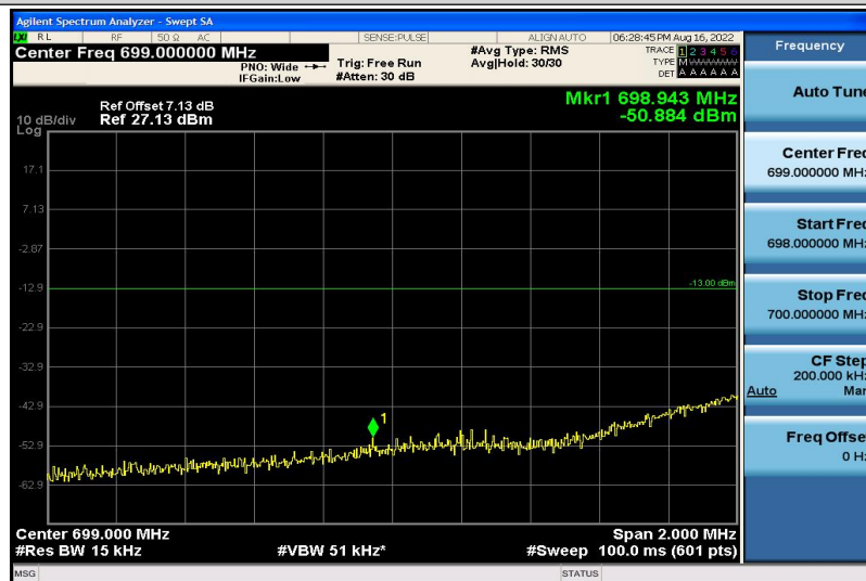
Band12-5MHz-QPSK-23035-1RB#5
