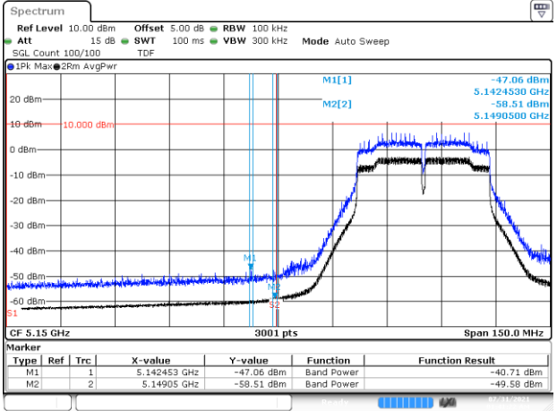
BE-R-LOW, MIMO-A, 802.11n40-HT8, Ch38
