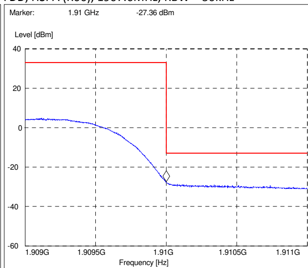
FDD, HSPA (R06), 1907.6MHz, RBW = 50kHz
