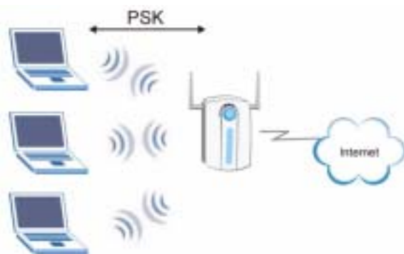
Figure 8 WPA-PSK Authentication
