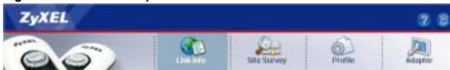
Figure 7 Menu Summary
