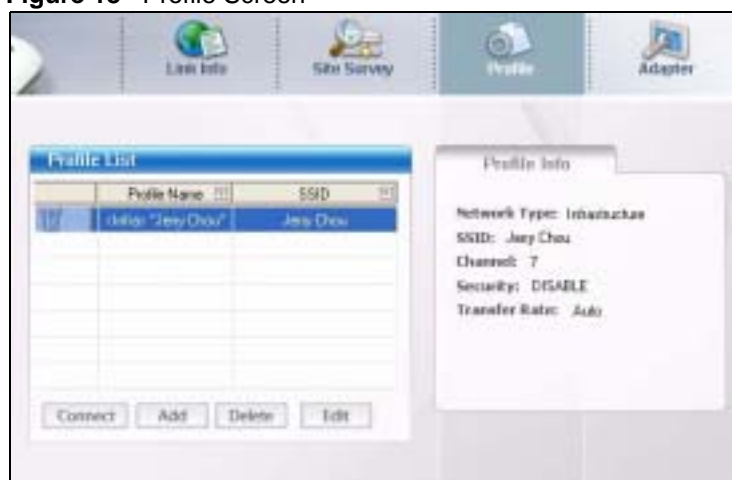
Figure 18 Profile Screen
