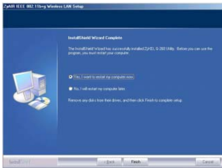
Figure 28 Uninstall: Finish
