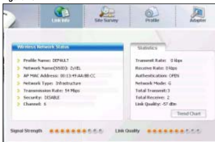
Figure 10 Link Info
