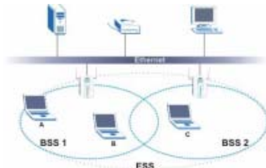
Figure 1 Application: Infrastructure
