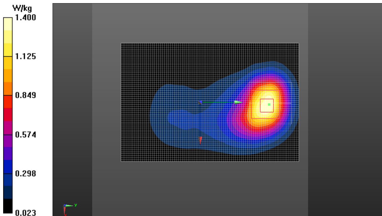
Fig.2 LTE Band 4
