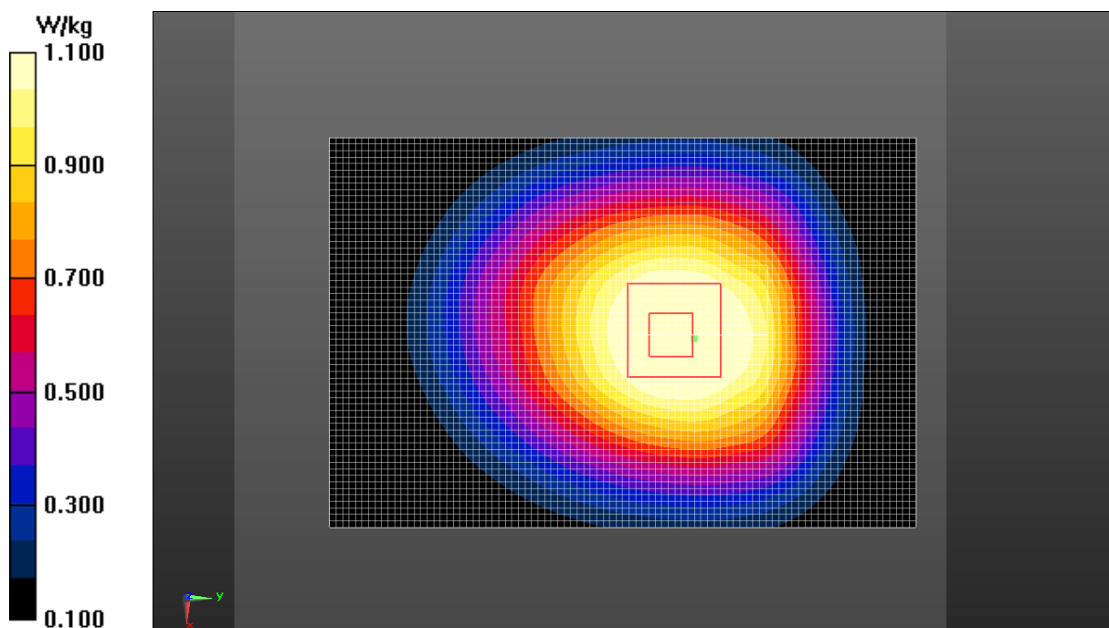
Fig.3 LTE Band 5
