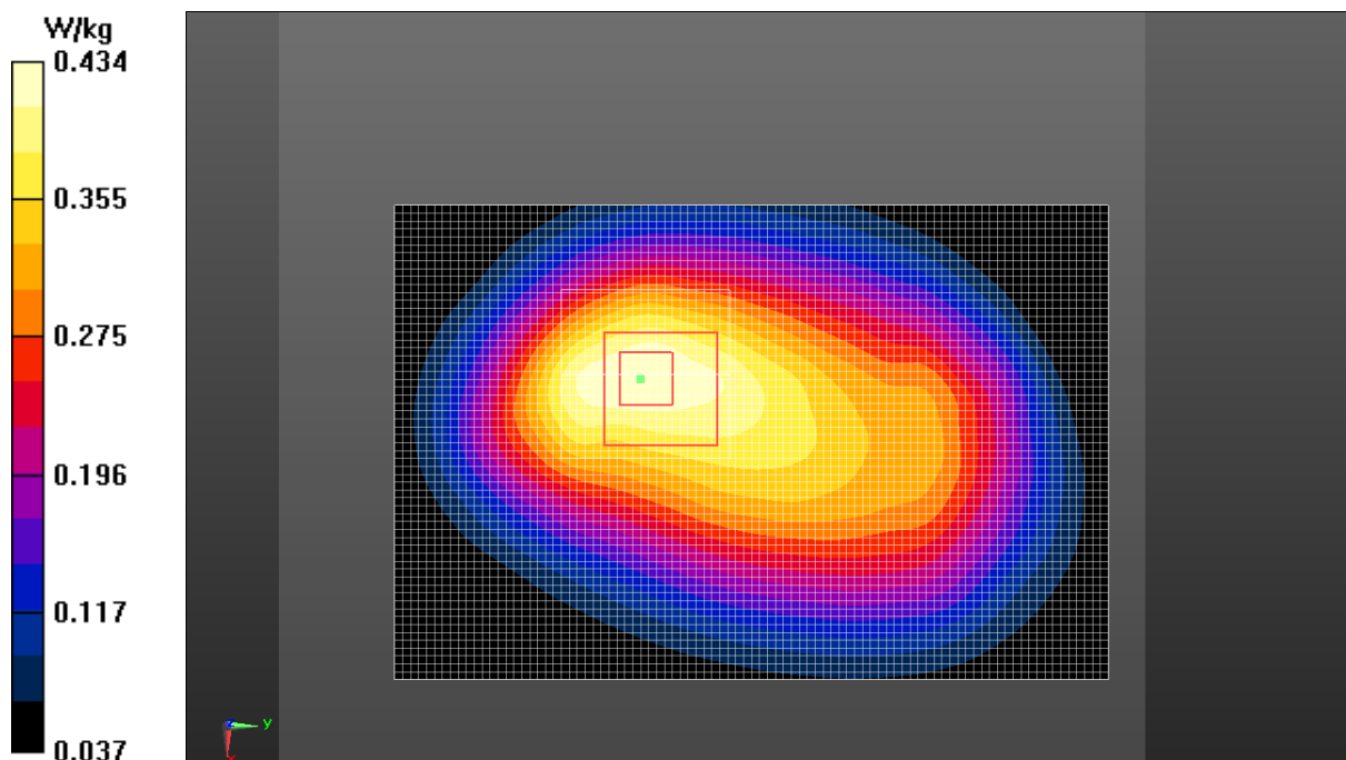
Fig.5 LTE Band 13
