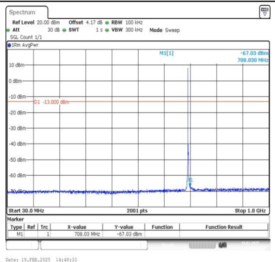
Band12_3MHz_16QAM_23025_1RB#0_30~1000_ 30~1000
