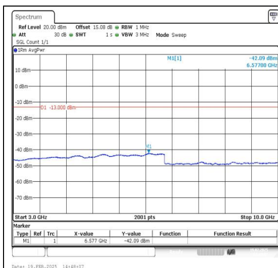
Band12_3MHz_QPSK_23025_1RB#0_3000~100 00_3000~10000
