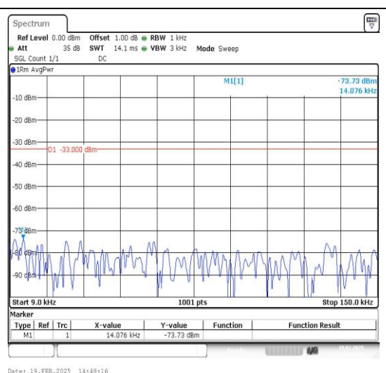
Band12_3MHz_16QAM_23025_1RB#0_0.009~0.1 5_0.009~0.15
