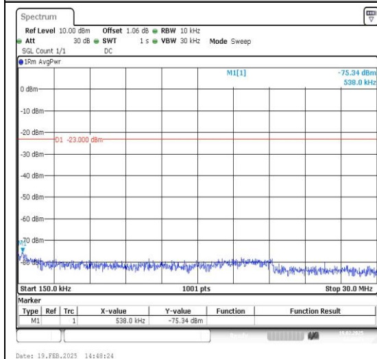
Band12_3MHz_16QAM_23025_1RB#0_0.15~30 _0.15~30
