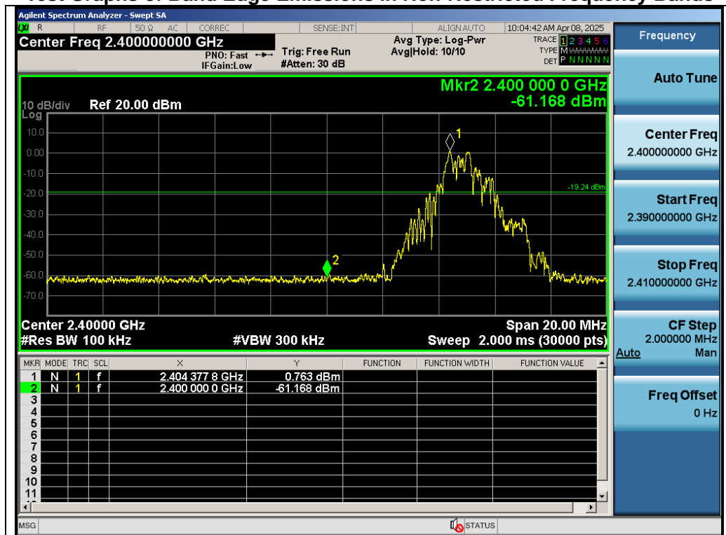
Test_Graph_SRD 2.4G_2405_Lower Band Edge Emissions
