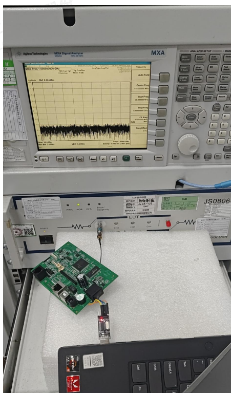
Conducted Measurement
