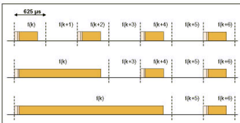
Figure 2.2: Multi-slot packets
