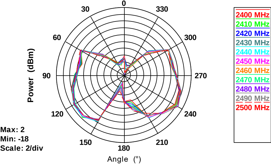
WBZ451HPA with Ground plane 2D_XZ-Cut
