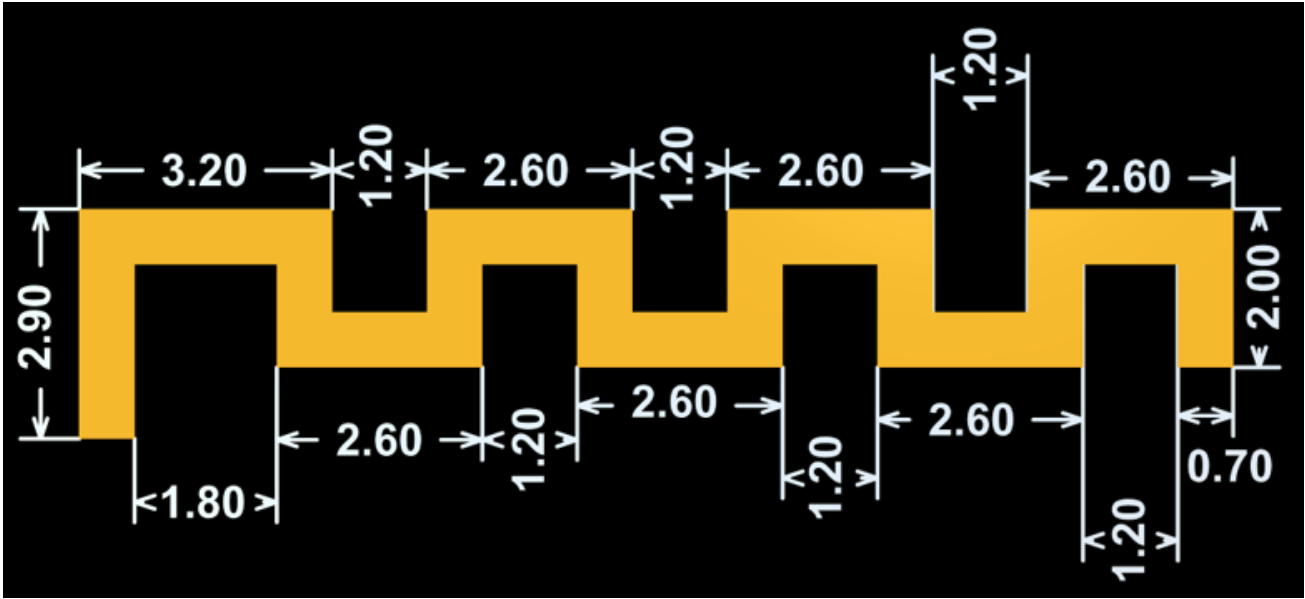
Antenna view
