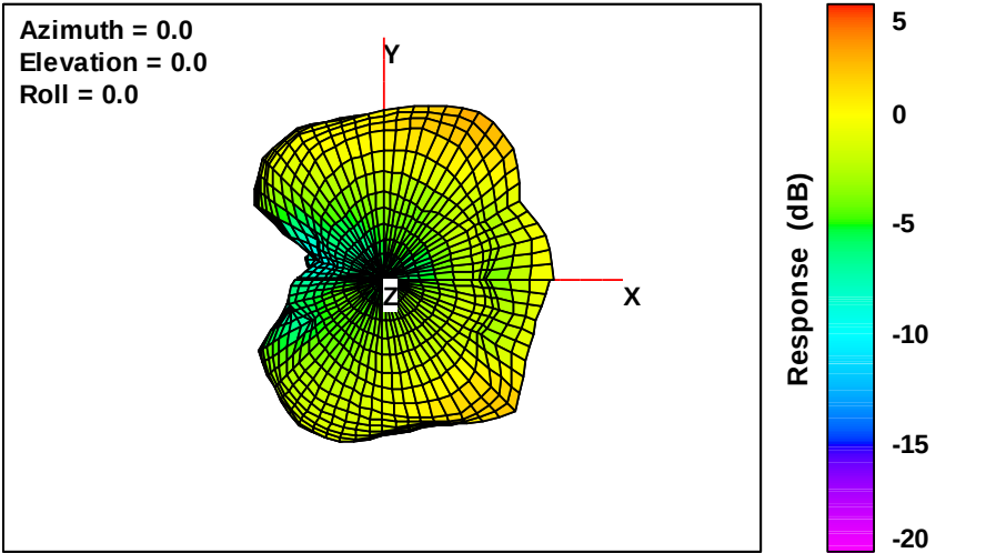
WBZ451HPA with Ground plane 2D_XY-Cut
