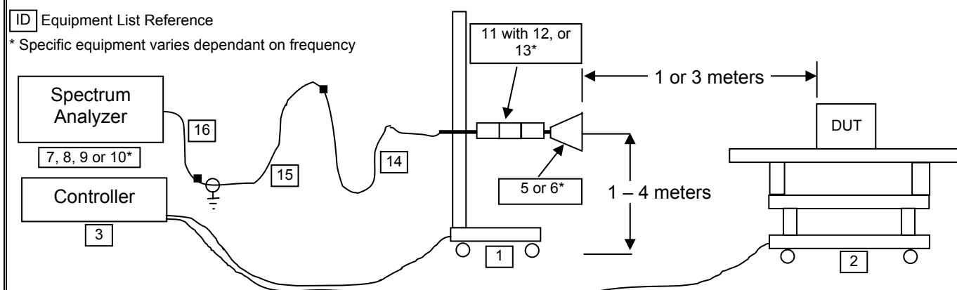
Figure H.6-1 - Setup Drawing
