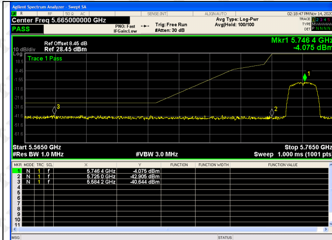
802.11n(HT40)-5755
