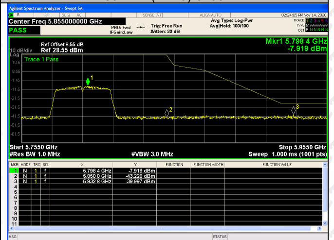
802.11n(HT40)-5795
