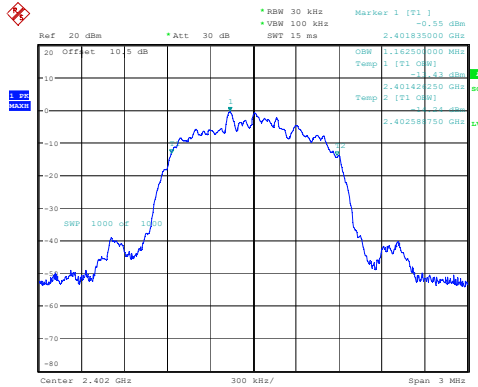
3DH1_Low 1.163MHz
