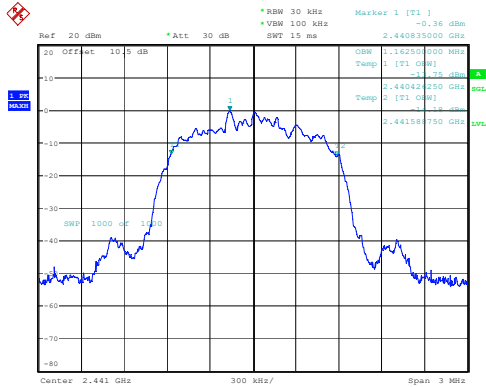
3DH1_Middle 1.163MHz
