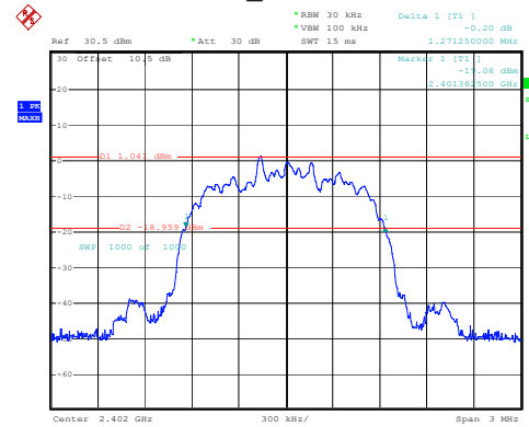
2DH1_Low 1.271MHz
