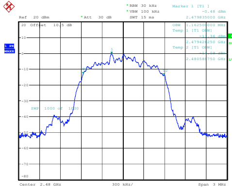
3DH1_High 1.163MHz
