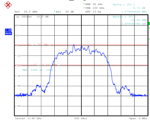
2DH1_High 1.275MHz
