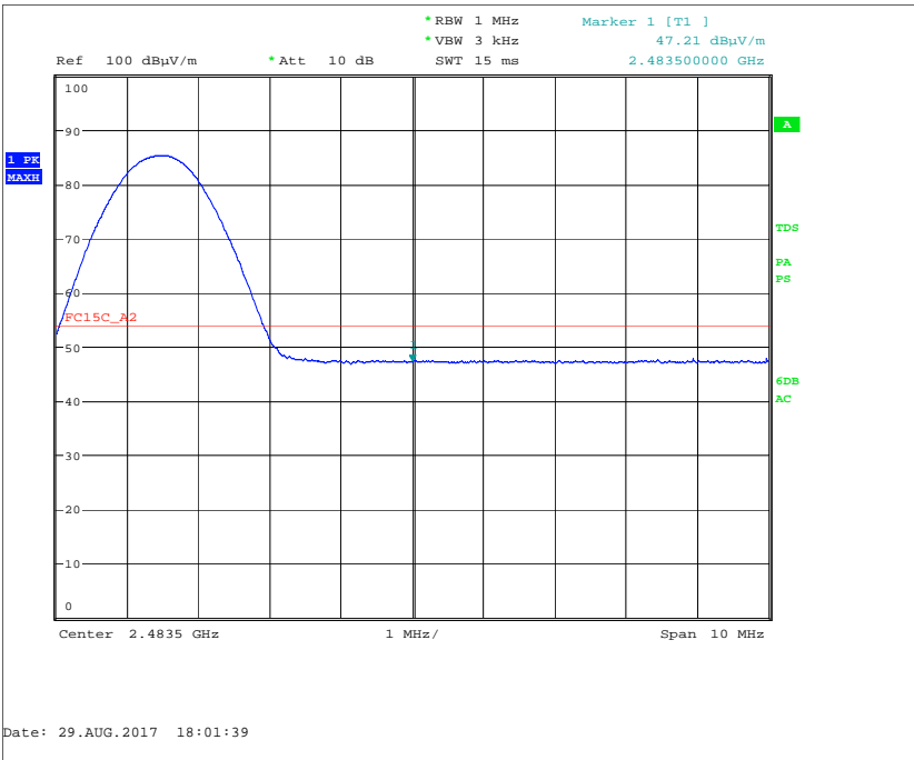
Figure 22 - GFSK - 2480 MHz - Measured Frequency 2483.5 MHz, Average
