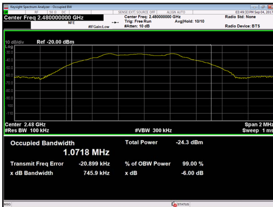
Figure 3 - 2480 MHz
