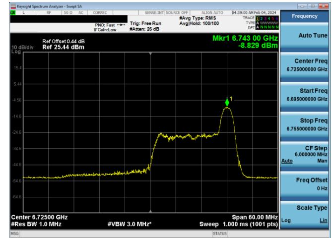
Plot 7-813. LPI Power Spectral Density Plot SDM Diversity Antenna WF8 (40MHz 802.11ax RU26 (UNII Band 7) – Ch. 155)
