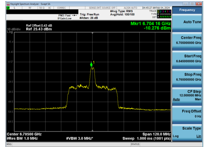
Plot 7-819. LPI Power Spectral Density Plot SDM Diversity Antenna WF8 (80MHz 802.11ax RU26 (UNII Band 7) – Ch. 151)
