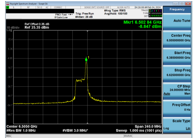
Plot 7-795. LPI Power Spectral Density Plot SDM Diversity Antenna WF8 (160MHz 802.11ax RU26 (UNII Band 6) – Ch. 111)
