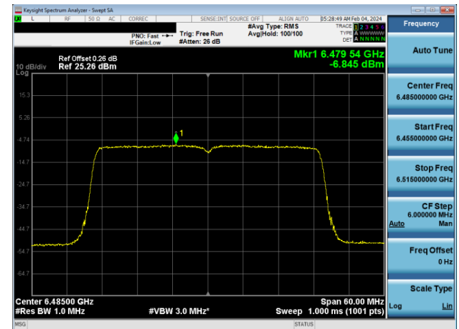
Plot 7-783. LPI Power Spectral Density Plot SDM Diversity Antenna WF8 (40MHz 802.11ax RU484 (UNII Band 6) – Ch. 107)
