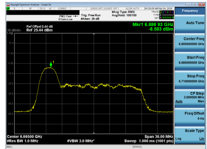
Plot 7-801. LPI Power Spectral Density Plot SDM Diversity Antenna WF8 (20MHz 802.11ax RU26 (UNII Band 7) – Ch. 149)
