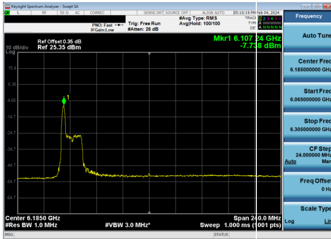
Plot 7-762. LPI Power Spectral Density Plot SDM Diversity Antenna WF7 (160MHz 802.11ax RU26 (UNII Band 5) – Ch. 47)
