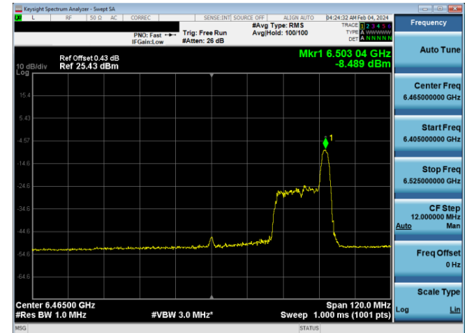
Plot 7-789. LPI Power Spectral Density Plot SDM Diversity Antenna WF8 (80MHz 802.11ax RU26 (UNII Band 6) – Ch. 103)
