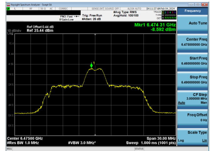
Plot 7-771. LPI Power Spectral Density Plot SDM Diversity Antenna WF8 (20MHz 802.11ax RU26 (UNII Band 6) – Ch. 105)
