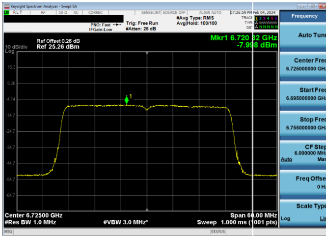
Plot 7-816. LPI Power Spectral Density Plot SDM Diversity Antenna WF7 (40MHz 802.11ax RU484 (UNII Band 7) – Ch. 155)
