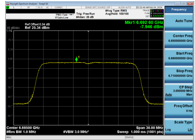
Plot 7-807. LPI Power Spectral Density Plot SDM Diversity Antenna WF8 (20MHz 802.11ax RU242 (UNII Band 7) – Ch. 149)
