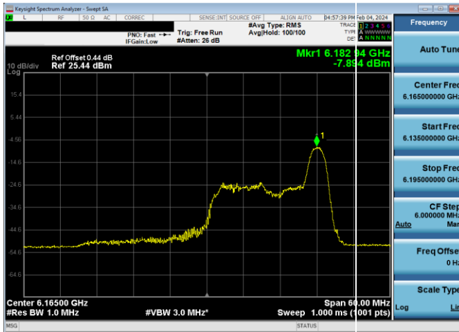
Plot 7-750. LPI Power Spectral Density Plot SDM Diversity Antenna WF7 (40MHz 802.11ax RU26 (UNII Band 5) - Ch. 43)
