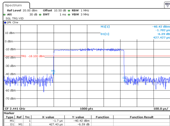
2DH1_Hopping 0.427ms
