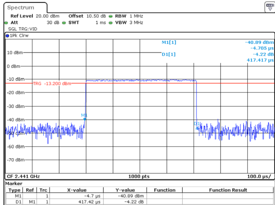
DH1_Hopping 0.417ms
