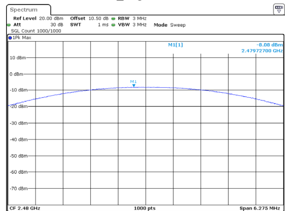
2DH1_High -8.08dBm
