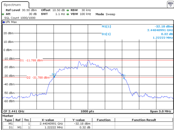
3DH1_Middle 1.222MHz
