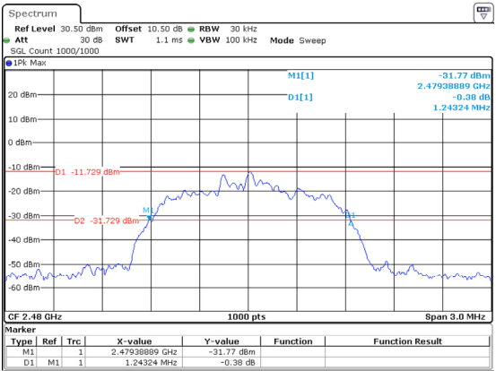
3DH1_High 1.243MHz
