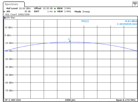
2DH1_Low -8.64dBm
