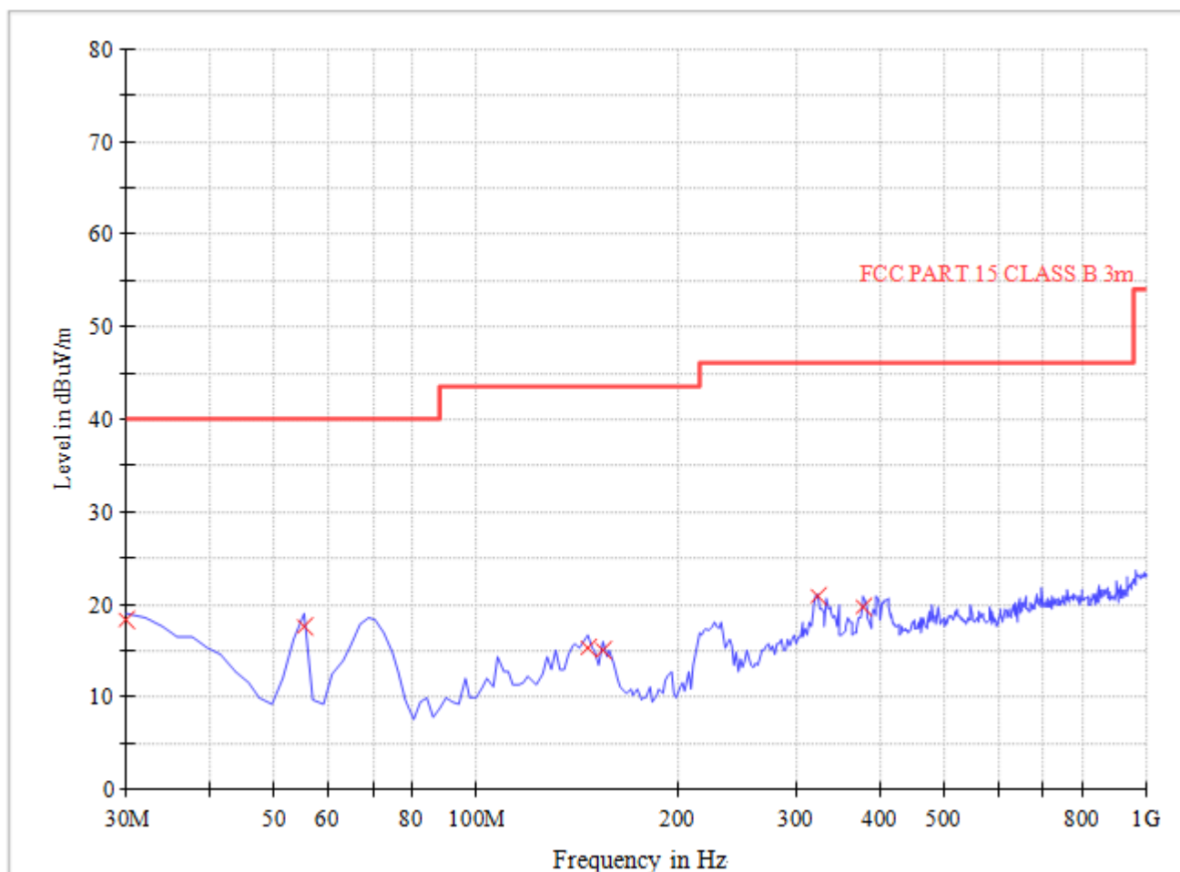
(Plot C: Test Antenna Horizontal 30M - 1G)
