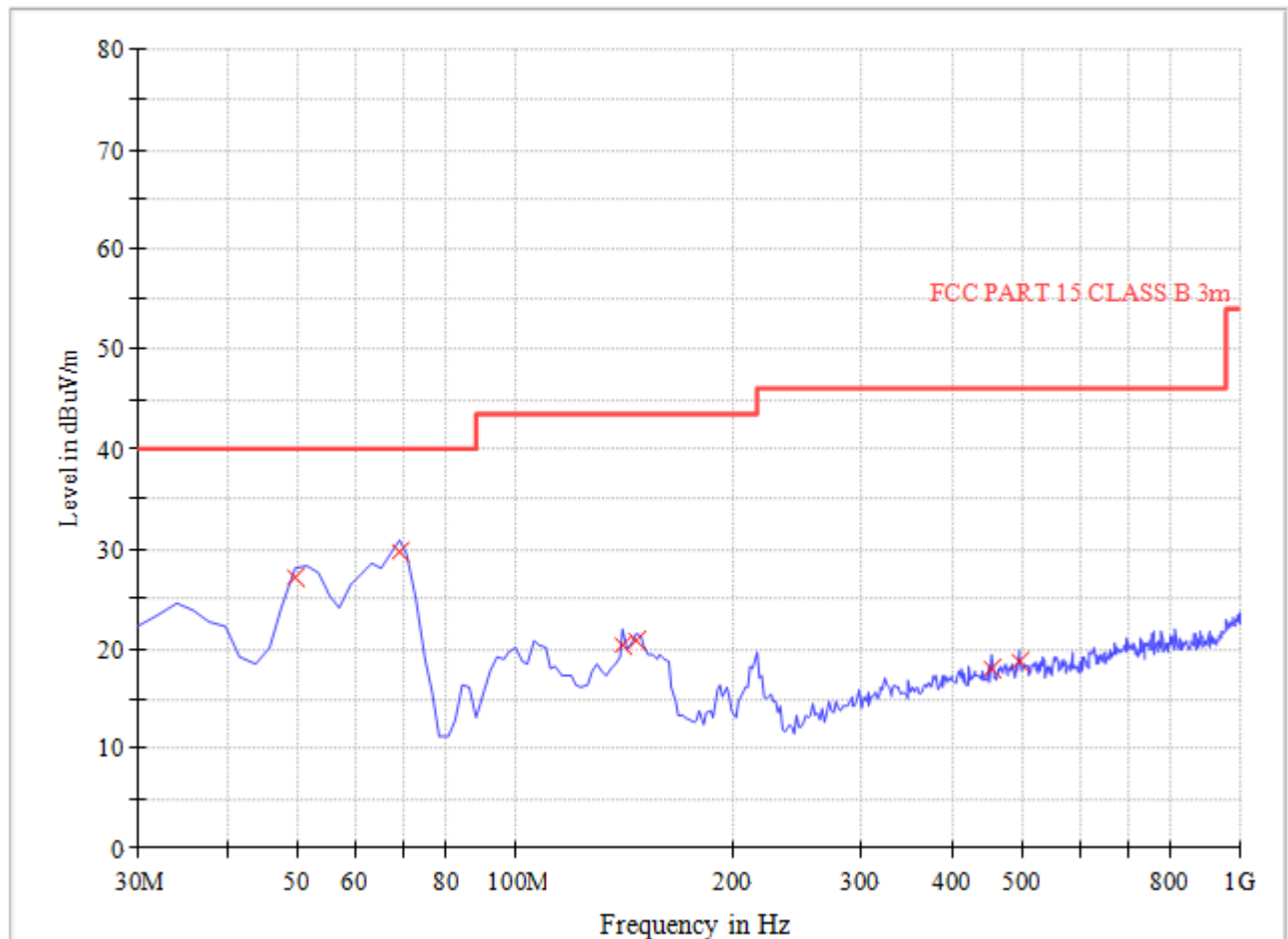
(Plot D: Test Antenna Vertical 30M - 1G)
