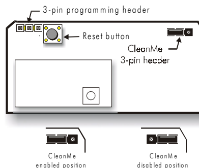
Figure B: Transmitter Board Features
