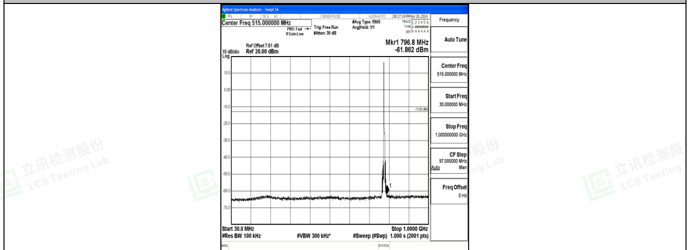
Band13_5MHz_QPSK_23230_1RB#0_30~1000_30~1000
