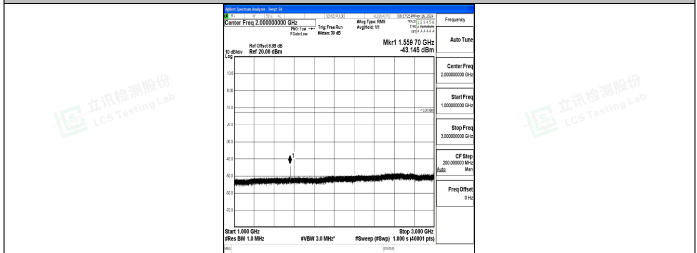
Band13_5MHz_QPSK_23230_1RB#0_1000~3000_1000~3000
