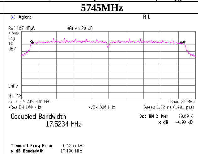
11n-20, Antenna port 2, MCS 0(Long)
