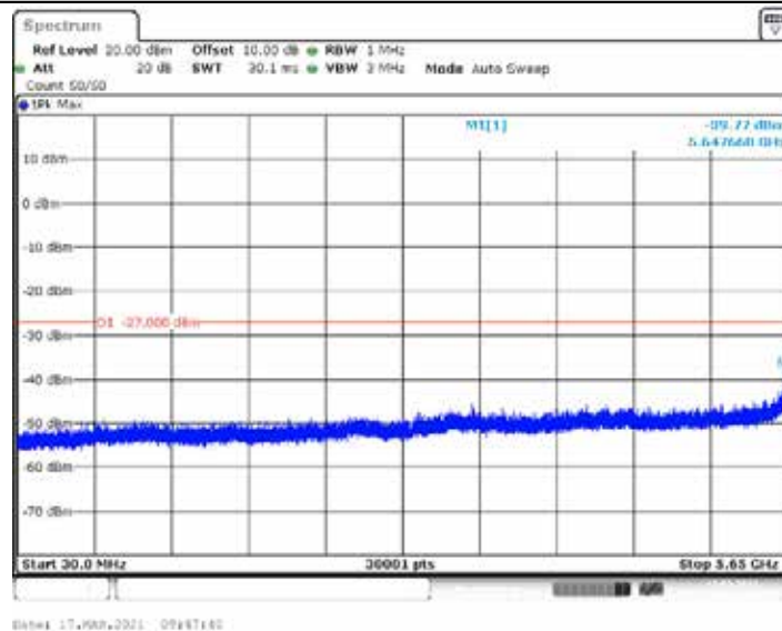
11AC80SISO_Ant2_5775_30~5650
