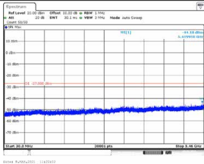
11A_Ant2_5700_30~5460
