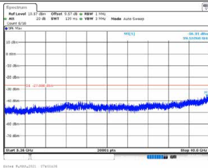
11AX20SISO_Ant1_5260_5360~40000
