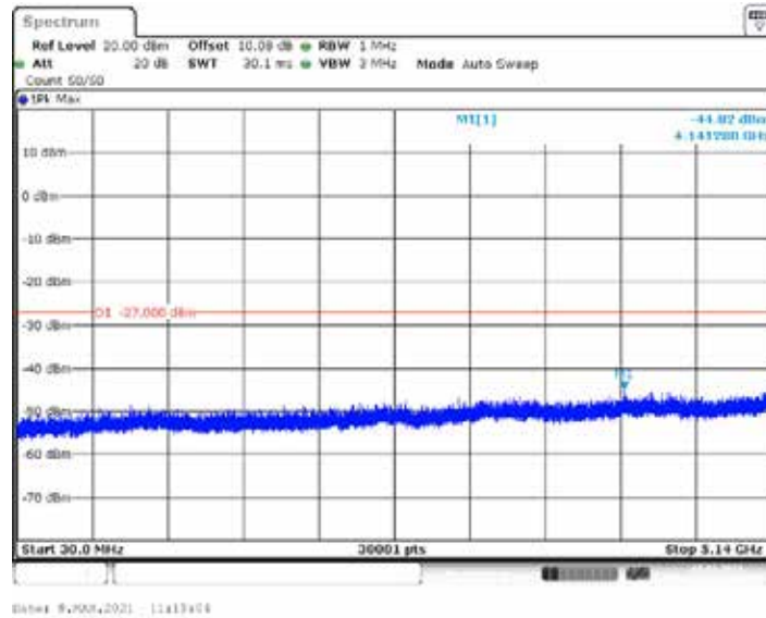
11A_Ant2_5320_5360~40000
