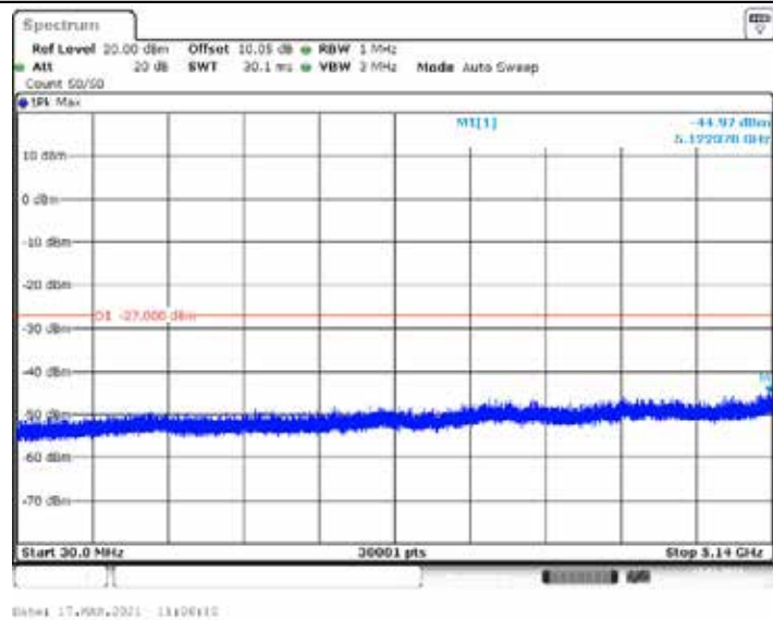
11AX40SISO_Ant2_5270_30~5140
