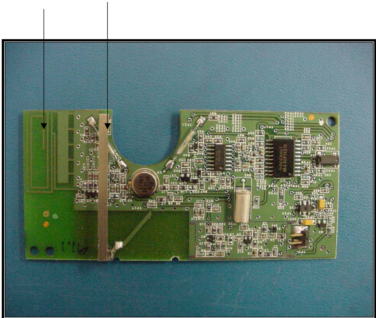
PHOTOGRAPH 1: ANTENNA LOCATION
