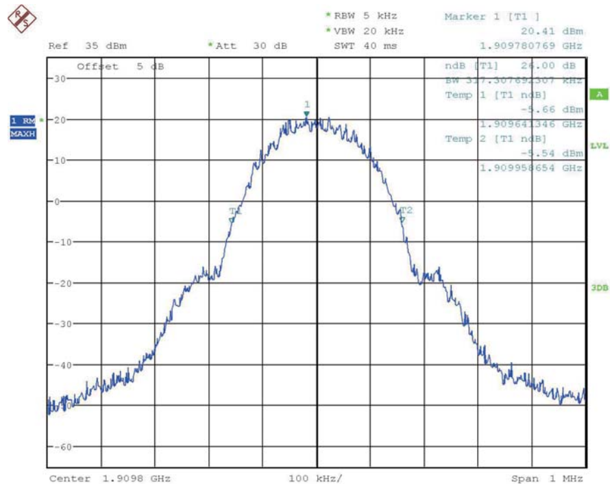
99% OBW-8PSK-Channel 810
