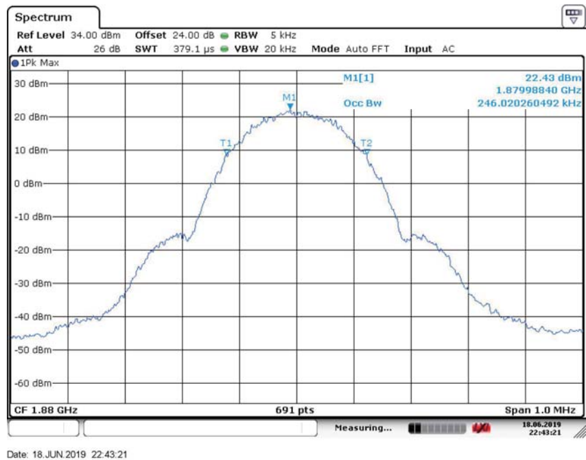
99% OBW-GMSK-Channel 661
