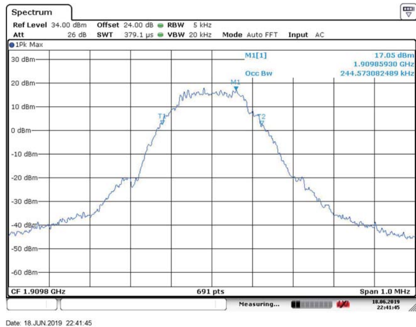
99% OBW-8PSK-Channel 810
