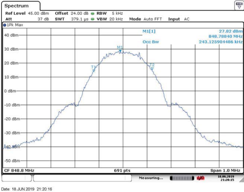
99% OBW-GMSK-Channel 251
