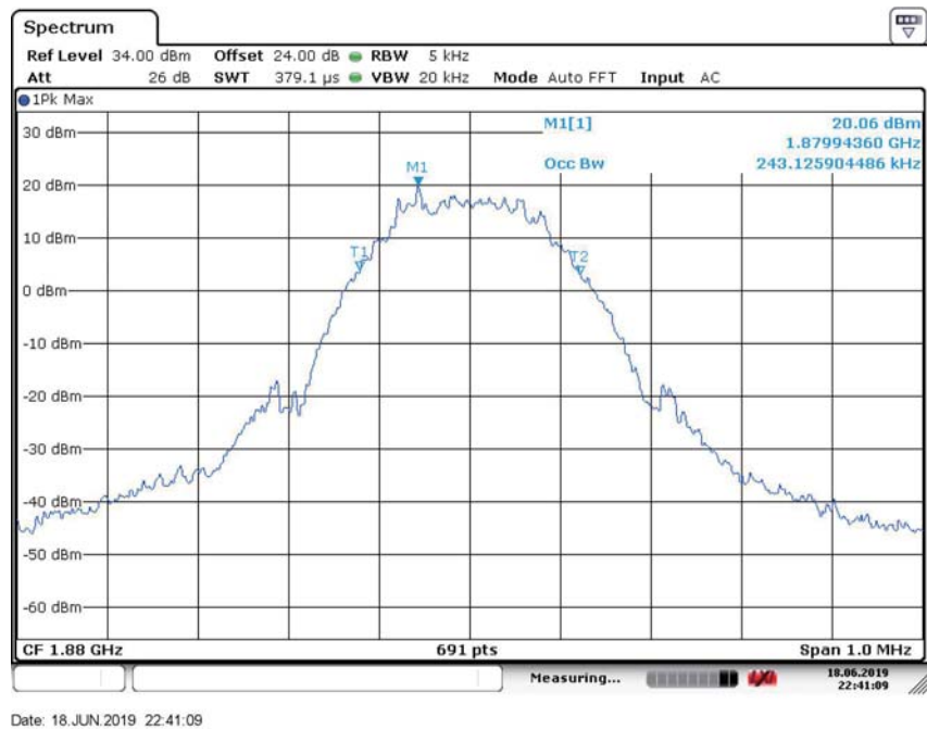
99% OBW-8PSK-Channel 661
