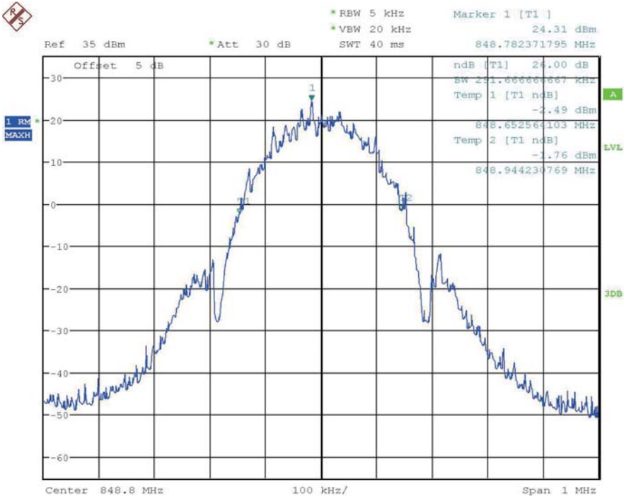
99% OBW-8PSK-Channel 251
