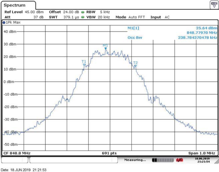
99% OBW-8PSK-Channel 251
