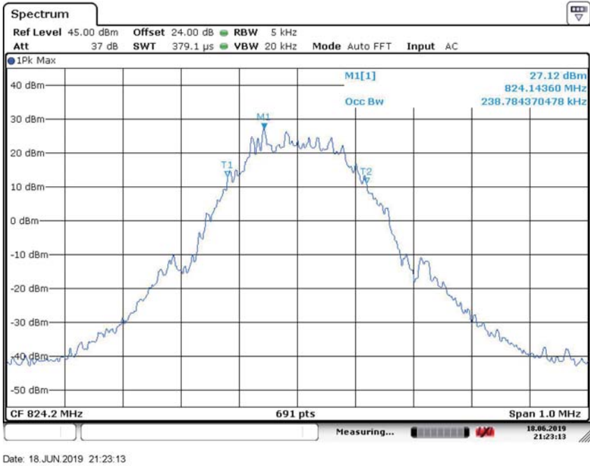
99% OBW-8PSK-Channel 128
