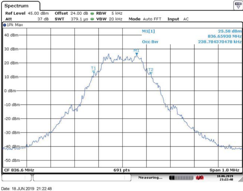
99% OBW-8PSK-Channel 190
