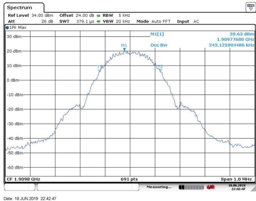
99% OBW-GMSK-Channel 810
