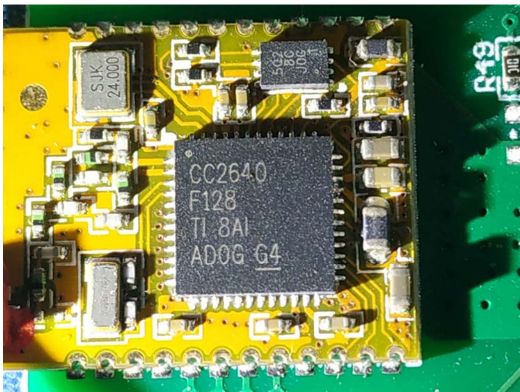
2.4G SRD Receiver module front
