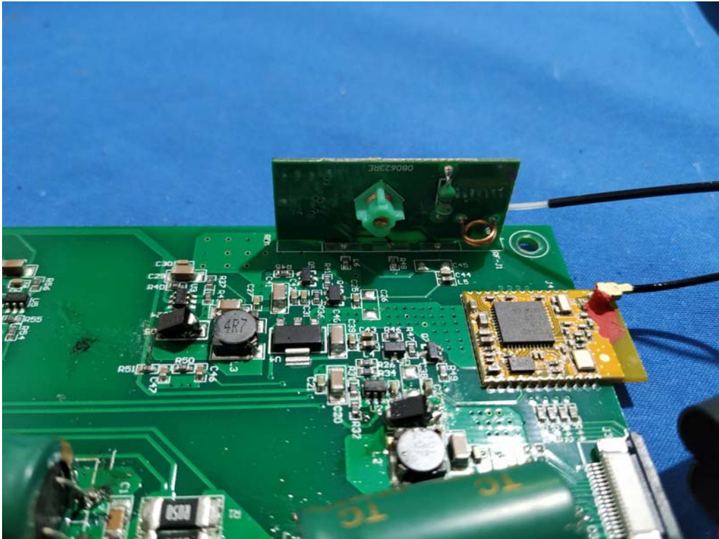
2.4G SRD Receiver Module bottom
