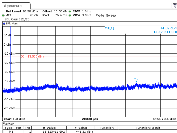
1.4MHz_Low_QPSK_6@0(1GHz~20.1GHz)
