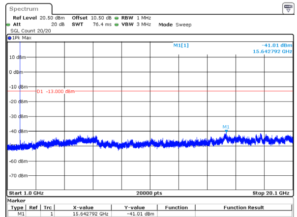
1.4MHz_Low_QPSK_1@0(1GHz~20.1GHz)
