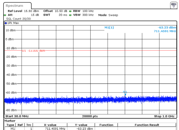
1.4MHz_Low_QPSK_6@0(30MHz~1GHz)
