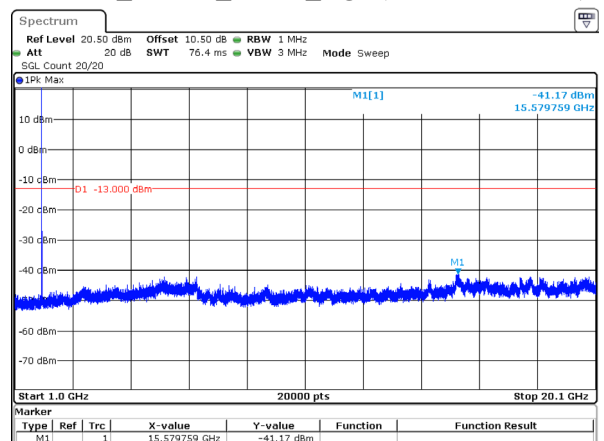
1.4MHz_Middle_QPSK_1@0(1GHz~20.1GHz)
