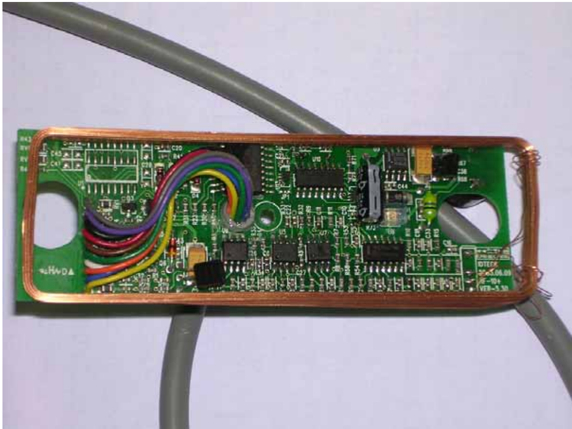
PCB ASS'Y_Top
