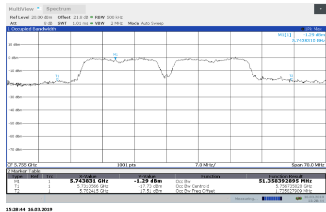
Figure 8.7-2: 99 % bandwidth on 802.11n, sample plot
