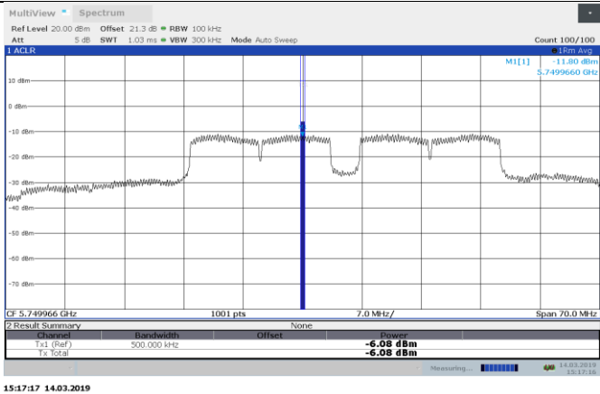
Figure 8.8-4: Sample plot for PPSD on 802.11n
