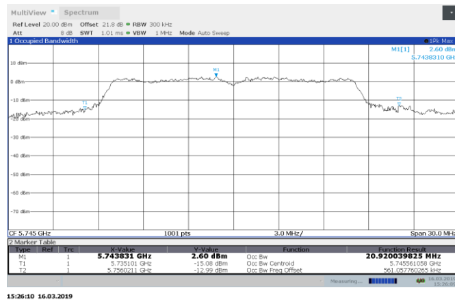
Figure 8.7-1: 99 % bandwidth on 802.11a, sample plot
