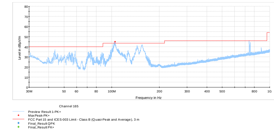
Figure 8.9-3: Radiated spurious emissions 30 MHz – 1 GHz high channel, 802.11a
