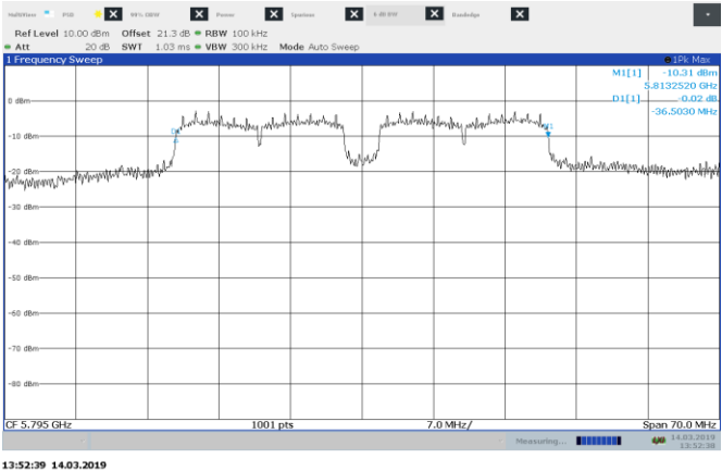
Figure 8.5-2: 6 dB bandwidth on 802.11n, sample plot
