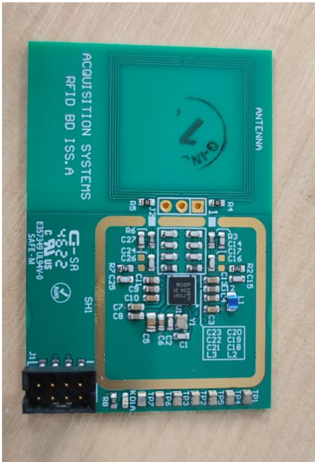
Figure 9: RFID PCB top
