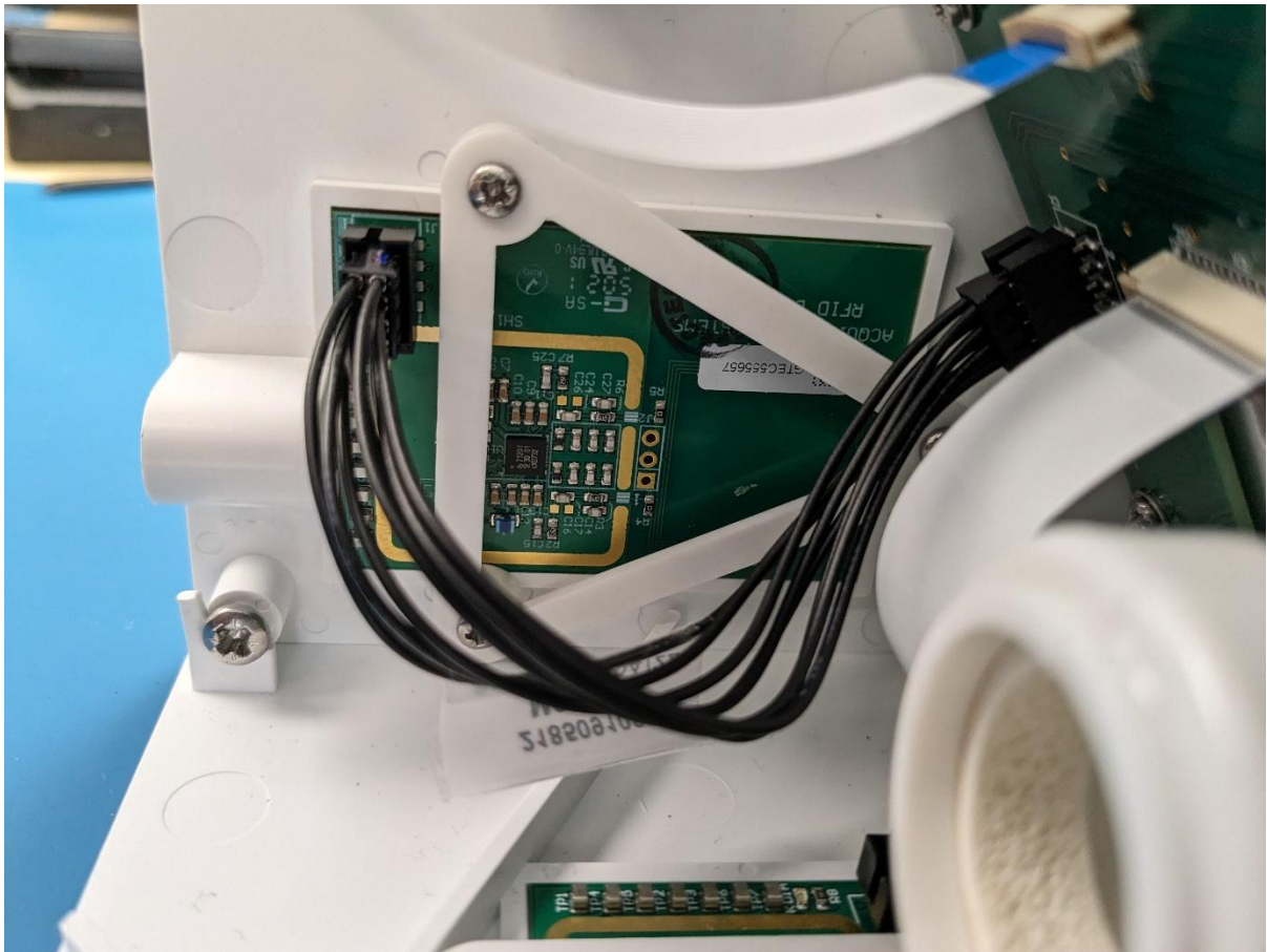
Figure 4: Side RFID PCB
