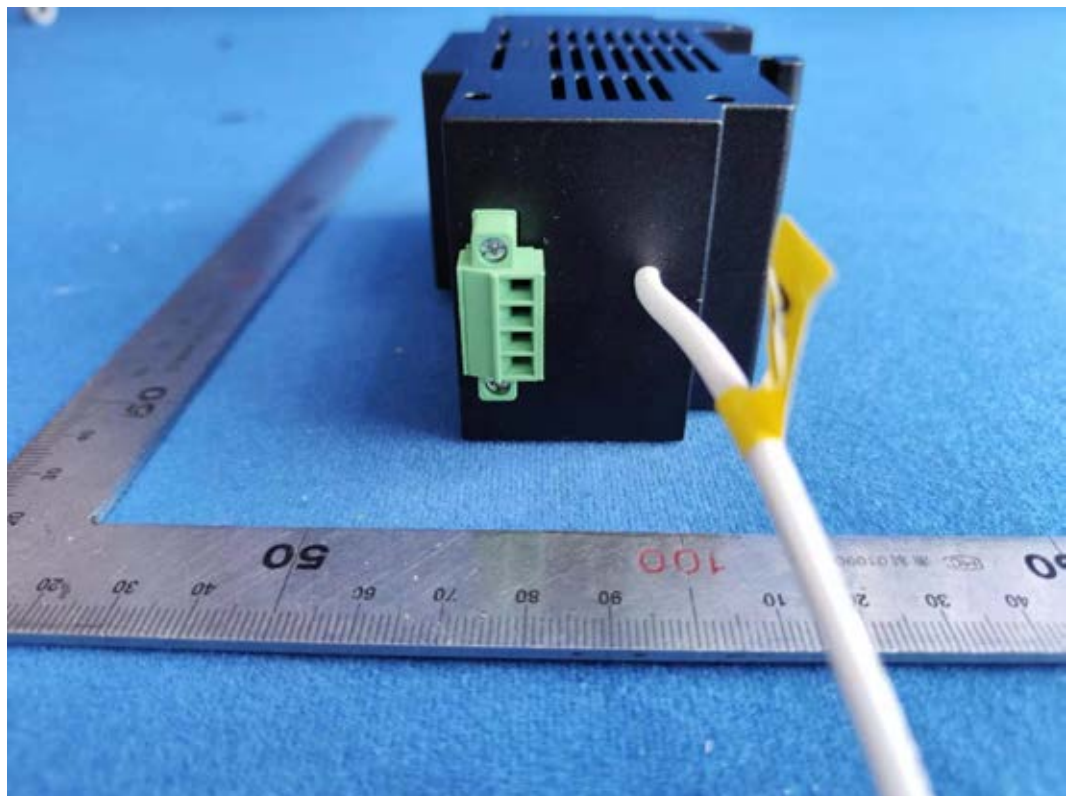
FIGURE 6 1-INCH 2-CHANNEL POWER MONITOR MODULE, PIGTAIL (M/N: GPM-H2SEM-00) GENERAL APPEARANCE RIGHT VIEW
