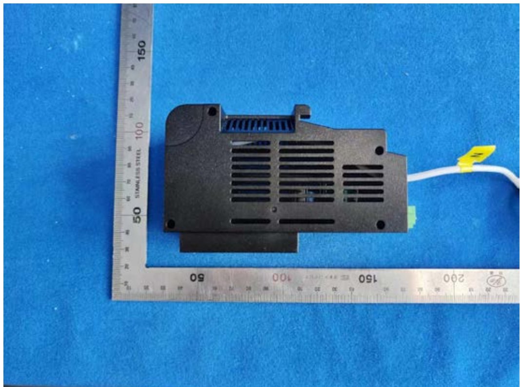
FIGURE 2 1-INCH 2-CHANNEL POWER MONITOR MODULE, PIGTAIL (M/N: GPM-H2SEM-00) GENERAL APPEARANCE TOP VIEW
