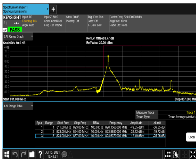
Band5-10MHz-QPSK-20450-50RB#0
