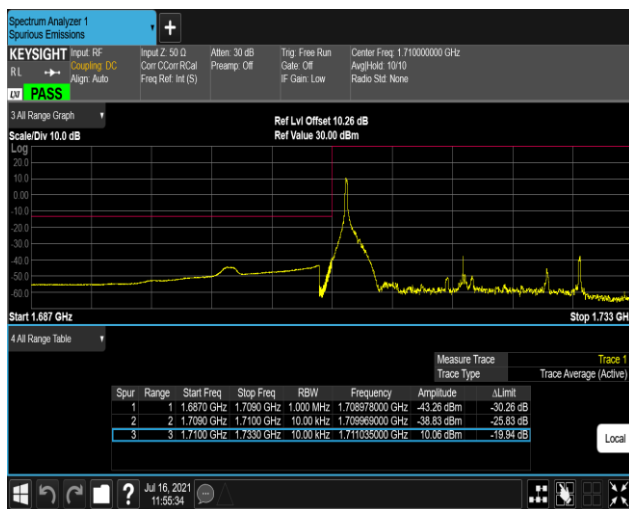
Band4-20MHz-16QAM-20050-100RB#0
