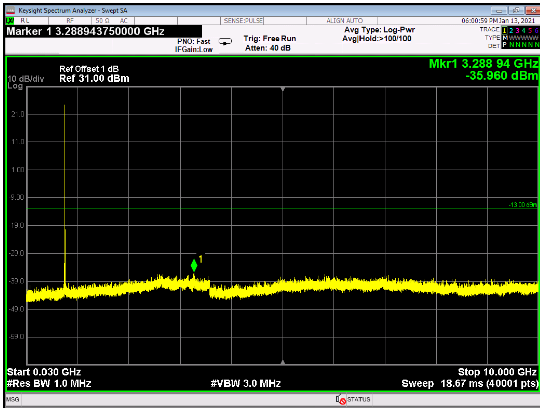
Band13 QAM16 BW=1.4MHz Channel=23205 RB Size=1 Position=#0
