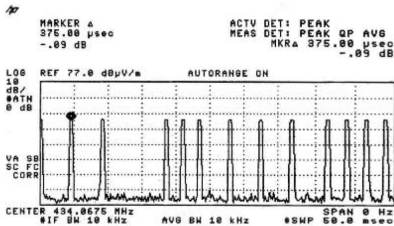
Figure C [Short Pulse]
