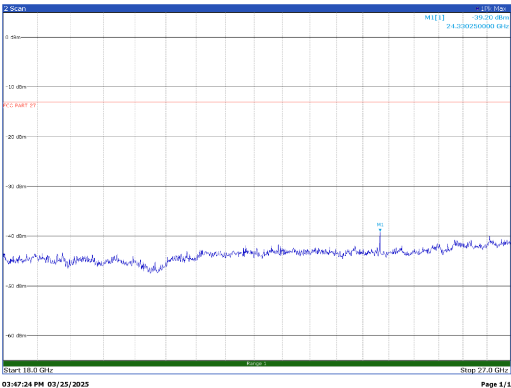
100 MHz signal, middle channel, 18GHz – 27GHz – V Pol
