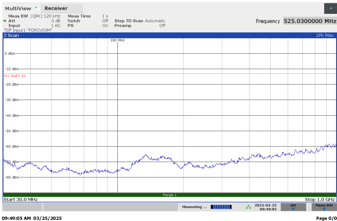
100 MHz signal, top channel, 30MHz – 1GHz – V Pol
