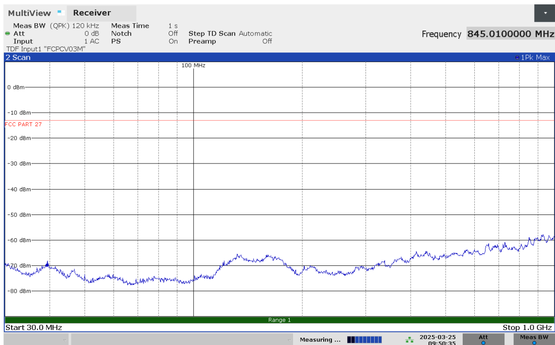
100 MHz signal, top channel, 30MHz – 1GHz – H Pol
