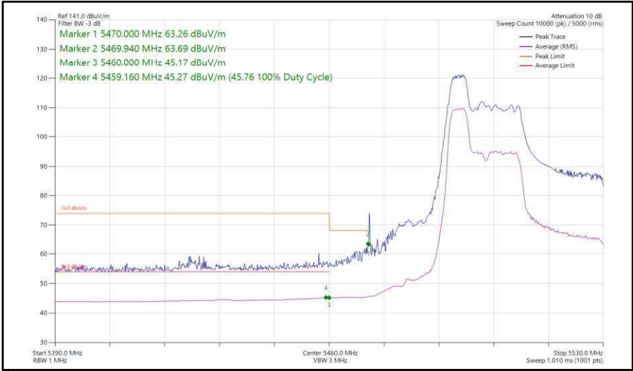
Figure 378 - 802.11ax, HE40, RU 52-37, SISO, Core 1 - 5510 MHz, Band Edge Frequency 5470 MHz
