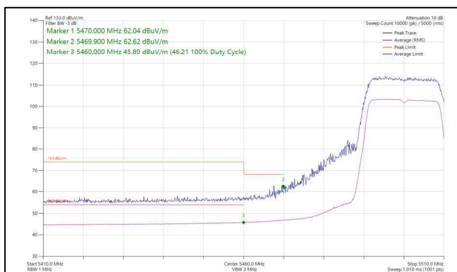
Figure 351 - 802.11ac, VHT20, TxBF, Core 0-1 - 5500 MHz, Band Edge Frequency 5470 MHz
