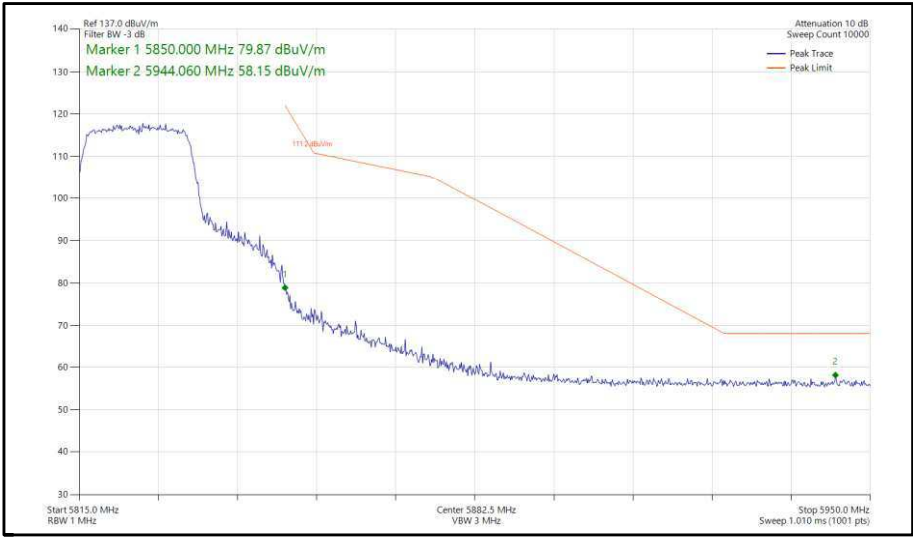
Figure 358 - 802.11ac, VHT20, TxBF, Core 0-1 - 5825 MHz, Band Edge Frequency 5850 MHz
