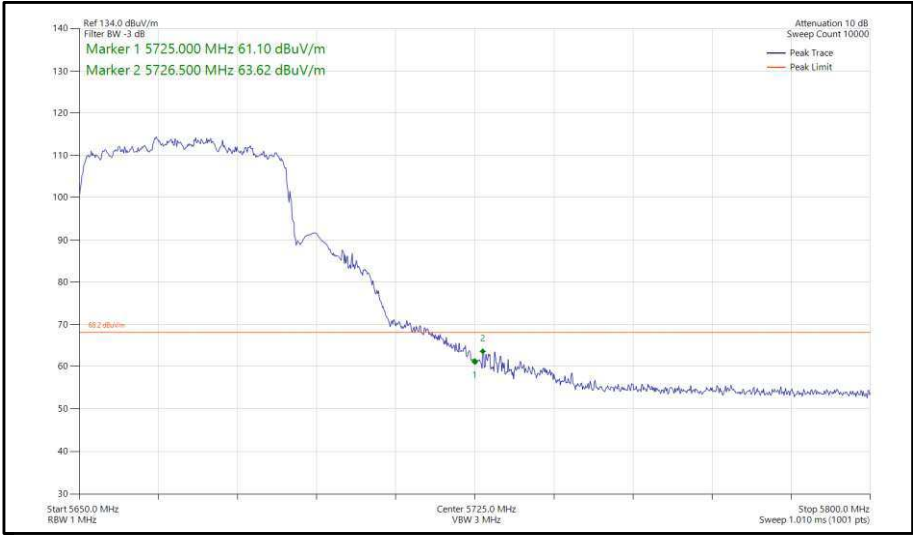
Figure 399 - 802.11ax, HE40, SU, CDD, Core 0-1 - 5670 MHz, Band Edge Frequency 5725 MHz
