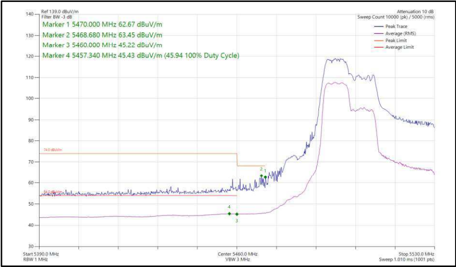
Figure 393 - 802.11ax, HE40, RU 106-53, CDD, Core 0-1 - 5510 MHz, Band Edge Frequency 5470 MHz
