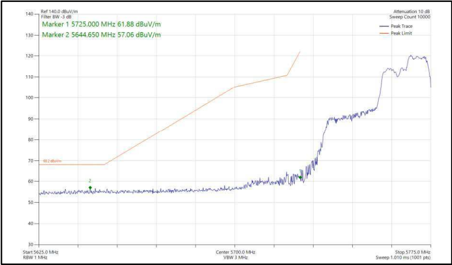
Figure 397 - 802.11ax, HE40, RU 106-56, CDD, Core 0-1 - 5755 MHz, Band Edge Frequency 5725 MHz
