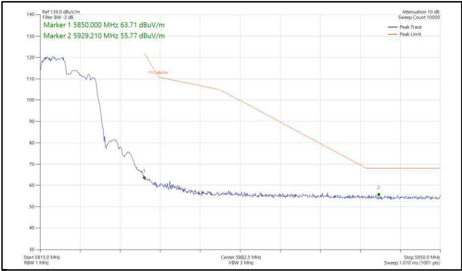
Figure 350 - 802.11ax, HE20, RU 106-53, SDM, Core 0-1 - 5825 MHz, Band Edge Frequency 5850 MHz
