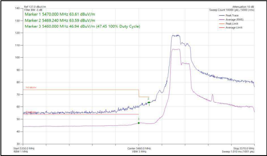
Figure 451 - 802.11ax, HE80, RU 106-53, SISO, Core 1 - 5530 MHz, Band Edge Frequency 5470 MHz
