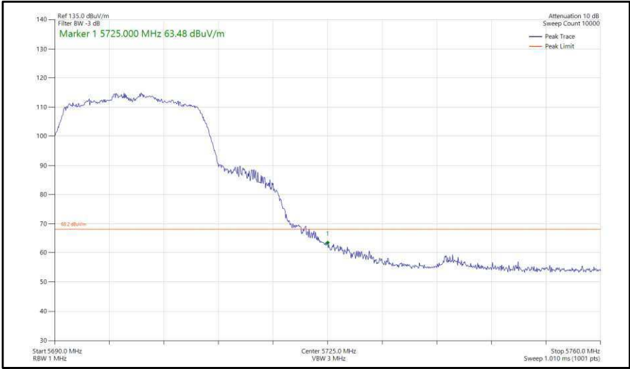
Figure 341 - 802.11n, HT20, SDM, Core 0-1 - 5700 MHz, Band Edge Frequency 5725 MHz
