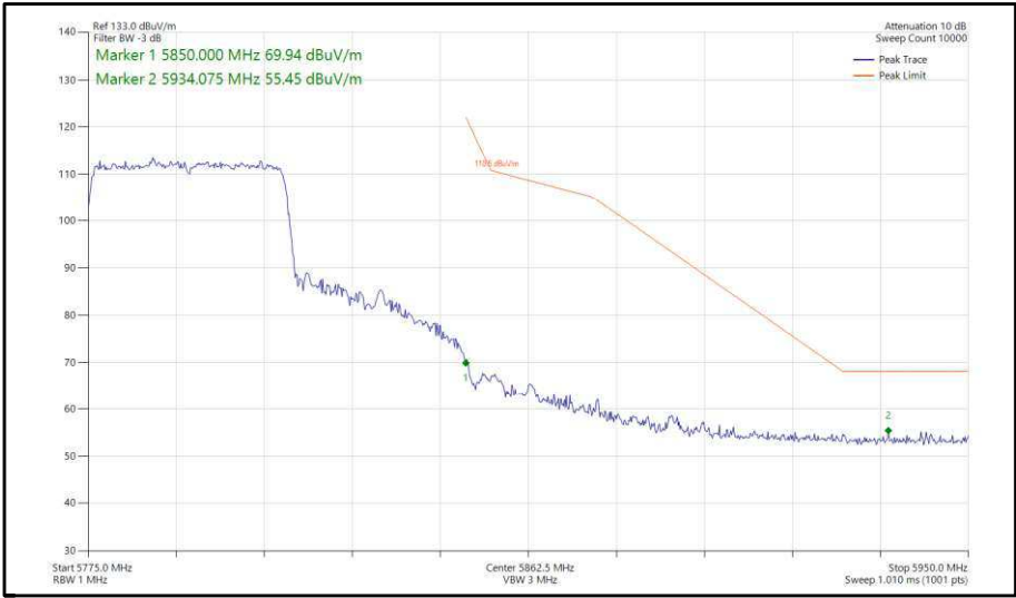
Figure 374 - 802.11ax, HE40, SU, SISO, Core 0 - 5795 MHz, Band Edge Frequency 5850 MHz
