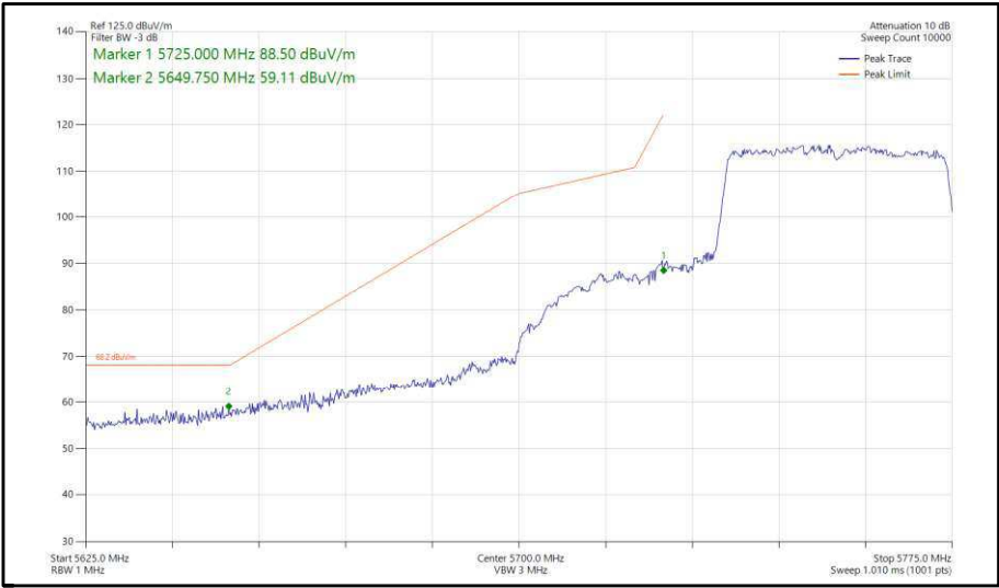
Figure 412 - 802.11ax, HE40, SU, SDM, Core 0-1 - 5755 MHz, Band Edge Frequency 5725 MHz
