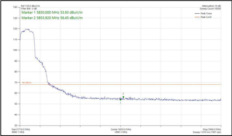
Figure 347 - 802.11ax, HE20, SU, SDM, Core 0-1 - 5720 MHz, Band Edge Frequency 5850 MHz
