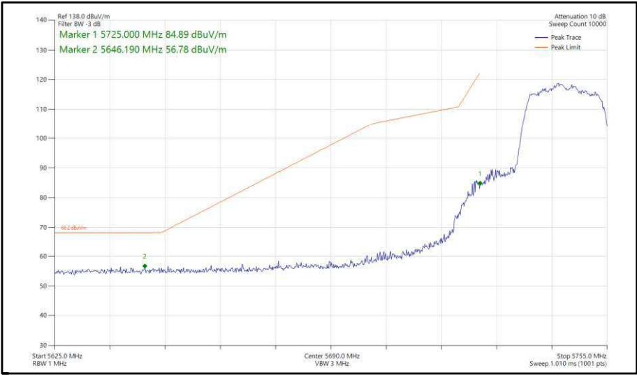
Figure 322 - 802.11n, HT20, CDD, Core 0-1 - 5745 MHz, Band Edge Frequency 5725 MHz
