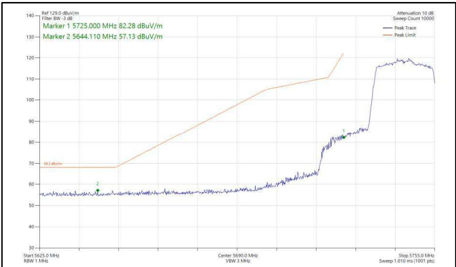
Figure 339 - 802.11ax, HE20, SU, SDM, Core 0-1 - 5745 MHz, Band Edge Frequency 5725 MHz
