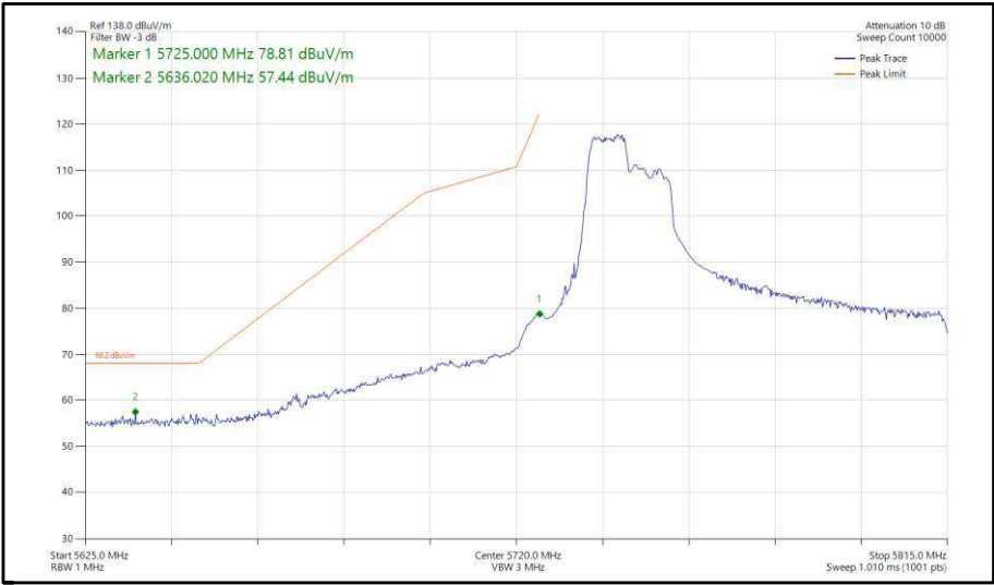
Figure 439 - 802.11ax, HE80, RU 106-53, SISO, Core 0 - 5775 MHz, Band Edge Frequency 5725 MHz
