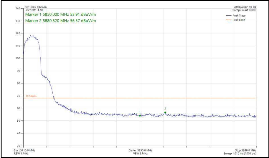
Figure 329 - 802.11n, HT20, CDD, Core 0-1 - 5720 MHz, Band Edge Frequency 5850 MHz
