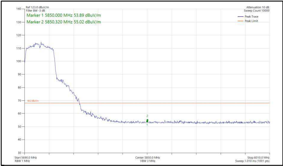
Figure 370 - 802.11n, HT40, SISO, Core 0 - 5710 MHz, Band Edge Frequency 5850 MHz
