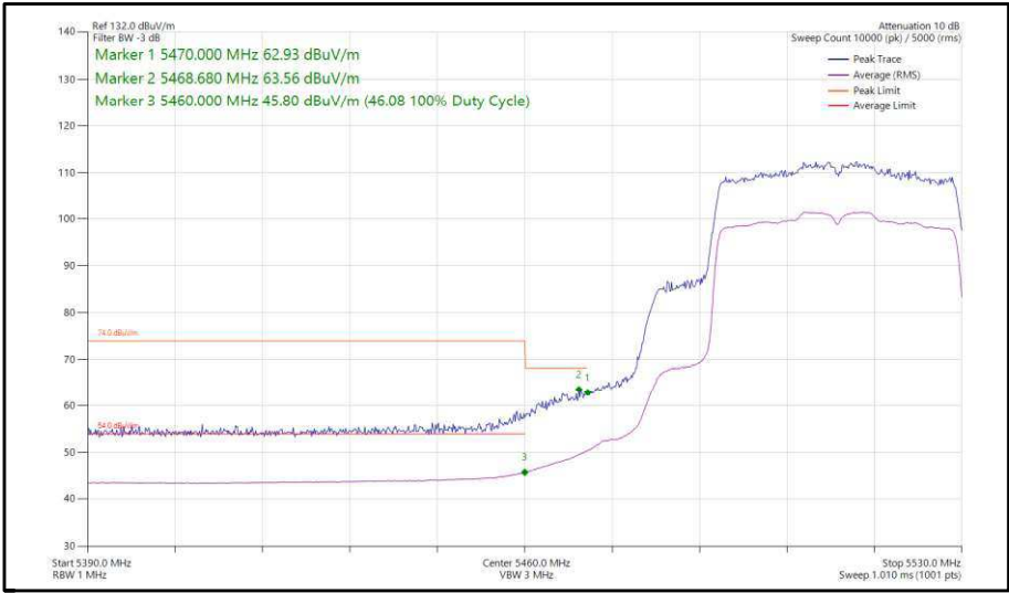
Figure 377 - 802.11ax, HE40, SU, SISO, Core 1 - 5510 MHz, Band Edge Frequency 5470 MHz
