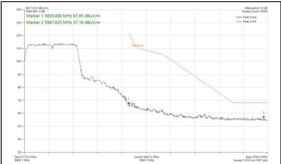
Figure 419 - 802.11n, HT40, SDM, Core 0-1 - 5795 MHz, Band Edge Frequency 5850 MHz
