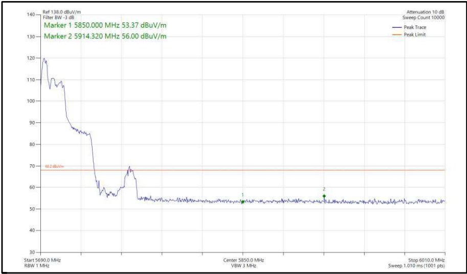
Figure 404 - 802.11ax, HE40, RU 52-37, CDD, Core 0-1 - 5710 MHz, Band Edge Frequency 5850 MHz
