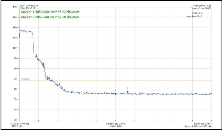
Figure 359 - 802.11ax, HE20, SU, TxBF, Core 0-1 - 5720 MHz, Band Edge Frequency 5850 MHz
