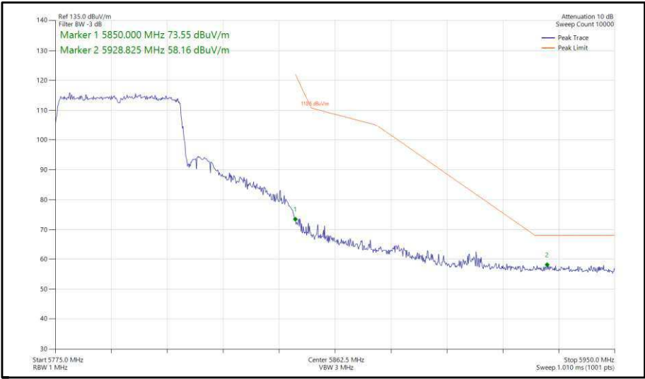
Figure 433 - 802.11ax, HE40, SU, TxBF, Core 0-1 - 5795 MHz, Band Edge Frequency 5850 MHz
