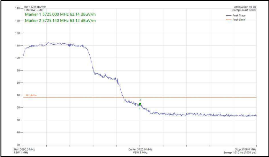
Figure 327 - 802.11ax, HE20, SU, CDD, Core 0-1 - 5700 MHz, Band Edge Frequency 5725 MHz
