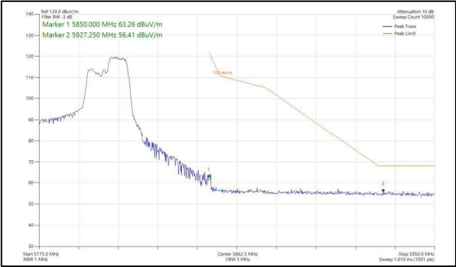
Figure 423 - 802.11ax, HE40, RU 106-56, SDM, Core 0-1 - 5795 MHz, Band Edge Frequency 5850 MHz
