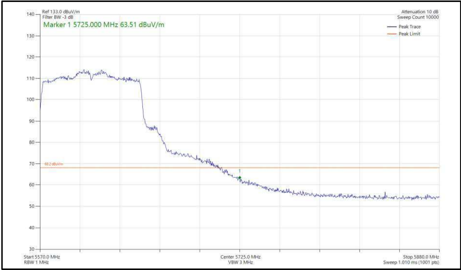
Figure 455 - 802.11ac, VHT80, SISO, Core 1 - 5610 MHz, Band Edge Frequency 5725 MHz
