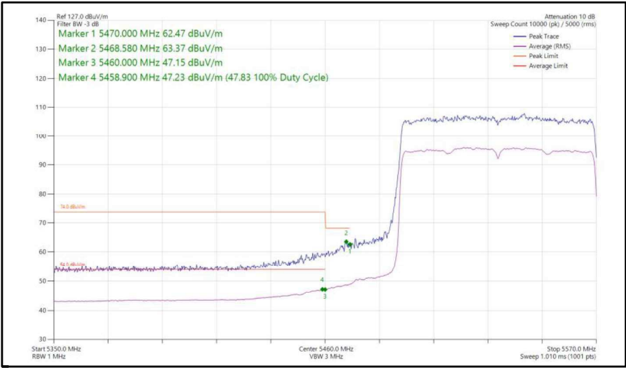
Figure 450 - 802.11ax, HE80, SU, SISO, Core 1 - 5530 MHz, Band Edge Frequency 5470 MHz
