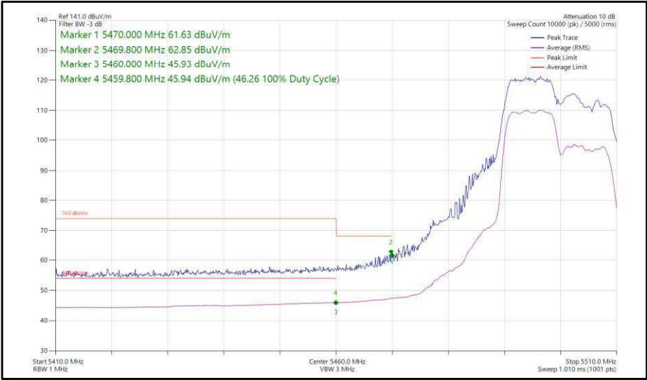
Figure 321 - 802.11ax, HE20, RU 106-53, CDD, Core 0-1 - 5500 MHz, Band Edge Frequency 5470 MHz
