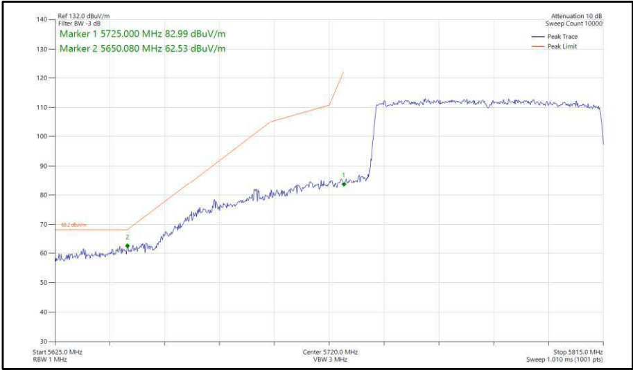
Figure 453 - 802.11ax, HE80, SU, SISO, Core 1 - 5775 MHz, Band Edge Frequency 5725 MHz
