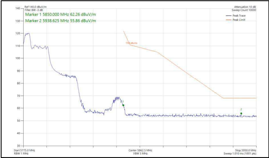
Figure 390 - 802.11ax, HE40, RU 52-37, SISO, Core 1 - 5795 MHz, Band Edge Frequency 5850 MHz
