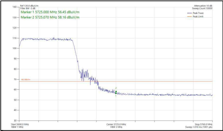
Figure 356 - 802.11ax, HE20, SU, TxBF, Core 0-1 - 5700 MHz, Band Edge Frequency 5725 MHz
