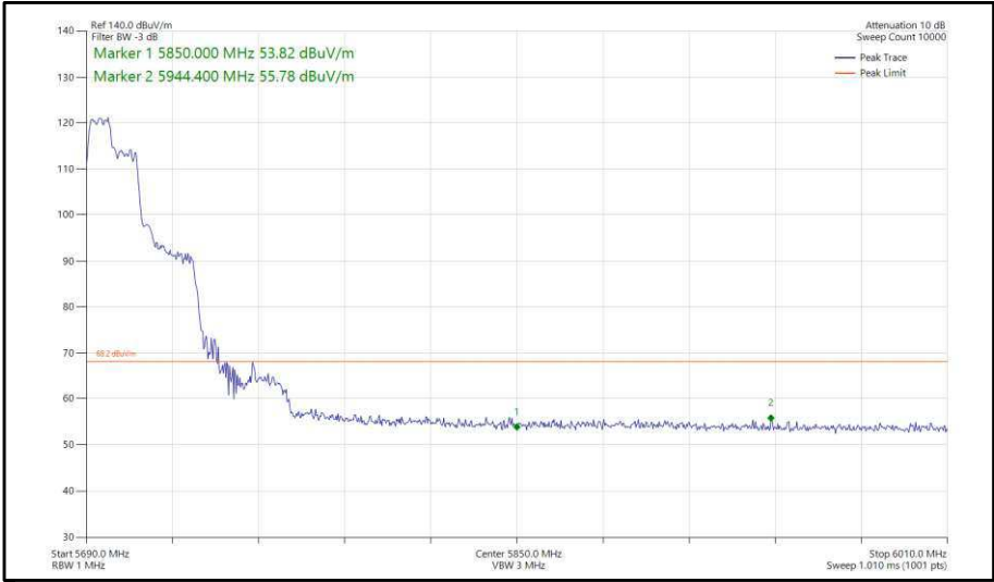
Figure 421 - 802.11ax, HE40, RU 106-53, SDM, Core 0-1 - 5710 MHz, Band Edge Frequency 5850 MHz
