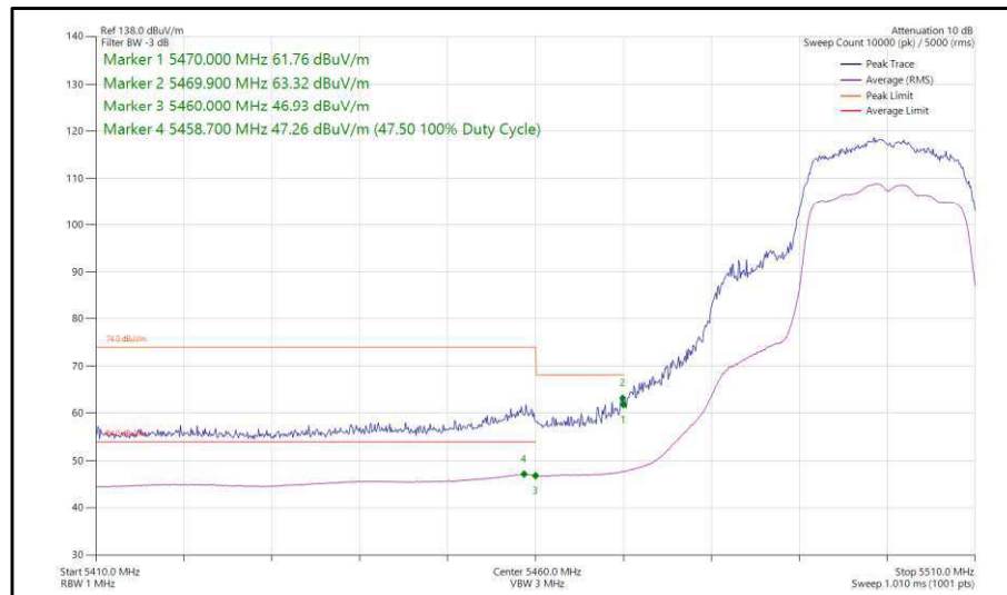
Figure 319 - 802.11n, HT20, CDD, Core 0-1 - 5500 MHz, Band Edge Frequency 5470 MHz
