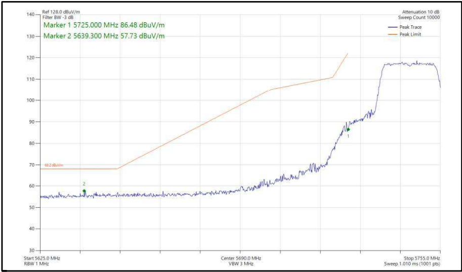
Figure 338 - 802.11n, HT20, SDM, Core 0-1 - 5745 MHz, Band Edge Frequency 5725 MHz
