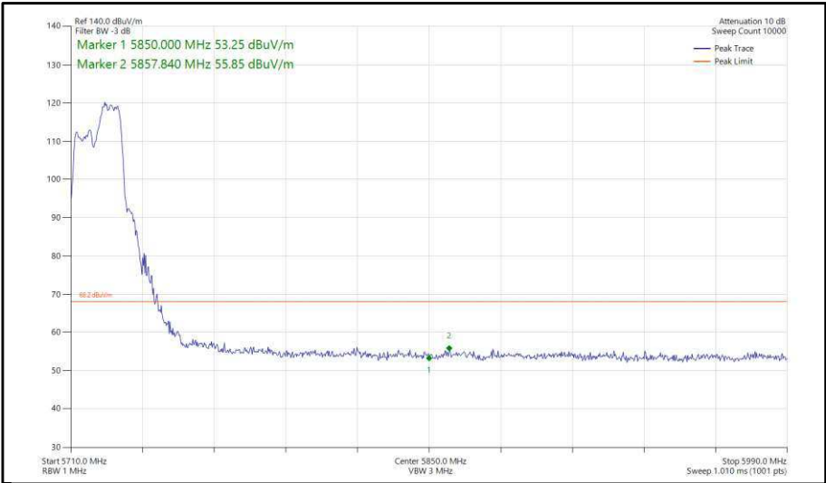
Figure 332 - 802.11ax, HE20, RU 106-54, CDD, Core 0-1 - 5720 MHz, Band Edge Frequency 5850 MHz
