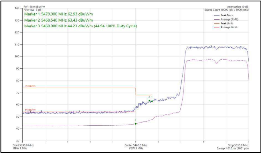
Figure 408 - 802.11ax, HE40, SU, SDM, Core 0-1 - 5510 MHz, Band Edge Frequency 5470 MHz
