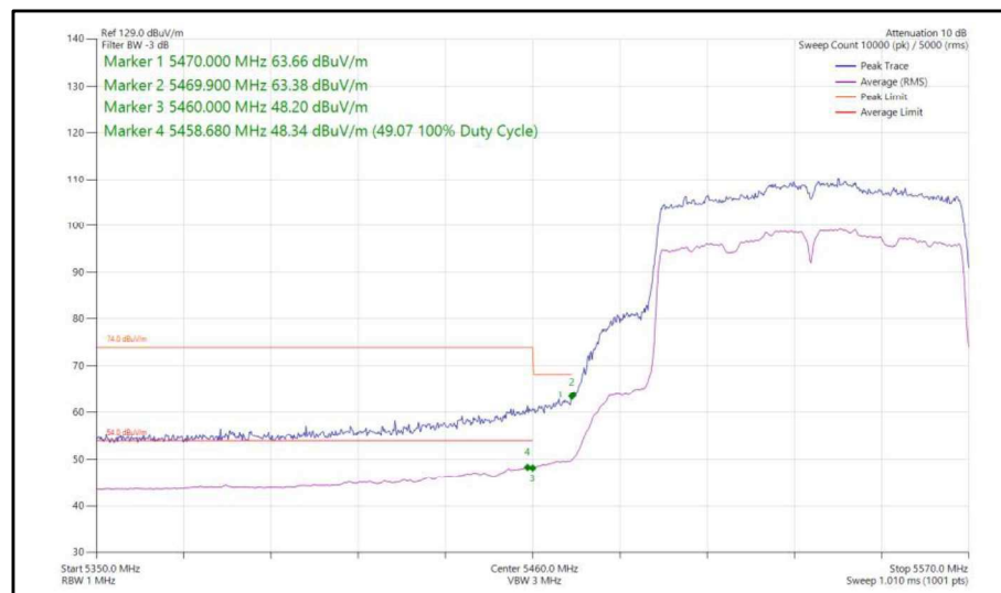
Figure 434 - 802.11ac, VHT80, SISO, Core 0 - 5530 MHz, Band Edge Frequency 5470 MHz
