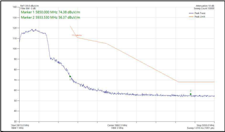
Figure 346 - 802.11n, HT20, SDM, Core 0-1 - 5825 MHz, Band Edge Frequency 5850 MHz
