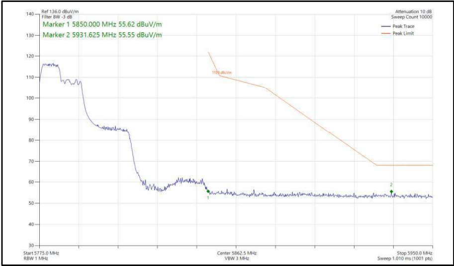
Figure 375 - 802.11ax, HE40, RU 106-53, SISO, Core 0 - 5795 MHz, Band Edge Frequency 5850 MHz
