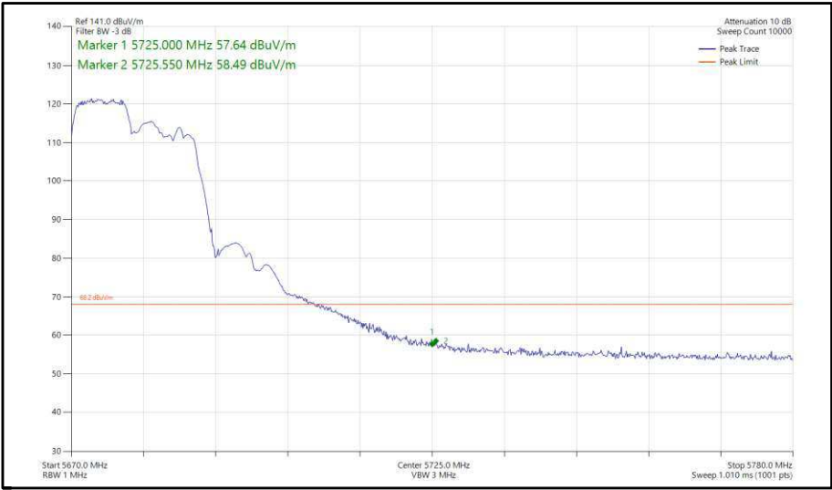
Figure 342 - 802.11ax, HE20, RU 106-53, SDM, Core 0-1 - 5680 MHz, Band Edge Frequency 5725 MHz
