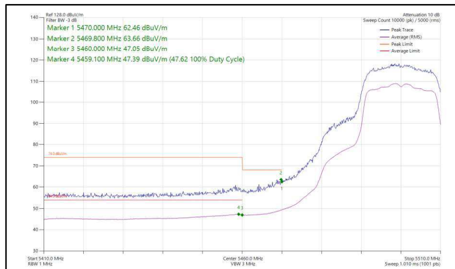
Figure 335 - 802.11n, HT20, SDM, Core 0-1 - 5500 MHz, Band Edge Frequency 5470 MHz
