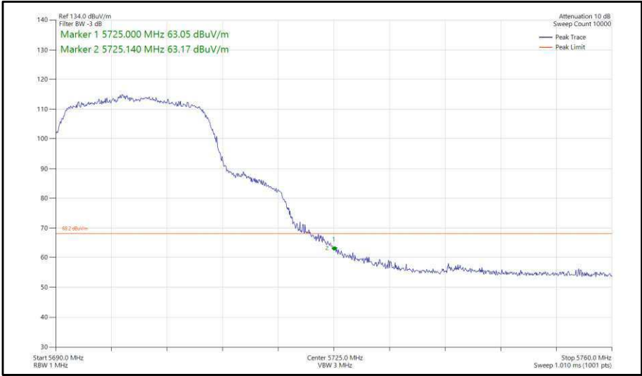
Figure 325 - 802.11n, HT20, CDD, Core 0-1 - 5700 MHz, Band Edge Frequency 5725 MHz
