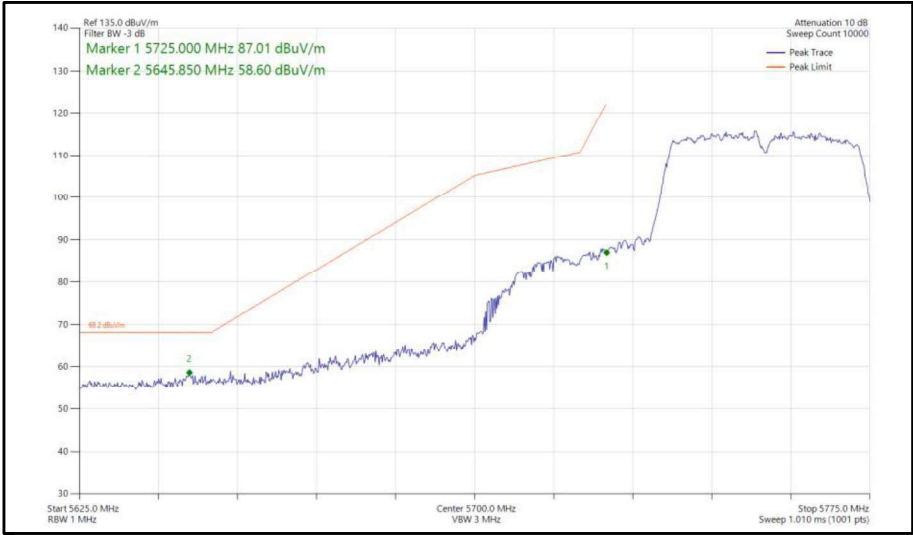
Figure 395 - 802.11n, HT40, CDD, Core 0-1 - 5755 MHz, Band Edge Frequency 5725 MHz
