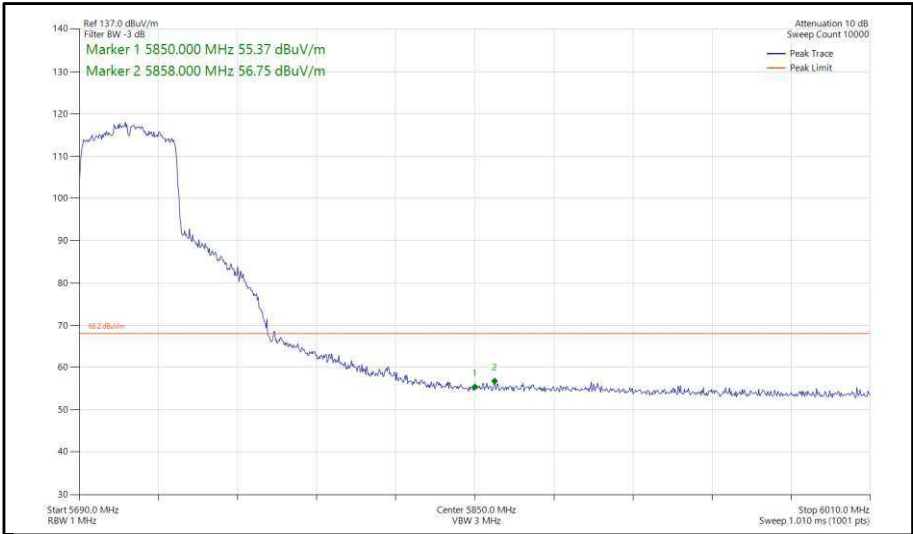
Figure 387 - 802.11ax, HE40, SU, SISO, Core 1 - 5710 MHz, Band Edge Frequency 5850 MHz
