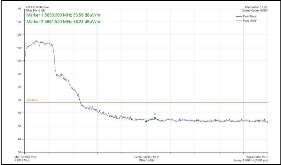
Figure 401 - 802.11n, HT40, CDD, Core 0-1 - 5710 MHz, Band Edge Frequency 5850 MHz
