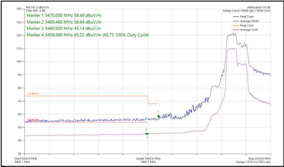
Figure 394 - 802.11ax, HE40, RU 106-53, CDD, Core 0-1 - 5550 MHz, Band Edge Frequency 5470 MHz
