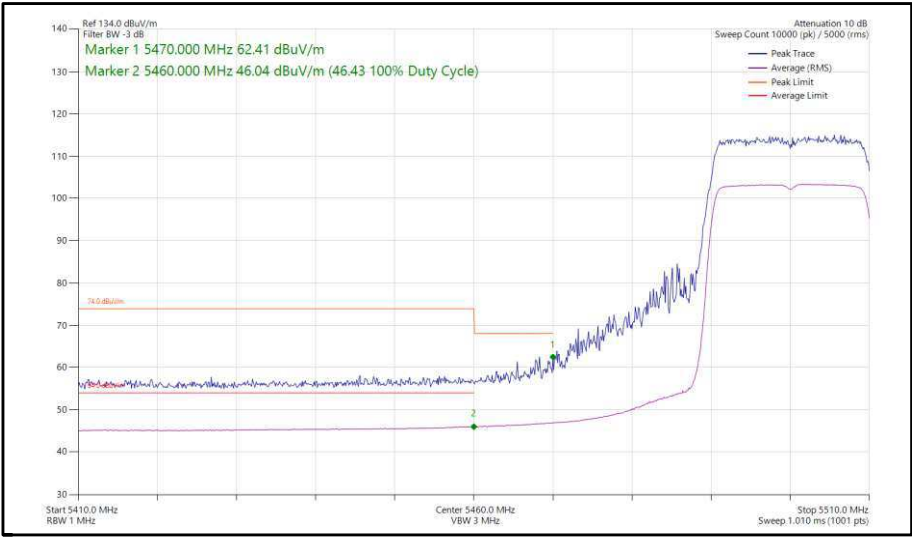
Figure 352 - 802.11ax, HE20, SU, TxBF, Core 0-1 - 5500 MHz, Band Edge Frequency 5470 MHz
