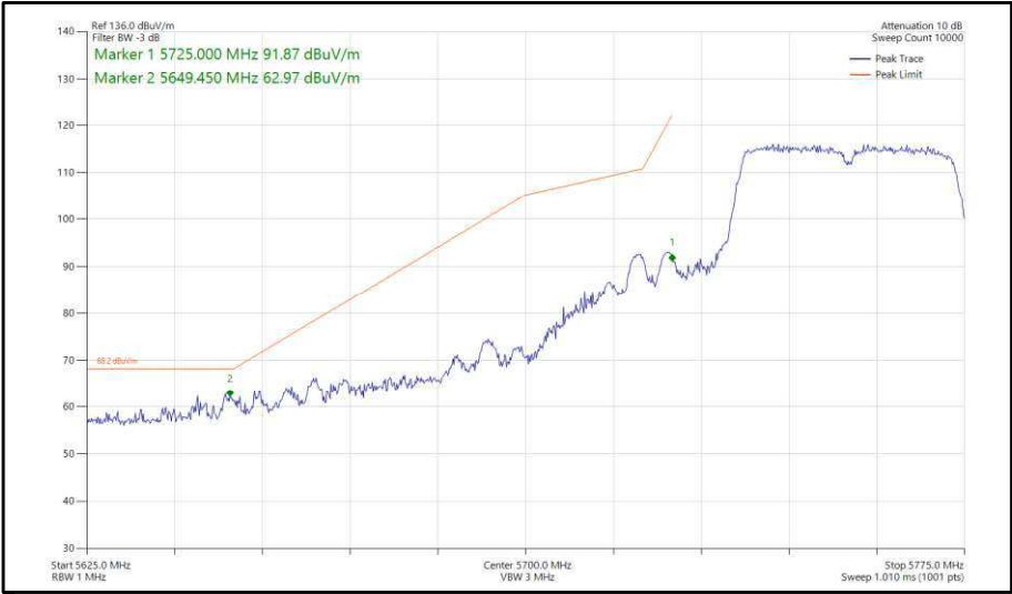
Figure 426 - 802.11ac, VHT40, TxBF, Core 0-1 - 5755 MHz, Band Edge Frequency 5725 MHz
