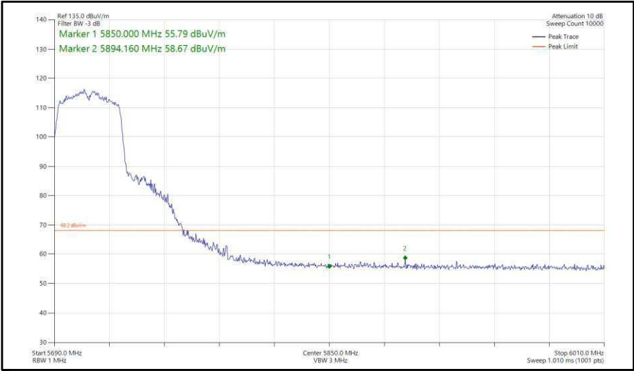
Figure 430 - 802.11ac, VHT40, TxBF, Core 0-1 - 5710 MHz, Band Edge Frequency 5850 MHz
