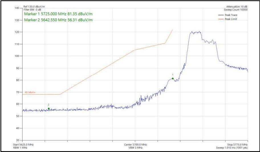
Figure 413 - 802.11ax, HE40, RU 106-53, SDM, Core 0-1 - 5755 MHz, Band Edge Frequency 5725 MHz
