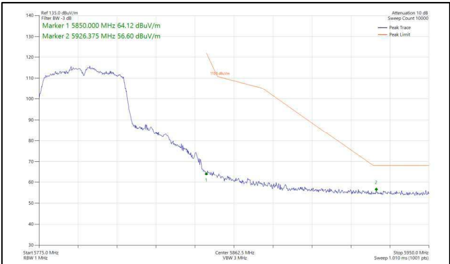
Figure 386 - 802.11n, HT40, SISO, Core 1 - 5795 MHz, Band Edge Frequency 5850 MHz
