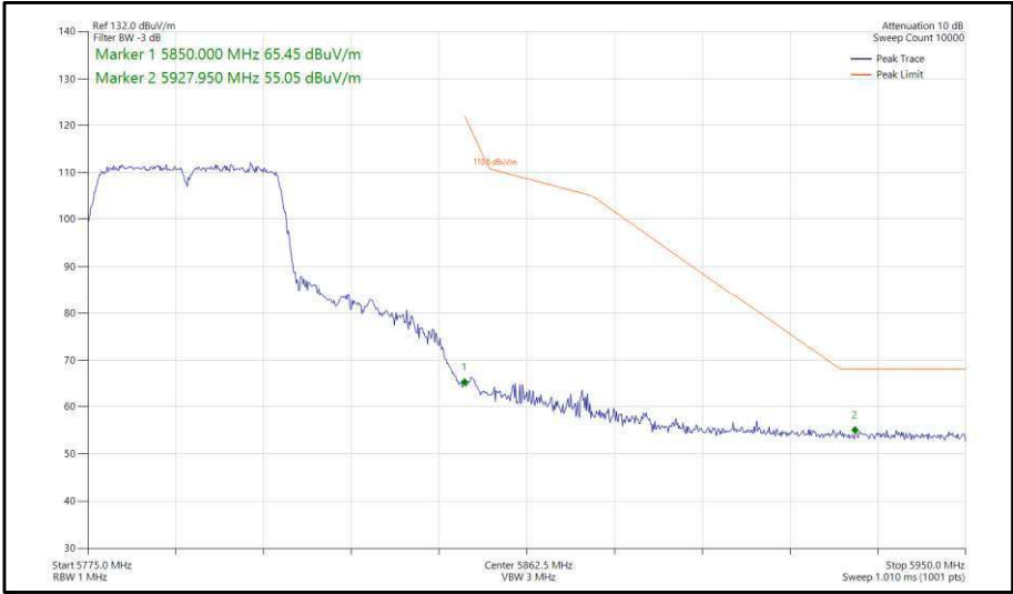
Figure 371 - 802.11n, HT40, SISO, Core 0 - 5795 MHz, Band Edge Frequency 5850 MHz
