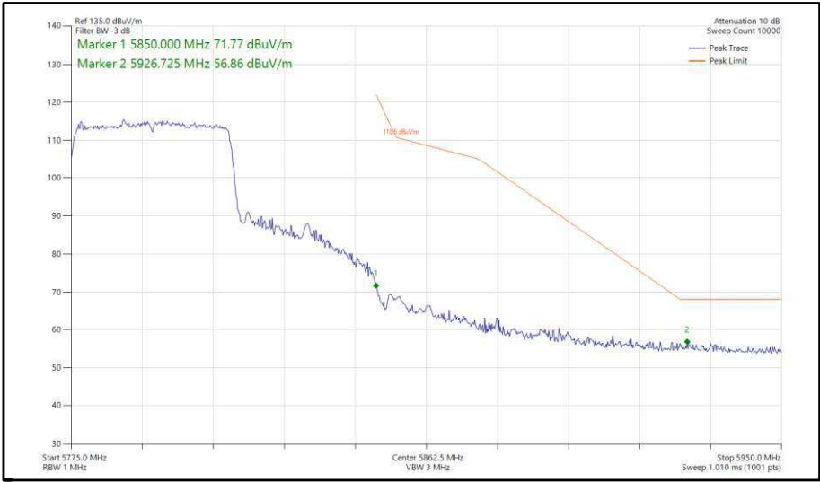
Figure 389 - 802.11ax, HE40, SU, SISO, Core 1 - 5795 MHz, Band Edge Frequency 5850 MHz
