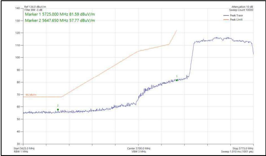
Figure 380 - 802.11ax, HE40, SU, SISO, Core 1 - 5755 MHz, Band Edge Frequency 5725 MHz
