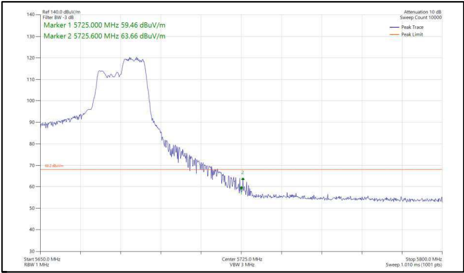
Figure 400 - 802.11ax, HE40, RU 106-56, CDD, Core 0-1 - 5670 MHz, Band Edge Frequency 5725 MHz
