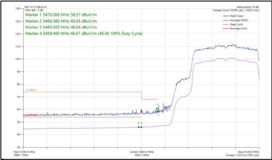
Figure 425 - 802.11ax, HE40, SU, TxBF, Core 0-1 - 5510 MHz, Band Edge Frequency 5470 MHz
