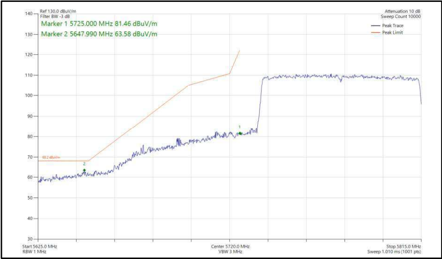
Figure 438 - 802.11ax, HE80, SU, SISO, Core 0 - 5775 MHz, Band Edge Frequency 5725 MHz
