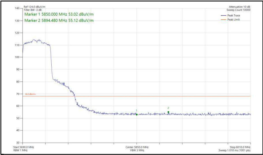
Figure 372 - 802.11ax, HE40, SU, SISO, Core 0 - 5710 MHz, Band Edge Frequency 5850 MHz
