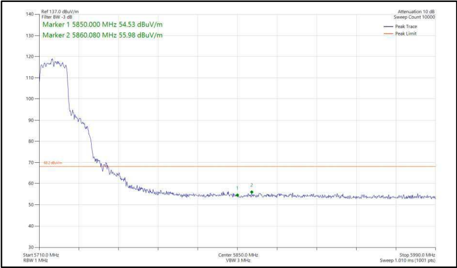
Figure 331 - 802.11ax, HE20, SU, CDD, Core 0-1 - 5720 MHz, Band Edge Frequency 5850 MHz
