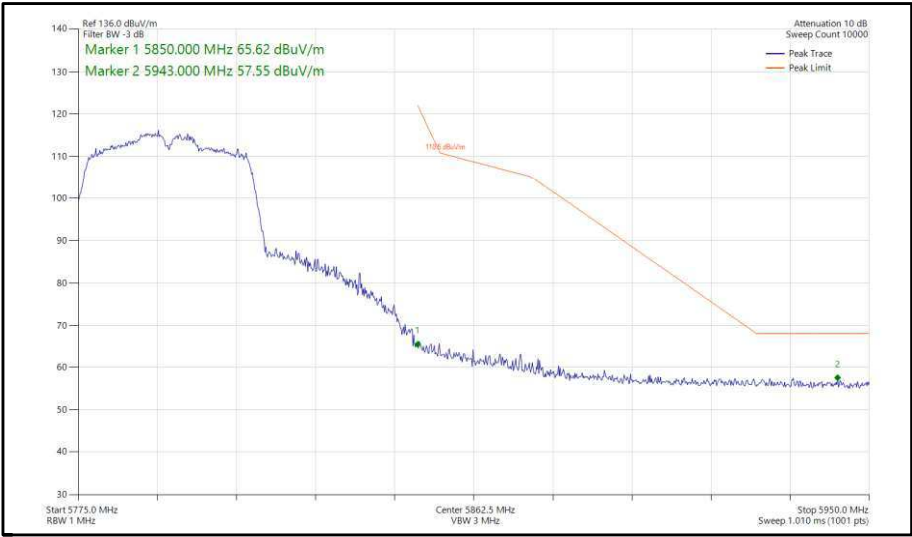
Figure 431 - 802.11ac, VHT40, TxBF, Core 0-1 - 5795 MHz, Band Edge Frequency 5850 MHz
