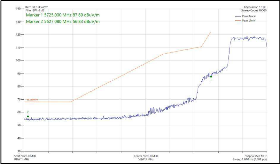
Figure 323 - 802.11ax, HE20, SU, CDD, Core 0-1 - 5745 MHz, Band Edge Frequency 5725 MHz
