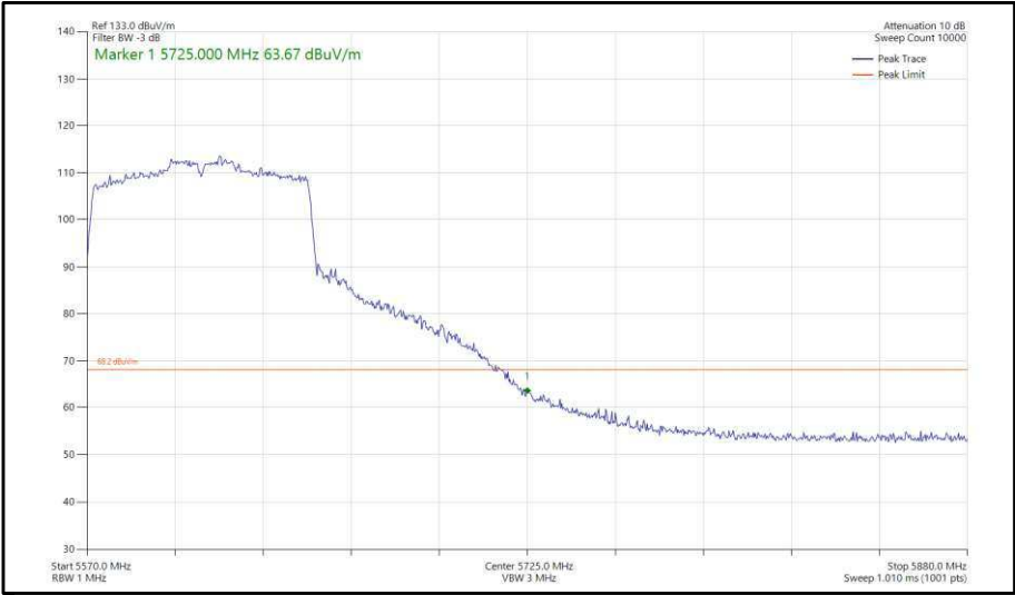
Figure 440 - 802.11ac, VHT80, SISO, Core 0 - 5610 MHz, Band Edge Frequency 5725 MHz
