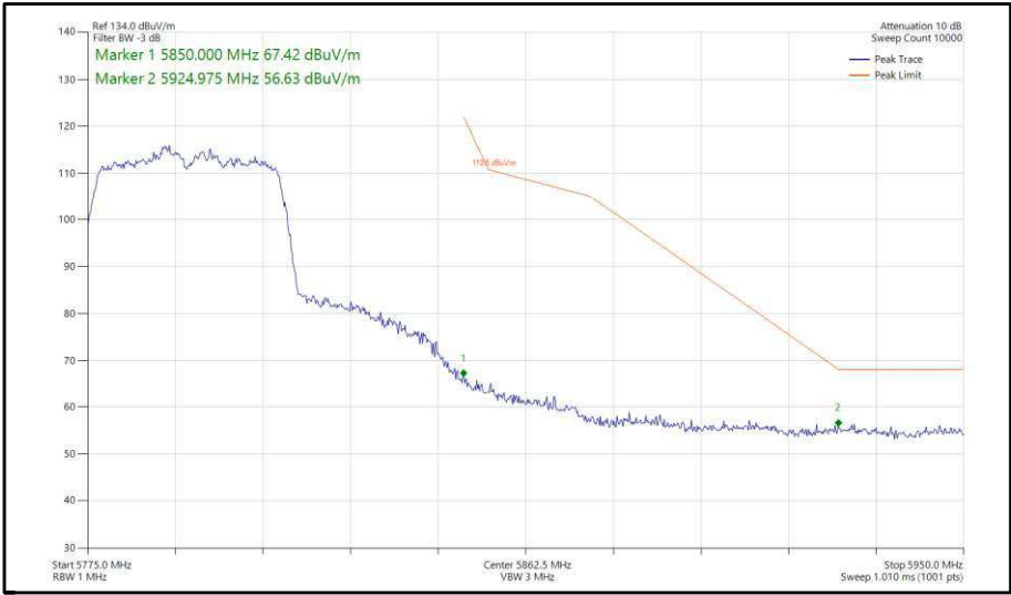
Figure 402 - 802.11n, HT40, CDD, Core 0-1 - 5795 MHz, Band Edge Frequency 5850 MHz
