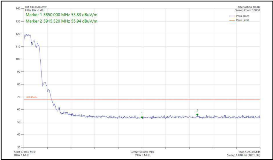
Figure 348 - 802.11ax HE20, RU 106-53, SDM, Core 0-1 - 5720 MHz, Band Edge Frequency 5850 MHz
