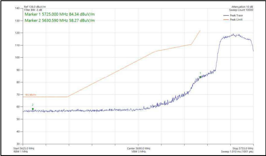
Figure 353 - 802.11ac, VHT20, TxBF, Core 0-1 - 5745 MHz, Band Edge Frequency 5725 MHz
