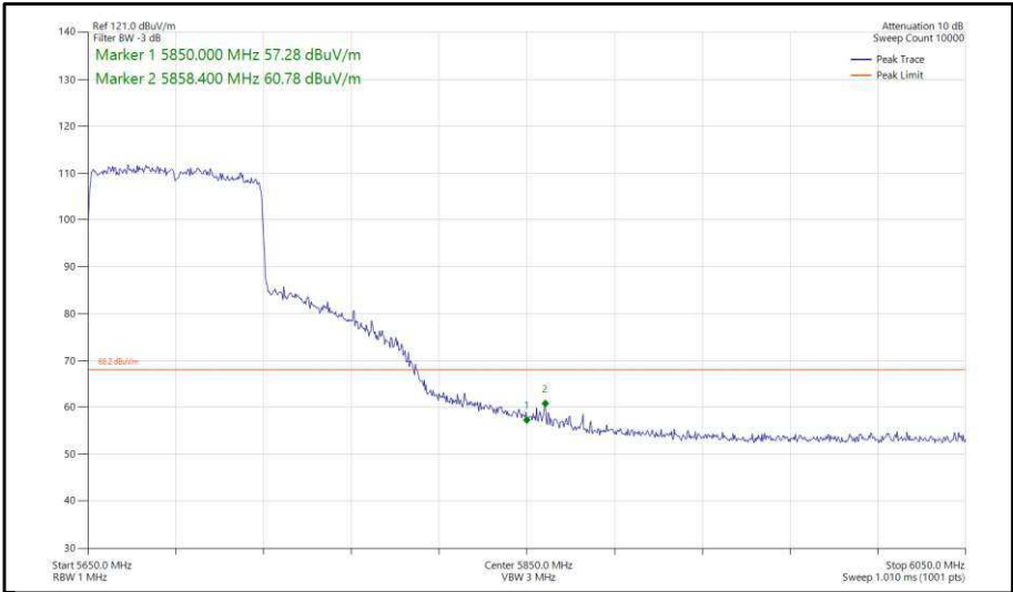
Figure 445 - 802.11ax, HE80, SU, SISO, Core 0 - 5690 MHz, Band Edge Frequency 5850 MHz
