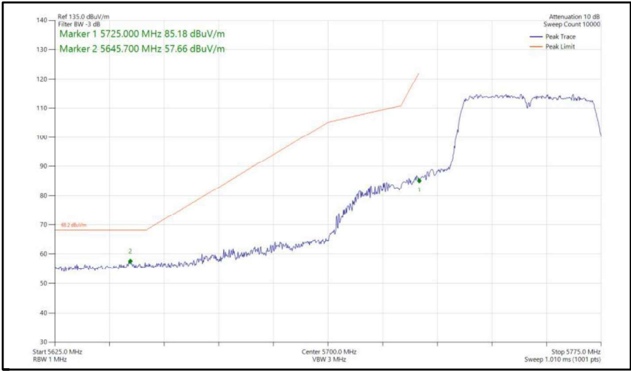
Figure 379 - 802.11n, HT40, SISO, Core 1 - 5755 MHz, Band Edge Frequency 5725 MHz
