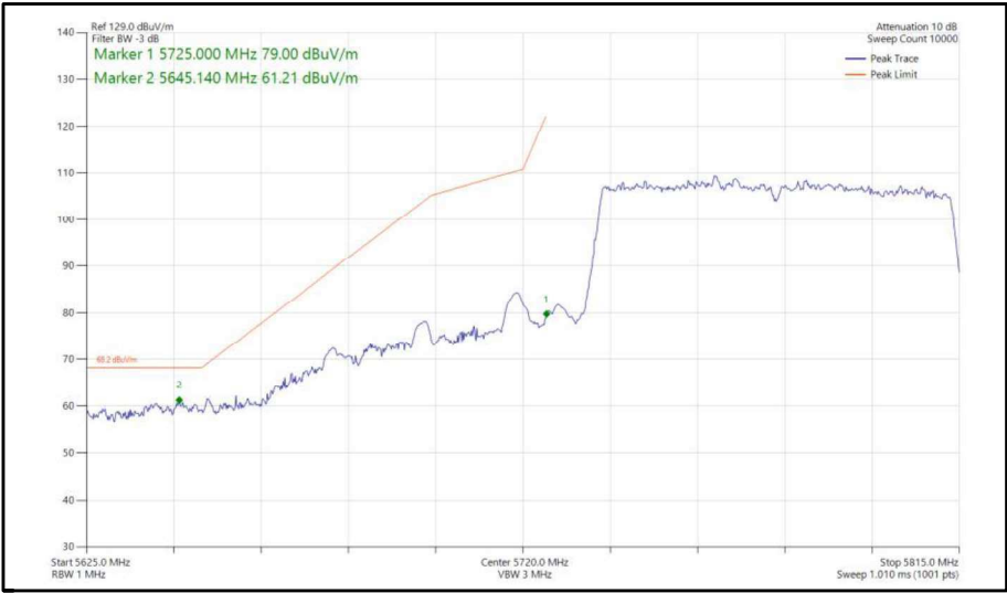
Figure 437 - 802.11ac, VHT80, SISO, Core 0 - 5775 MHz, Band Edge Frequency 5725 MHz
