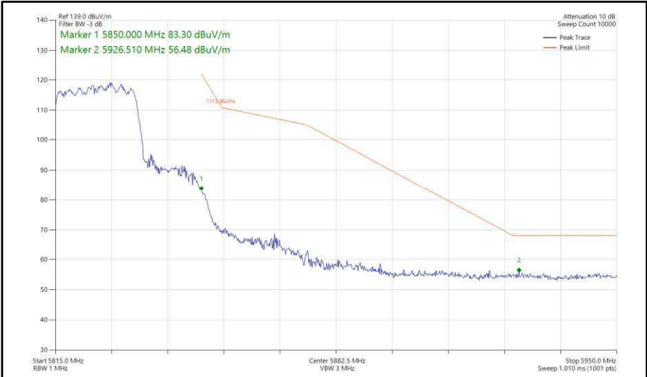
Figure 333 - 802.11ax, HE20, SU, CDD, Core 0-1 - 5825 MHz, Band Edge Frequency 5850 MHz
