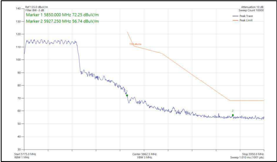
Figure 405 - 802.11ax, HE40, SU, CDD, Core 0-1 - 5795 MHz, Band Edge Frequency 5850 MHz
