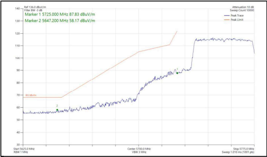
Figure 396 - 802.11ax, HE40, SU, CDD, Core 0-1 - 5755 MHz, Band Edge Frequency 5725 MHz
