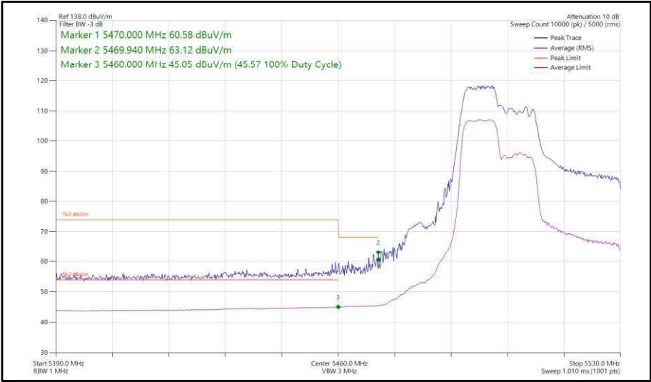
Figure 409 - 802.11ax, HE40, RU 106-53, SDM, Core 0-1 - 5510 MHz, Band Edge Frequency 5470 MHz
