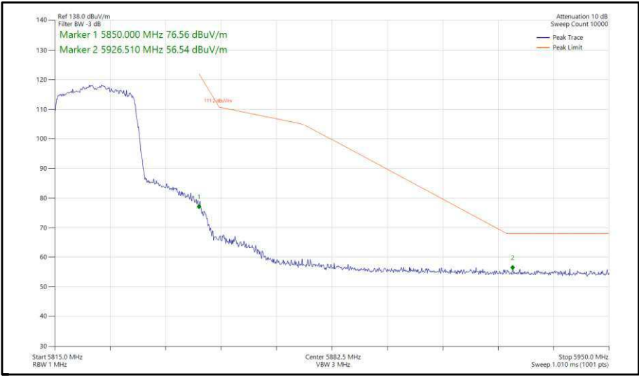
Figure 317 - 802.11ax, HE20, SU, SISO, Core 1 - 5825 MHz, Band Edge Frequency 5850 MHz
