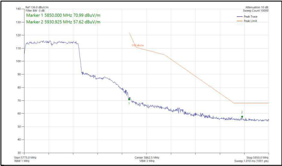
Figure 422 - 802.11ax, HE40, SU, SDM, Core 0-1 - 5795 MHz, Band Edge Frequency 5850 MHz
