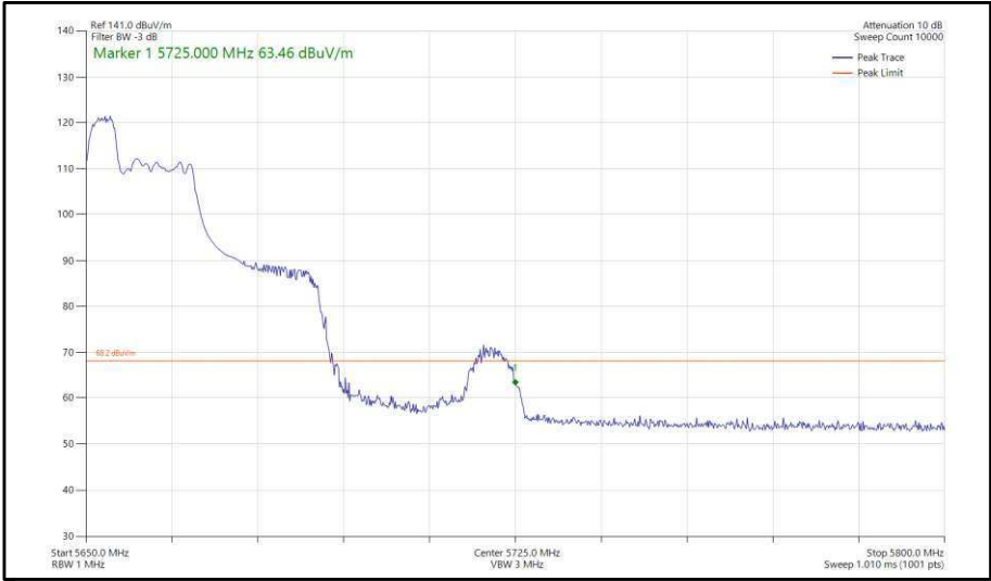
Figure 384 - 802.11ax, HE40, RU 52-37, SISO, Core 1 - 5670 MHz, Band Edge Frequency 5725 MHz
