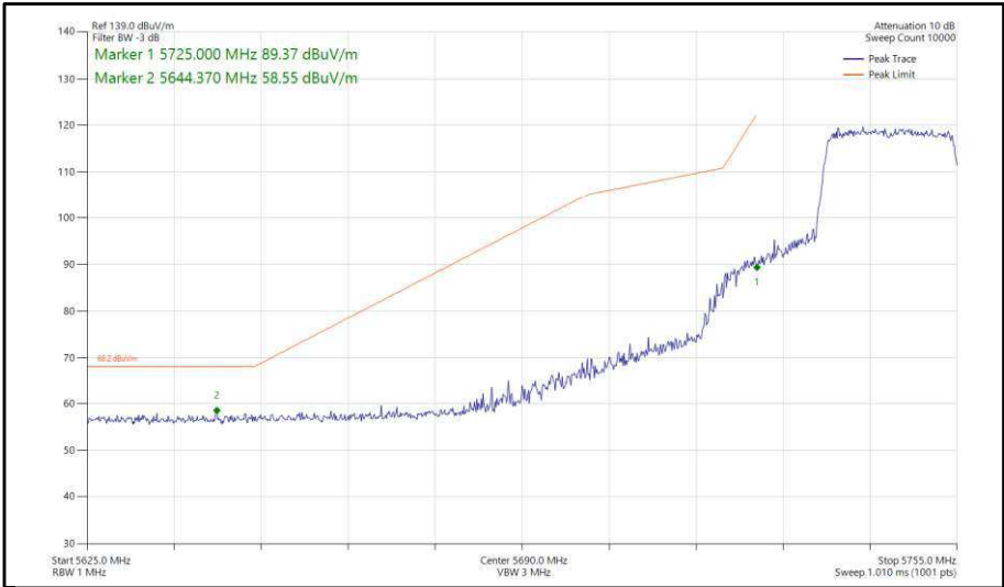
Figure 354 - 802.11ax, HE20, SU, TxBF, Core 0-1 - 5745 MHz, Band Edge Frequency 5725 MHz
