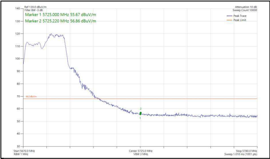
Figure 326 - 802.11ax, HE20, RU 106-54, CDD, Core 0-1 - 5680 MHz, Band Edge Frequency 5725 MHz
