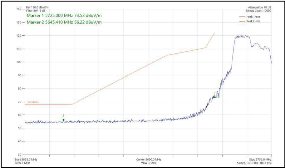
Figure 340 - 802.11ax, HE20, RU 106-53, SDM, Core 0-1 - 5745 MHz, Band Edge Frequency 5725 MHz
