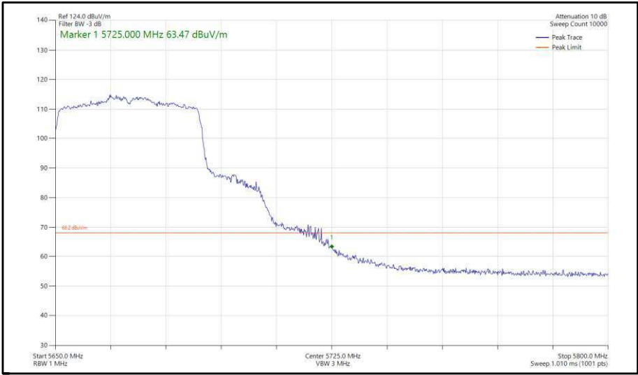
Figure 416 - 802.11ax, HE40, SU, SDM, Core 0-1 - 5670 MHz, Band Edge Frequency 5725 MHz
