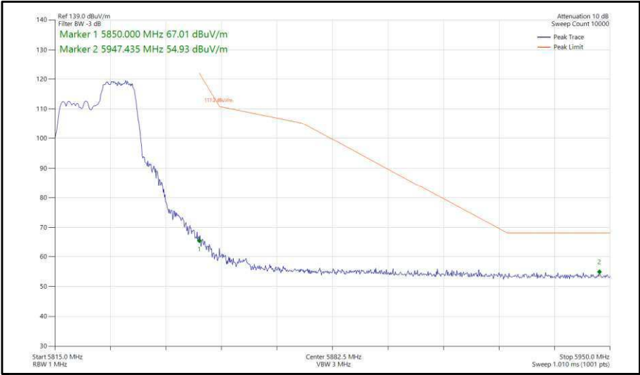
Figure 318 - 802.11ax, HE20, RU 106-54, SISO, Core 1 - 5825 MHz, Band Edge Frequency 5850 MHz
