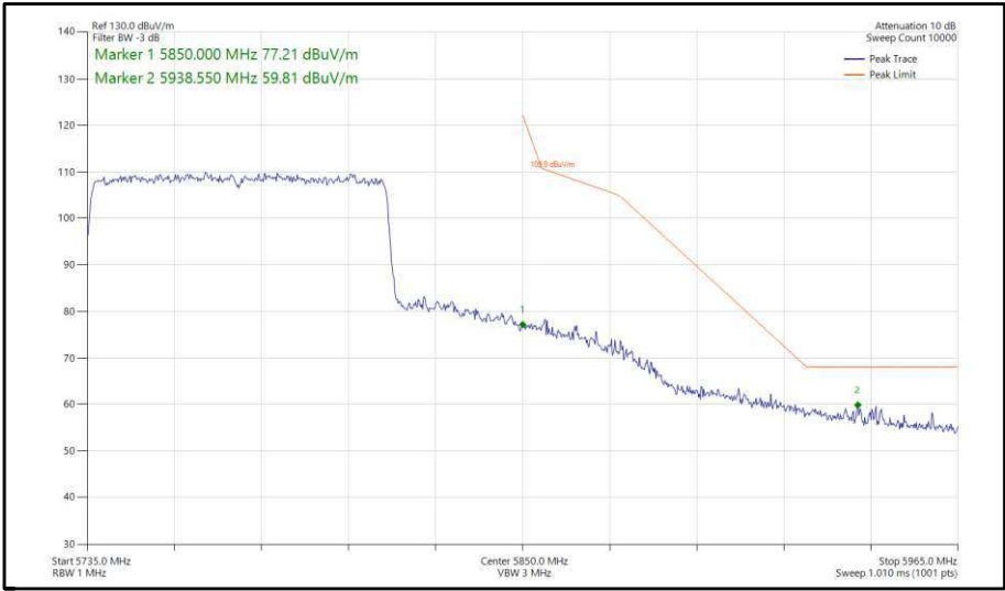
Figure 447 - 802.11ax, HE80, SU, SISO, Core 0 - 5775 MHz, Band Edge Frequency 5850 MHz
