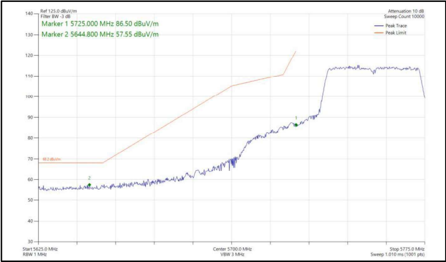
Figure 411 - 802.11n, HT40, SDM, Core 0-1 - 5755 MHz, Band Edge Frequency 5725 MHz
