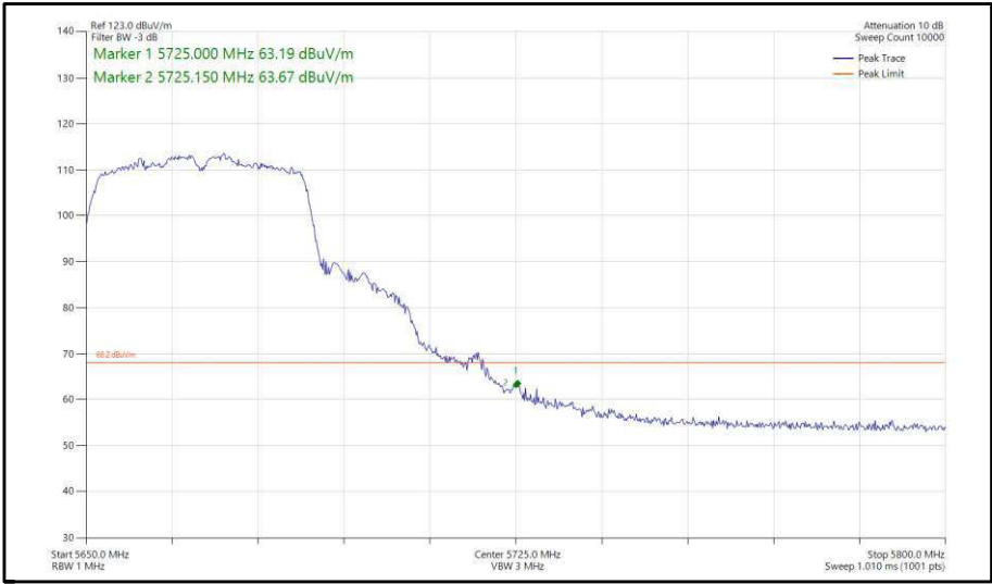
Figure 414 - 802.11n, HT40, SDM, Core 0-1 - 5670 MHz, Band Edge Frequency 5725 MHz
