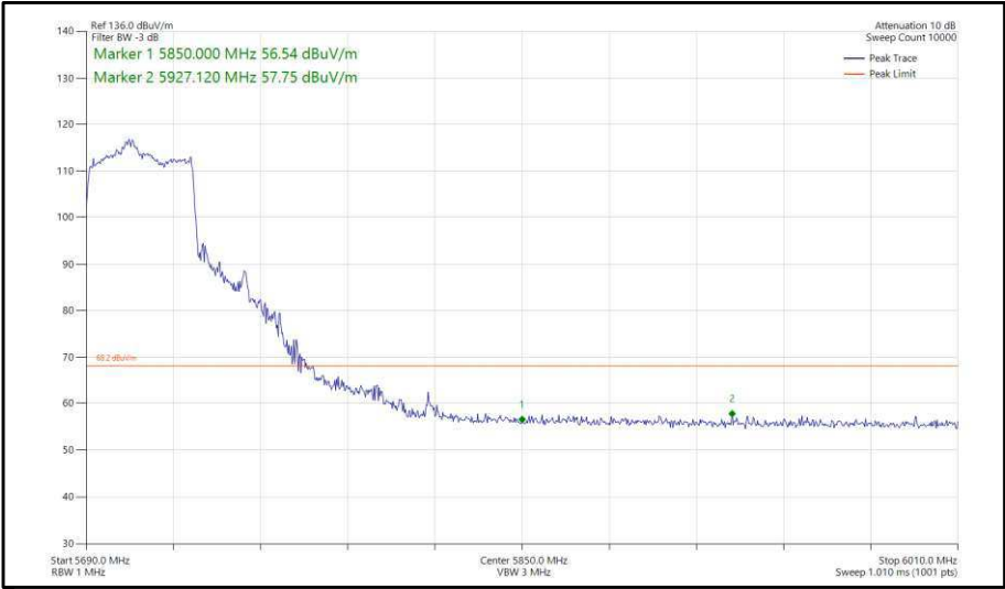
Figure 432 - 802.11ax, HE40, SU, TxBF, Core 0-1 - 5710 MHz, Band Edge Frequency 5850 MHz
