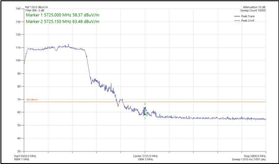
Figure 428 - 802.11ac, VHT40, TxBF, Core 0-1 - 5670 MHz, Band Edge Frequency 5725 MHz
