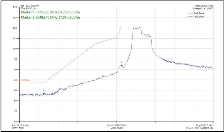
Figure 454 - 802.11ax, HE80, RU 106-53, SISO, Core 1 - 5775 MHz, Band Edge Frequency 5725 MHz
