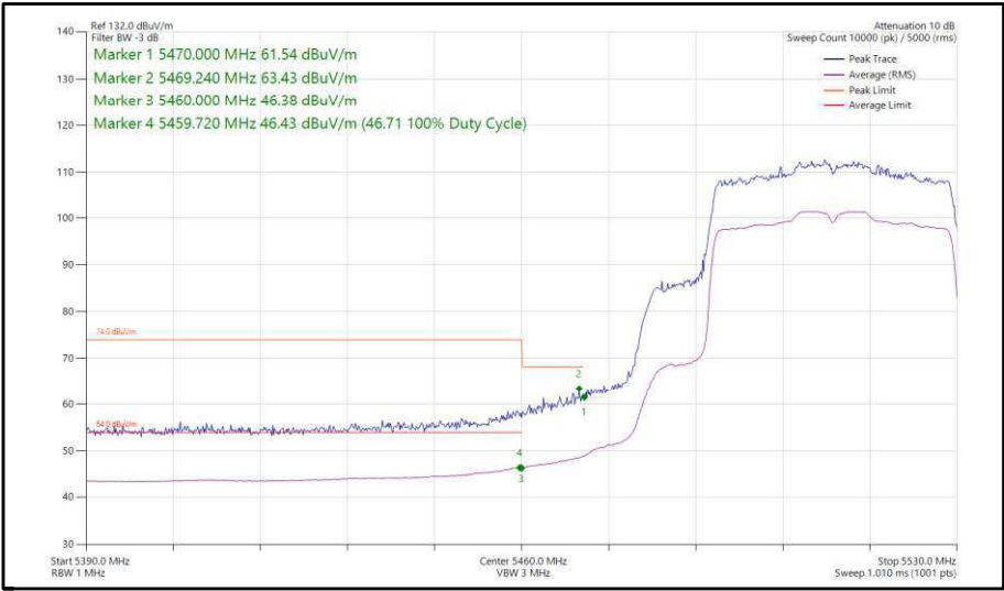
Figure 362 - 802.11ax, HE40, SU, SISO, Core 0 - 5510 MHz, Band Edge Frequency 5470 MHz
