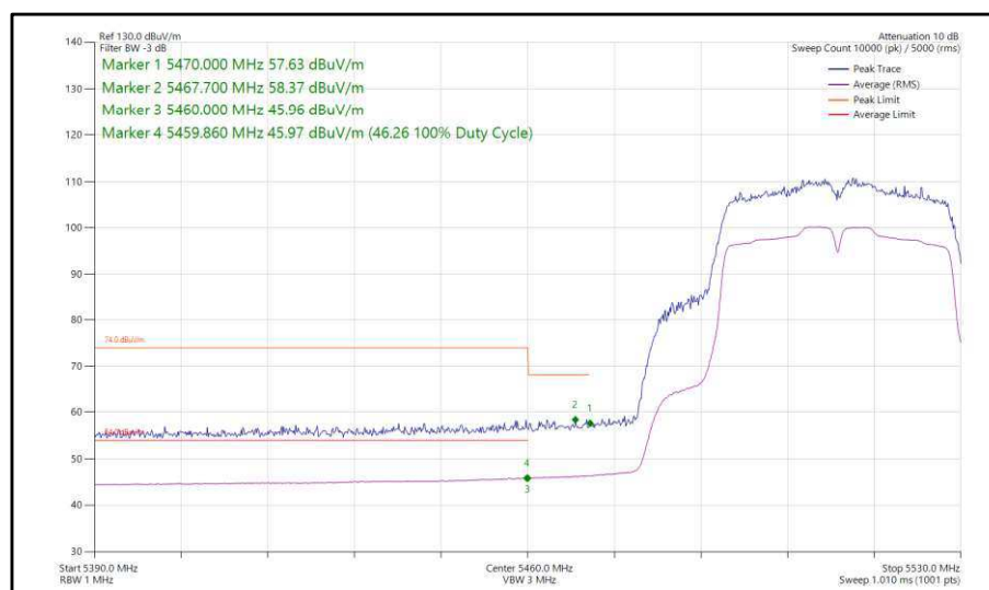
Figure 424 - 802.11ac, VHT40, TxBF, Core 0-1 - 5510 MHz, Band Edge Frequency 5470 MHz
