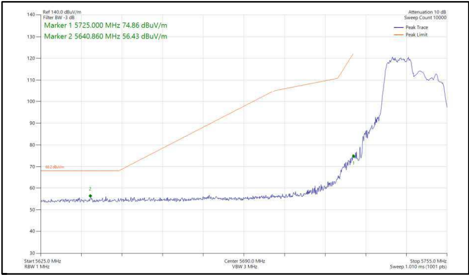
Figure 324 - 802.11ax, HE20, RU 106-53, CDD, Core 0-1 - 5745 MHz, Band Edge Frequency 5725 MHz
