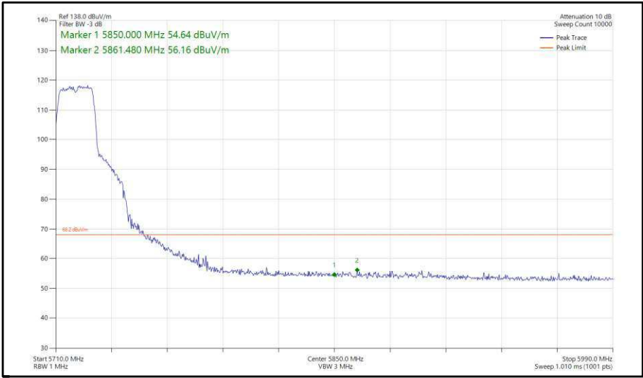
Figure 313 - 802.11n, HT20, SISO, Core 1 - 5720 MHz, Band Edge Frequency 5850 MHz
