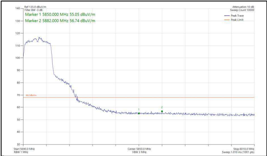
Figure 385 - 802.11n, HT40, SISO, Core 1 - 5710 MHz, Band Edge Frequency 5850 MHz
