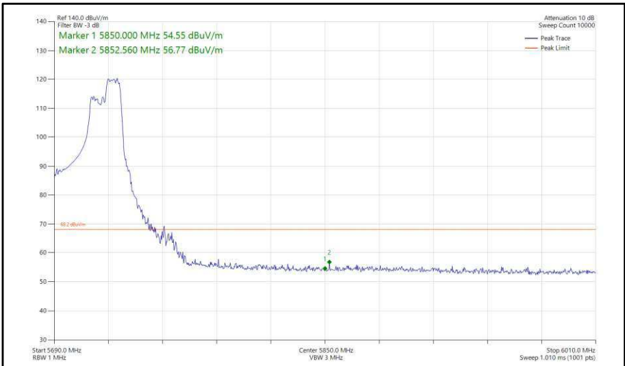
Figure 388 - 802.11ax, HE40, RU 106-56, SISO, Core 1 - 5710 MHz, Band Edge Frequency 5850 MHz
