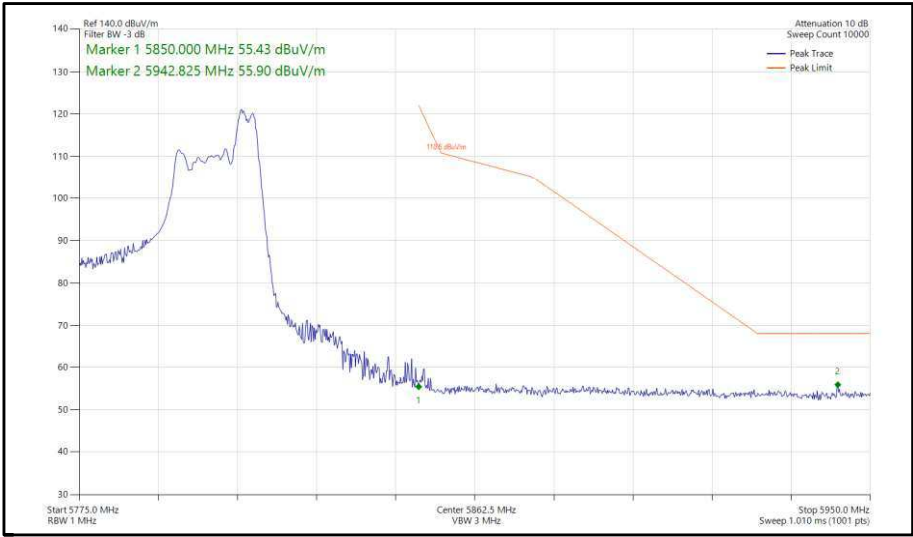
Figure 406 - 802.11ax, HE40, RU 52-44, CDD, Core 0-1 - 5795 MHz, Band Edge Frequency 5850 MHz
