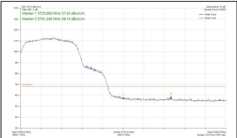
Figure 355 - 802.11ac, VHT20, TxBF, Core 0-1 - 5700 MHz, Band Edge Frequency 5725 MHz
