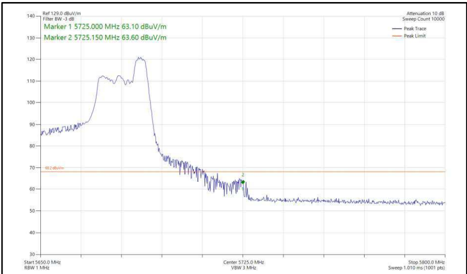
Figure 417 - 802.11ax, HE40, RU 52-44, SDM, Core 0-1 - 5670 MHz, Band Edge Frequency 5725 MHz
