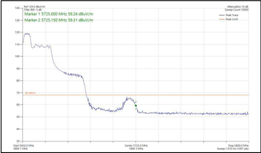
Figure 369 - 802.11ax, HE40, RU 52-37, SISO, Core 0 - 5670 MHz, Band Edge Frequency 5725 MHz
