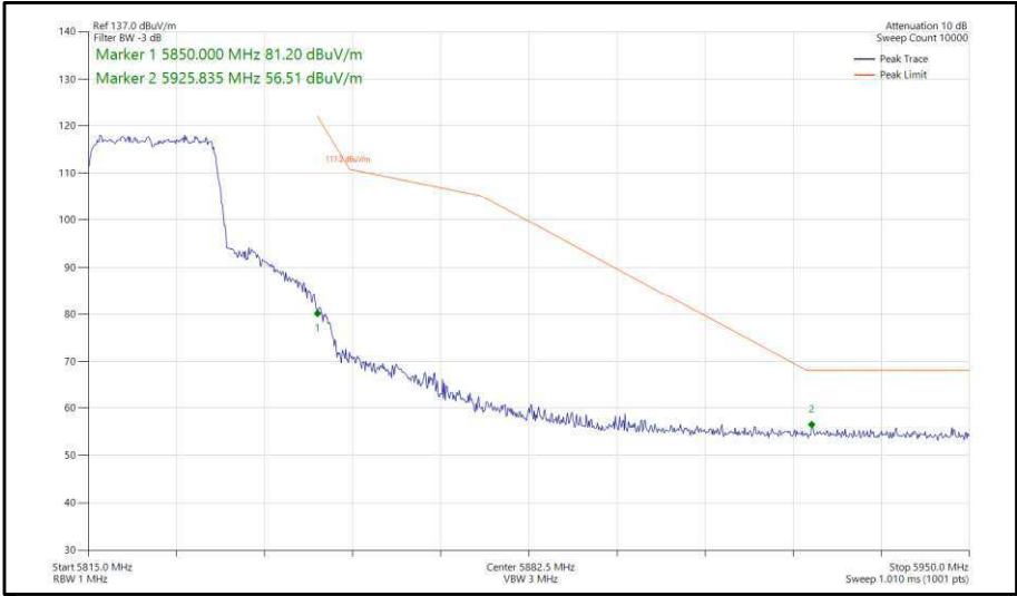
Figure 349 - 802.11ax, HE20, SU, SDM, Core 0-1 - 5825 MHz, Band Edge Frequency 5850 MHz
