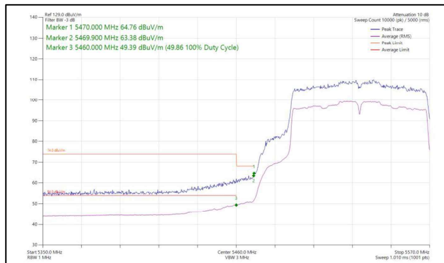
Figure 449 - 802.11ac, VHT80, SISO, Core 1 - 5530 MHz, Band Edge Frequency 5470 MHz
