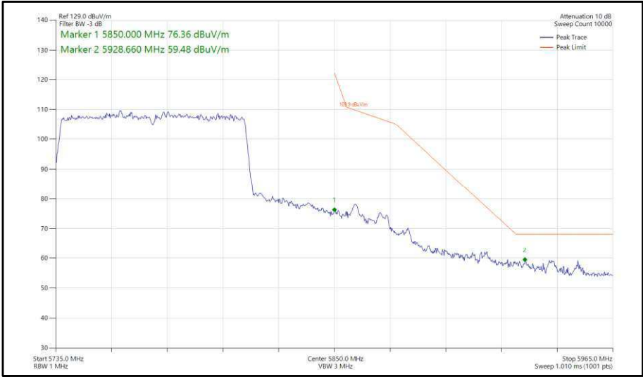
Figure 444 - 802.11ac, VHT80, SISO, Core 0 - 5775 MHz, Band Edge Frequency 5850 MHz
