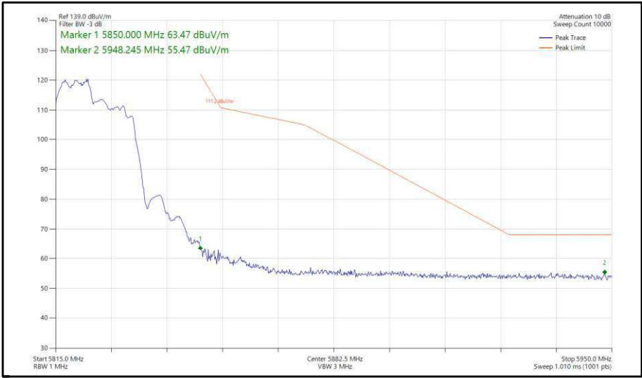
Figure 334 - 802.11ax, HE20, RU 106-53, CDD, Core 0-1 - 5825 MHz, Band Edge Frequency 5850 MHz
