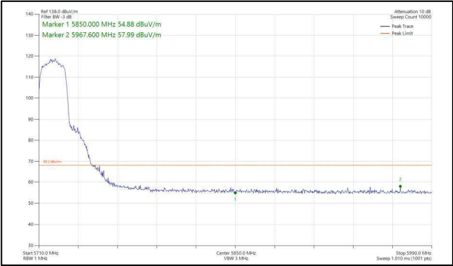
Figure 357 - 802.11ac, VHT20, TxBF, Core 0-1 - 5720 MHz, Band Edge Frequency 5850 MHz
