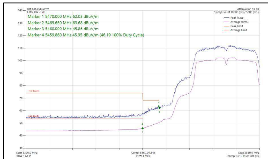
Figure 376 - 802.11n, HT40, SISO, Core 1 - 5510 MHz, Band Edge Frequency 5470 MHz
