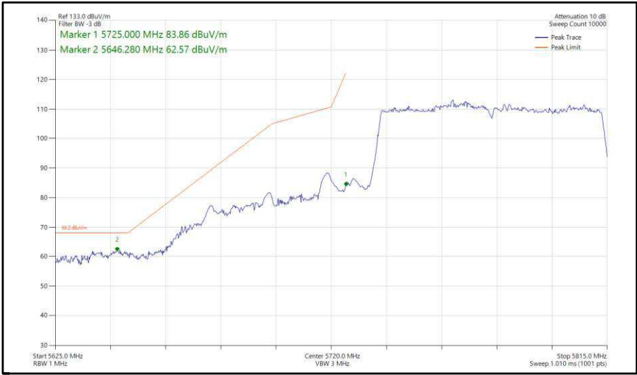
Figure 452 - 802.11ac, VHT80, SISO, Core 1 - 5775 MHz, Band Edge Frequency 5725 MHz
