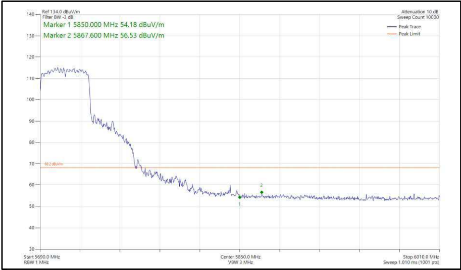
Figure 403 - 802.11ax, HE40, SU, CDD, Core 0-1 - 5710 MHz, Band Edge Frequency 5850 MHz
