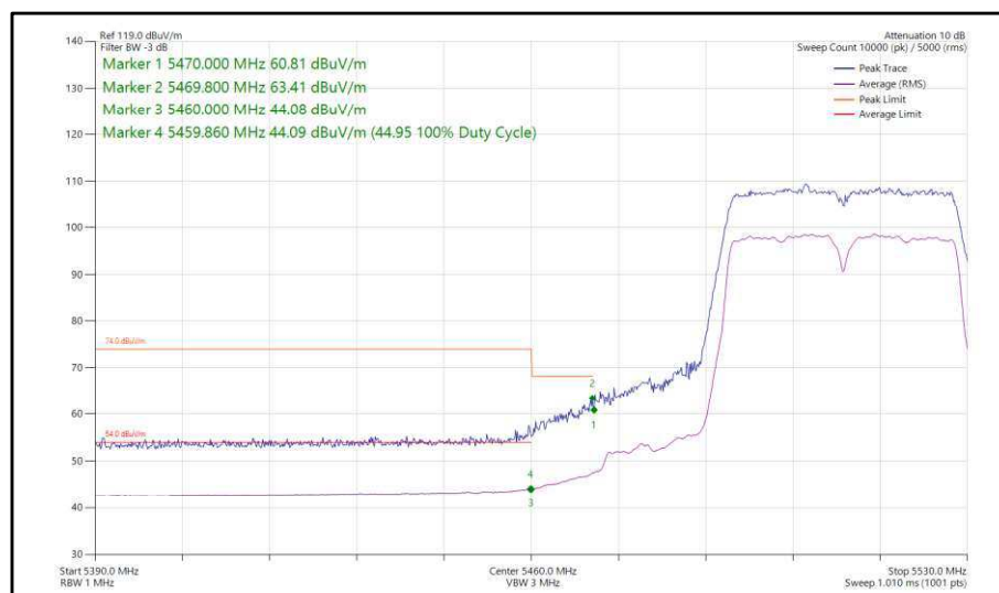
Figure 407 - 802.11n, HT40, SDM, Core 0-1 - 5510 MHz, Band Edge Frequency 5470 MHz
