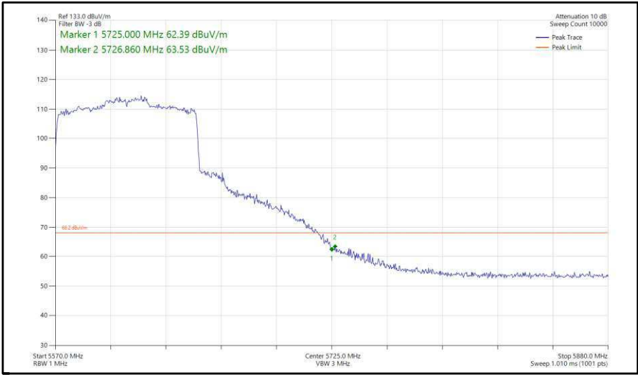
Figure 441 - 802.11ax, HE80, SU, SISO, Core 0 - 5610 MHz, Band Edge Frequency 5725 MHz
