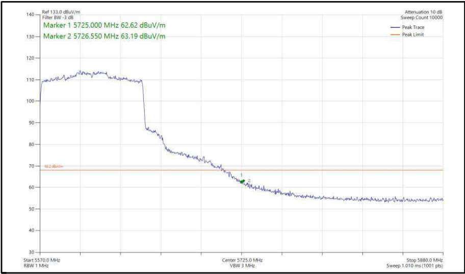
Figure 456 - 802.11ax, HE80, SU, SISO, Core 1 - 5610 MHz, Band Edge Frequency 5725 MHz
