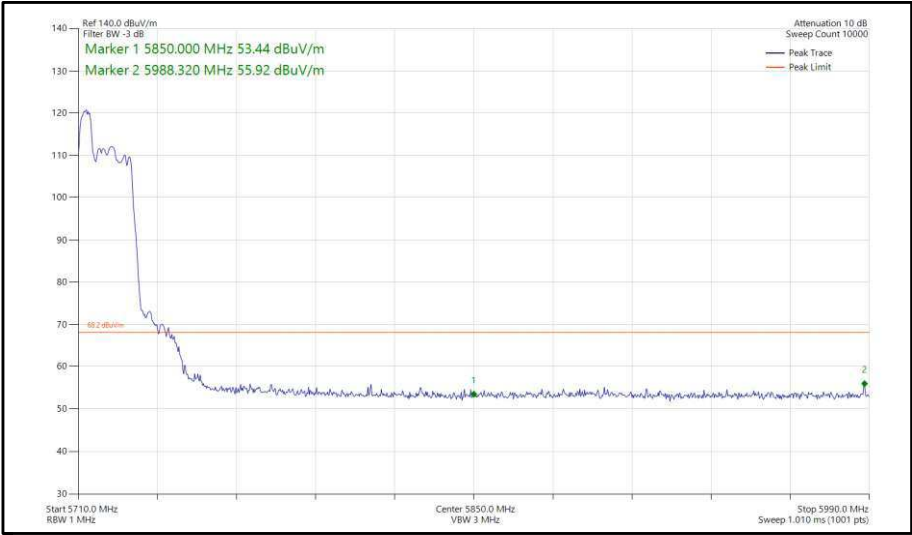
Figure 316 - 802.11ax, HE20, RU 52-37, SISO, Core 1 - 5720 MHz, Band Edge Frequency 5850 MHz
