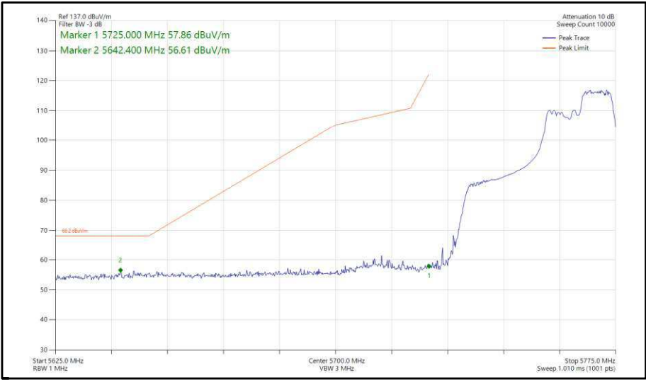
Figure 366 - 802.11ax, HE40, RU 106-56, SISO, Core 0 - 5755 MHz, Band Edge Frequency 5725 MHz
