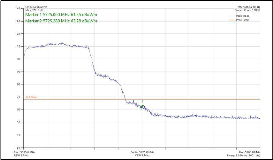
Figure 343 - 802.11ax, HE20, SU, SDM, Core 0-1 - 5700 MHz, Band Edge Frequency 5725 MHz
