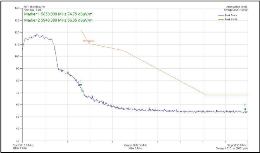
Figure 330 - 802.11n, HT20, CDD, Core 0-1 - 5825 MHz, Band Edge Frequency 5850 MHz
