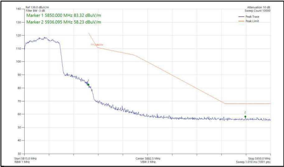
Figure 360 - 802.11ax, HE20, SU, TxBF, Core 0-1 - 5825 MHz, Band Edge Frequency 5850 MHz
