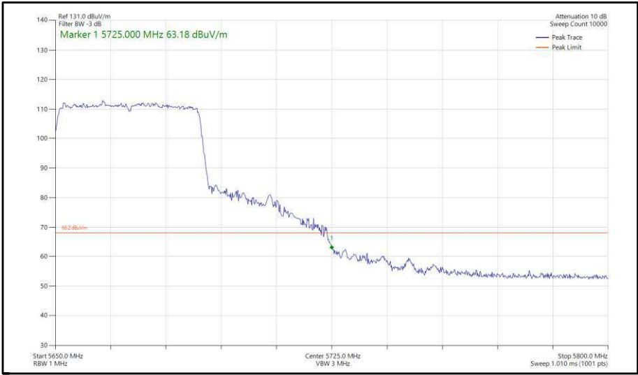
Figure 368 - 802.11ax, HE40, SU, SISO, Core 0 - 5670 MHz, Band Edge Frequency 5725 MHz
