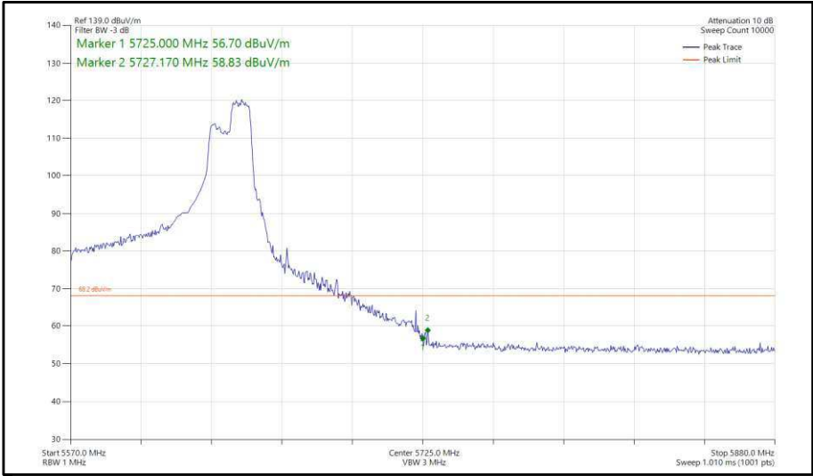
Figure 442 - 802.11ax, HE80, RU 106-60, SISO, Core 0 - 5610 MHz, Band Edge Frequency 5725 MHz
