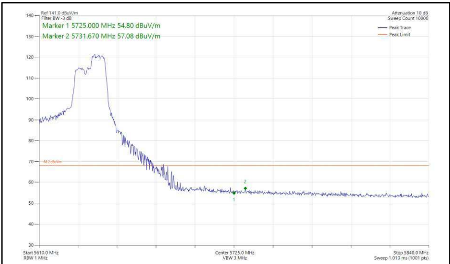
Figure 415 - 802.11ax, HE40, RU 106-56, SDM, Core 0-1 - 5630 MHz, Band Edge Frequency 5725 MHz
