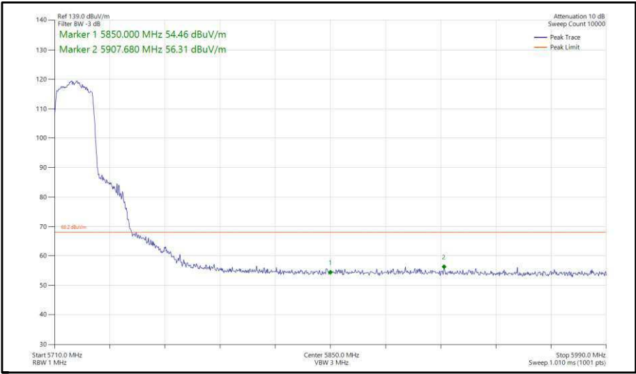
Figure 315 - 802.11ax, HE20, SU, SISO, Core 1 - 5720 MHz, Band Edge Frequency 5850 MHz
