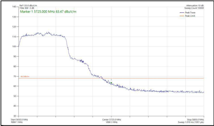
Figure 398 - 802.11n, HT40, CDD, Core 0-1 - 5670 MHz, Band Edge Frequency 5725 MHz
