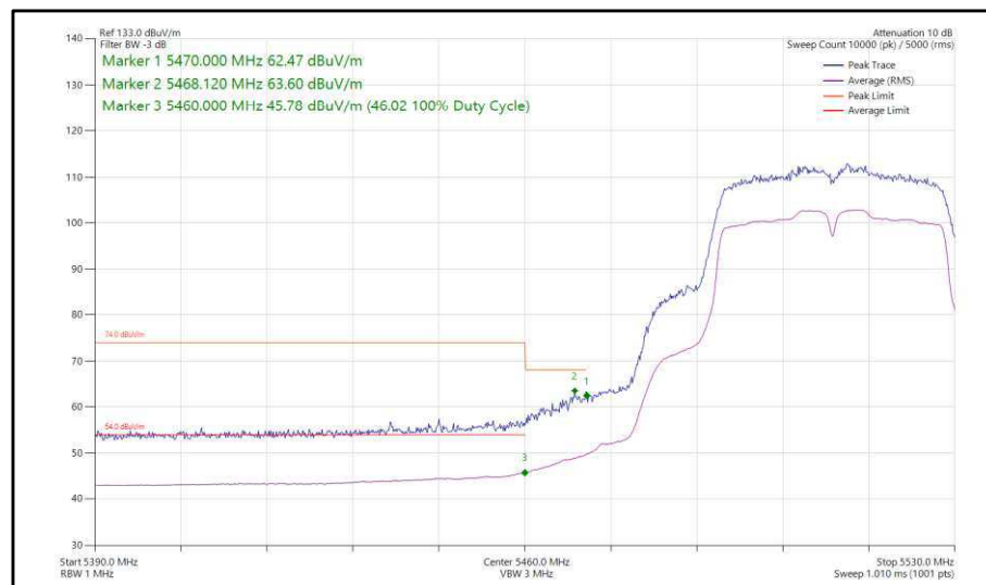
Figure 361 - 802.11n, HT40, SISO, Core 0 - 5510 MHz, Band Edge Frequency 5470 MHz
