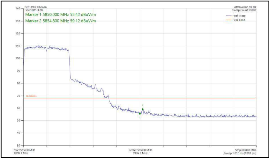
Figure 443 - 802.11ac, VHT80, SISO, Core 0 - 5690 MHz, Band Edge Frequency 5850 MHz
