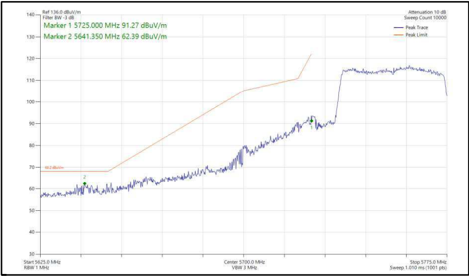
Figure 427 - 802.11ax, HE40, SU, TxBF, Core 0-1 - 5755 MHz, Band Edge Frequency 5725 MHz
