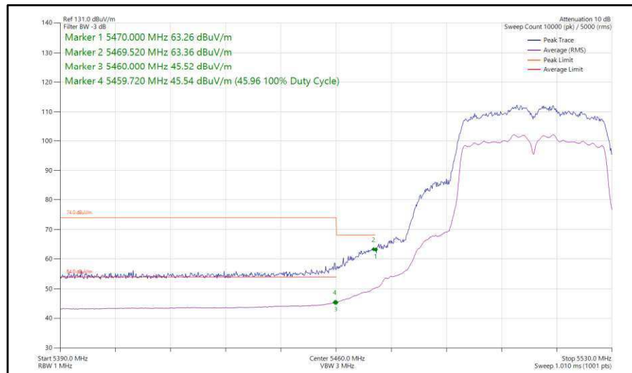
Figure 391 - 802.11n, HT40, CDD, Core 0-1 - 5510 MHz, Band Edge Frequency 5470 MHz
