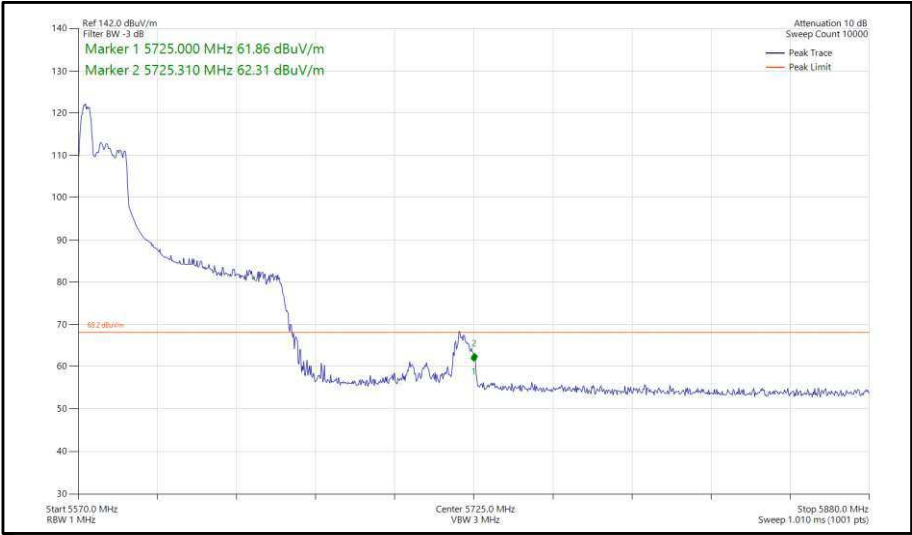
Figure 457 - 802.11ax, HE80, RU 52-37, SISO, Core 1 - 5610 MHz, Band Edge Frequency 5725 MHz
