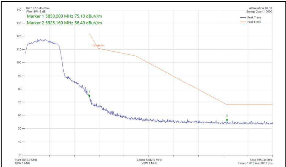
Figure 314 - 802.11n, HT20, SISO, Core 1 - 5825 MHz, Band Edge Frequency 5850 MHz
