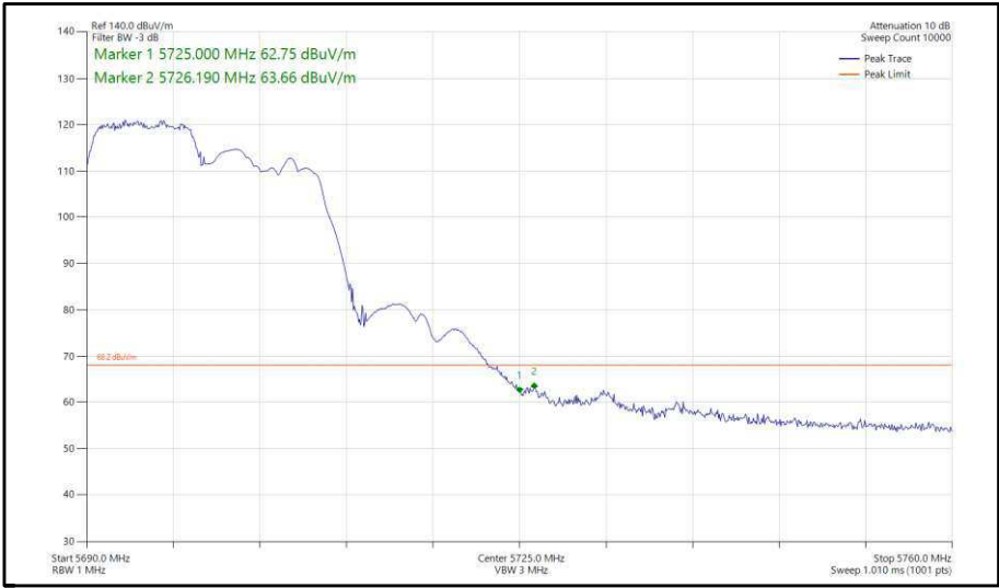
Figure 328 - 802.11ax, HE20, RU 106-53, CDD, Core 0-1 - 5700 MHz, Band Edge Frequency 5725 MHz
