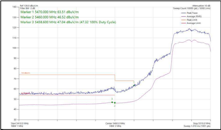
Figure 320 - 802.11ax, HE20, SU, CDD, Core 0-1 - 5500 MHz, Band Edge Frequency 5470 MHz
