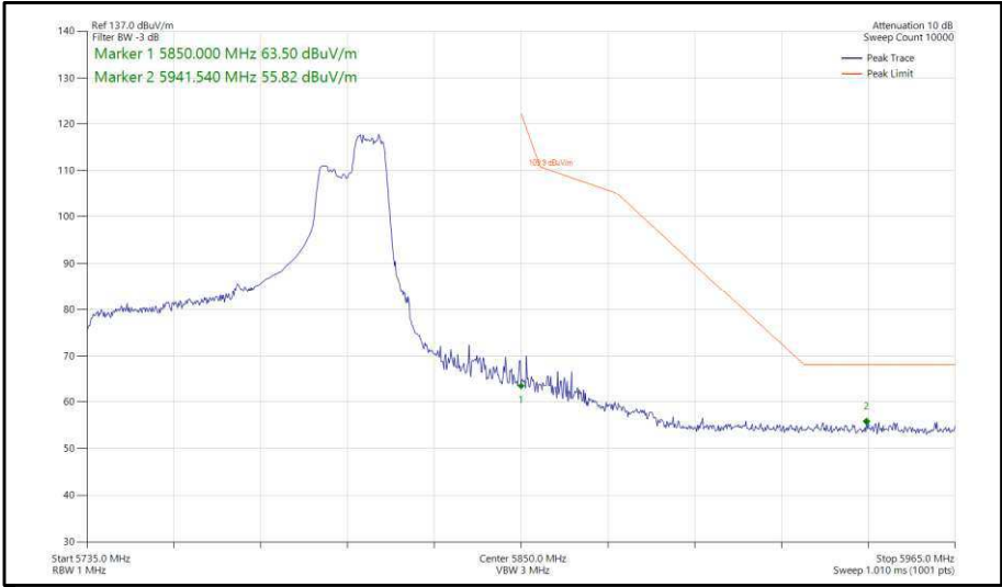
Figure 448 - 802.11ax, HE80, RU 106-60, SISO, Core 0 - 5775 MHz, Band Edge Frequency 5850 MHz
