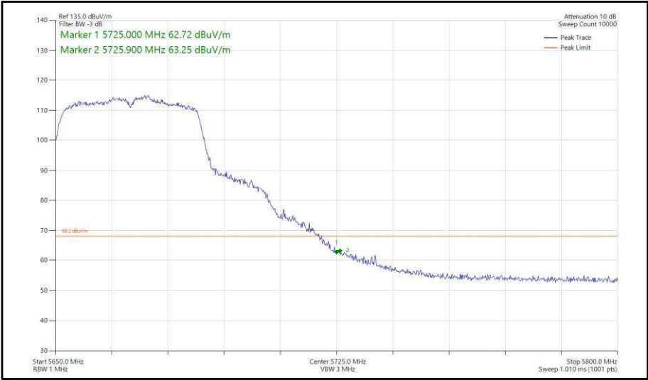
Figure 367 - 802.11n, HT40, SISO, Core 0 - 5670 MHz, Band Edge Frequency 5725 MHz
