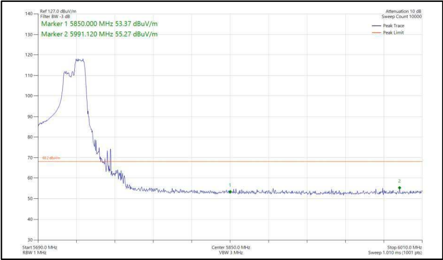
Figure 373 - 802.11ax, HE40, RU 106-56, SISO, Core 0 - 5710 MHz, Band Edge Frequency 5850 MHz
