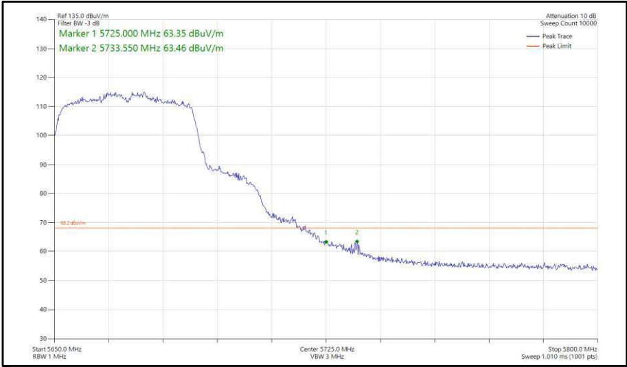
Figure 382 - 802.11n, HT40, SISO, Core 1 - 5670 MHz, Band Edge Frequency 5725 MHz
