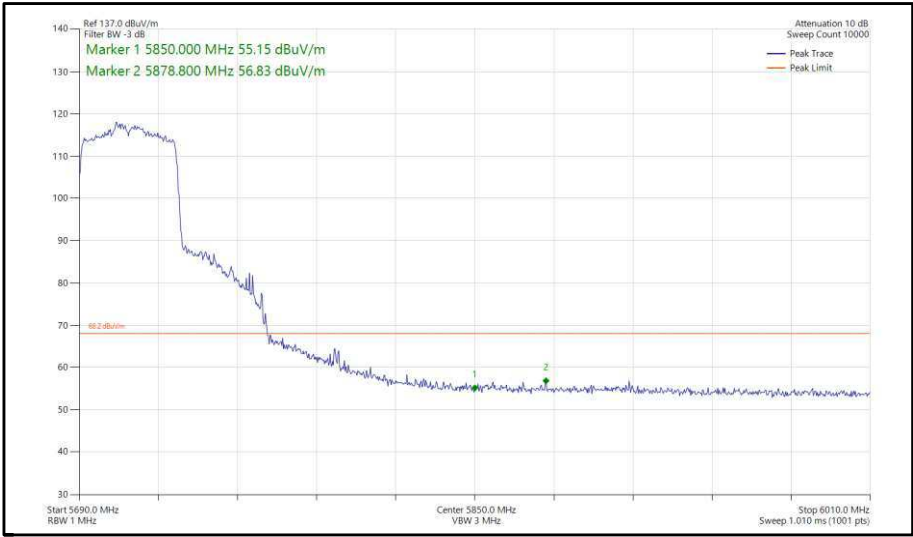
Figure 420 - 802.11ax, HE40, SU, SDM, Core 0-1 - 5710 MHz, Band Edge Frequency 5850 MHz
