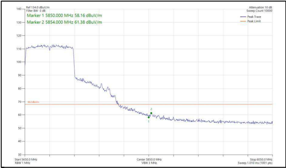
Figure 458 - 802.11ac, VHT80, SISO, Core 1 - 5690 MHz, Band Edge Frequency 5850 MHz
