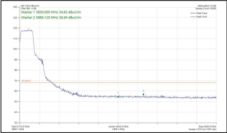
Figure 345 - 802.11n, HT20, SDM, Core 0-1 - 5720 MHz, Band Edge Frequency 5850 MHz
