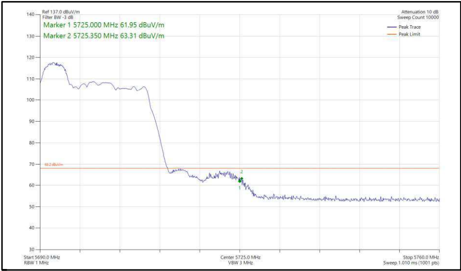
Figure 344 - 802.11ax, HE20, RU 52-37, SDM, Core 0-1 - 5700 MHz, Band Edge Frequency 5725 MHz
