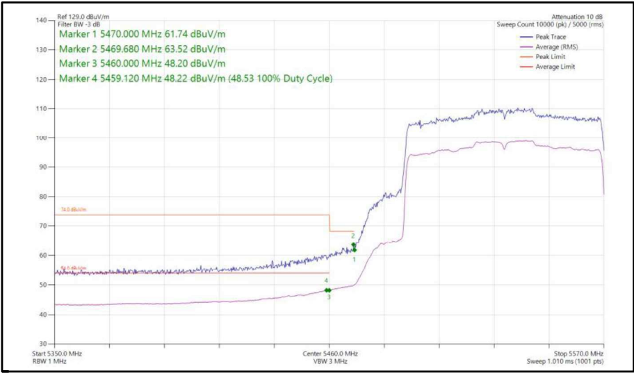
Figure 435 - 802.11ax, HE80, SU, SISO, Core 0 - 5530 MHz, Band Edge Frequency 5470 MHz
