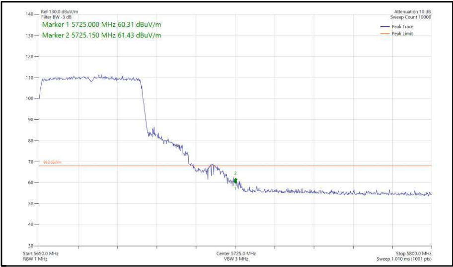
Figure 429 - 802.11ax, HE40, SU, TxBF, Core 0-1 - 5670 MHz, Band Edge Frequency 5725 MHz
