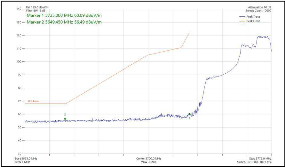
Figure 381 - 802.11ax, HE40, RU 106-56, SISO, Core 1 - 5755 MHz, Band Edge Frequency 5725 MHz
