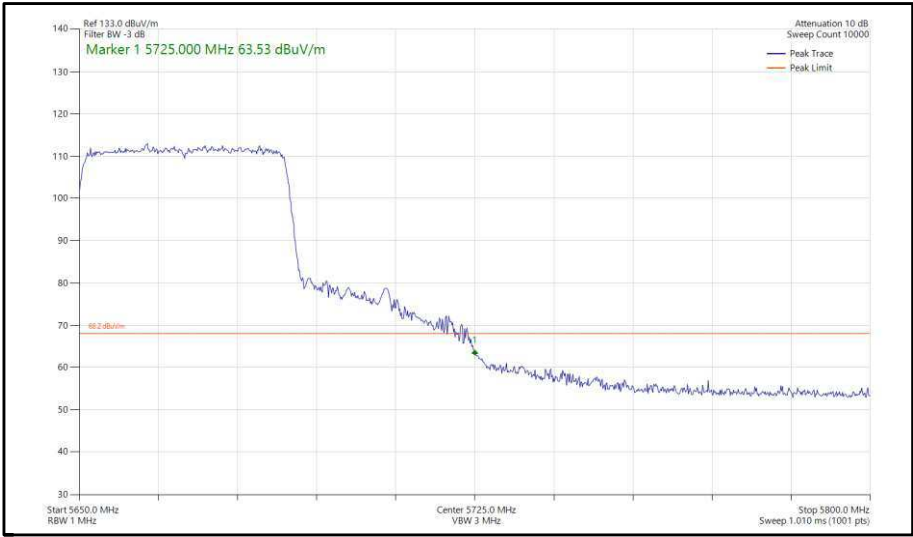
Figure 383 - 802.11ax, HE40, SU, SISO, Core 1 - 5670 MHz, Band Edge Frequency 5725 MHz
