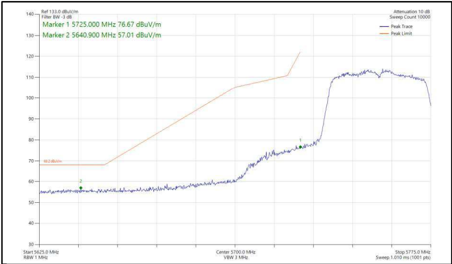
Figure 364 - 802.11n, HT40, SISO, Core 0 - 5755 MHz, Band Edge Frequency 5725 MHz
