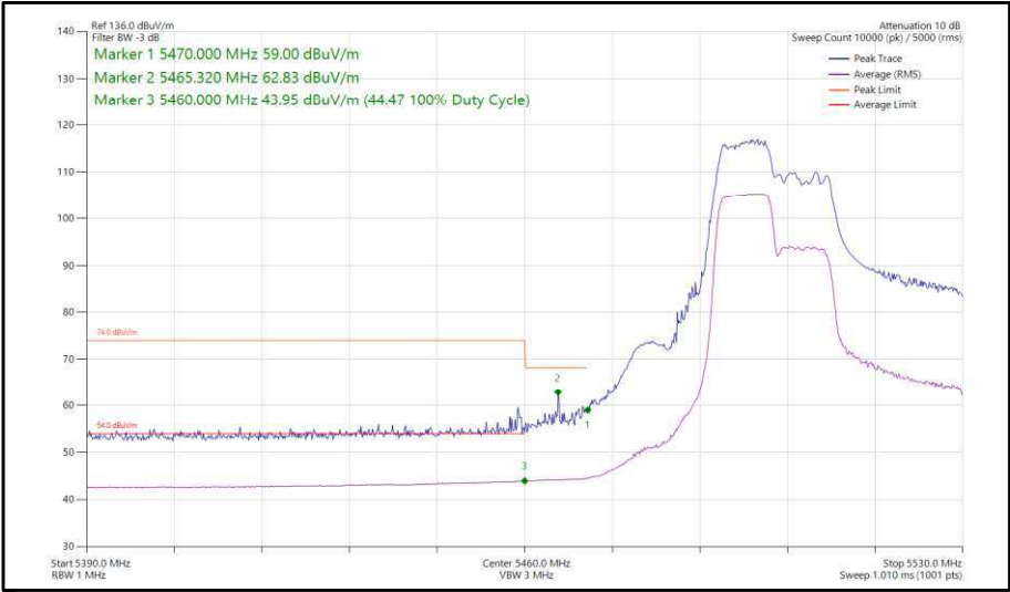
Figure 363 - 802.11ax, HE40, RU 106-53, SISO, Core 0 - 5510 MHz, Band Edge Frequency 5470 MHz
