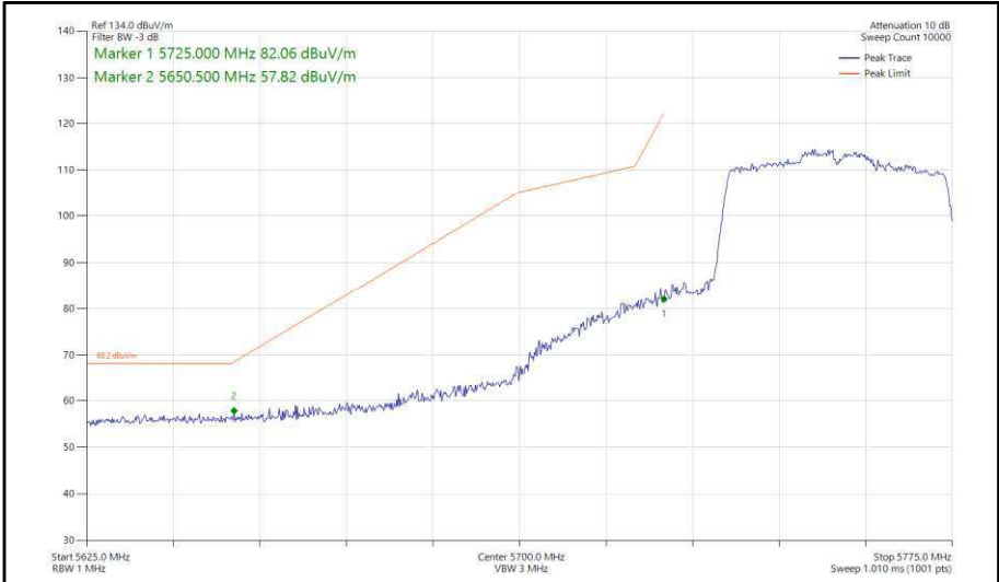
Figure 365 - 802.11ax, HE40, SU, SISO, Core 0 - 5755 MHz, Band Edge Frequency 5725 MHz
