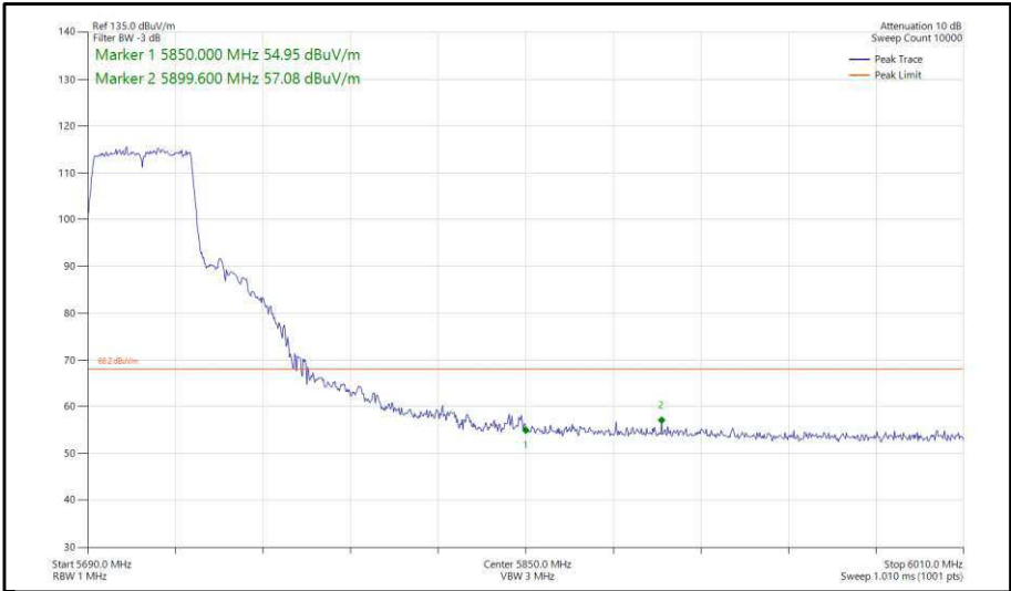
Figure 418 - 802.11n, HT40, SDM, Core 0-1 - 5710 MHz, Band Edge Frequency 5850 MHz
