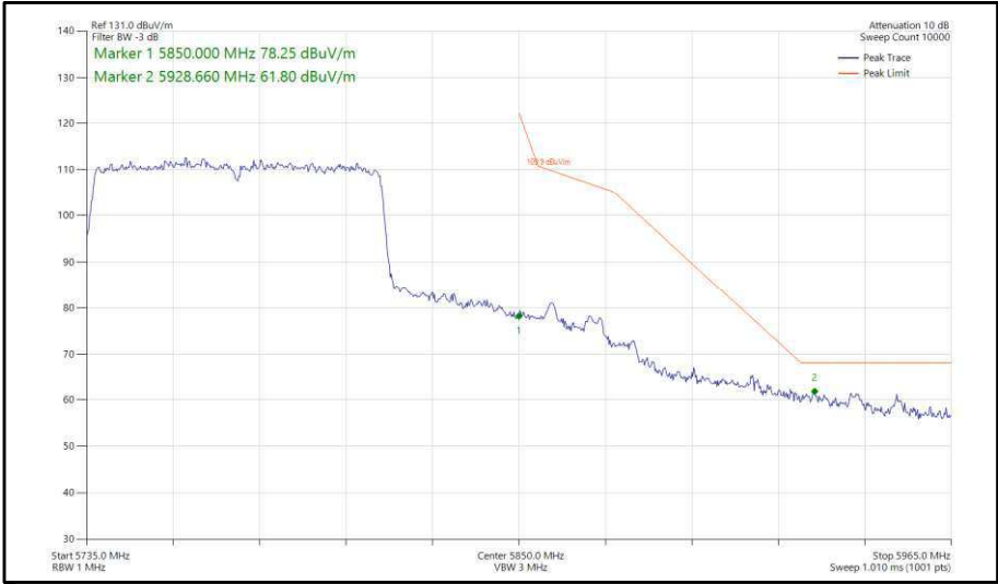
Figure 459 - 802.11ac, VHT80, SISO, Core 1 - 5775 MHz, Band Edge Frequency 5850 MHz
