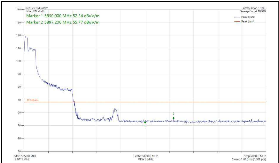
Figure 446 - 802.11ax, HE80, RU 52-37, SISO, Core 0 - 5690 MHz, Band Edge Frequency 5850 MHz
