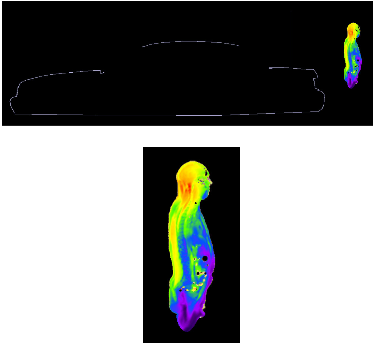
Figure 8. SAR distribution at 165.0125 MHz in the bystander model located at the 0 degree angle of the vehicle trunk, produced by the trunk-mount HAD4022A antenna. The SAR distribution plot is relative to the plane where the peak 1-g average SAR for this exposure condition occurs.
