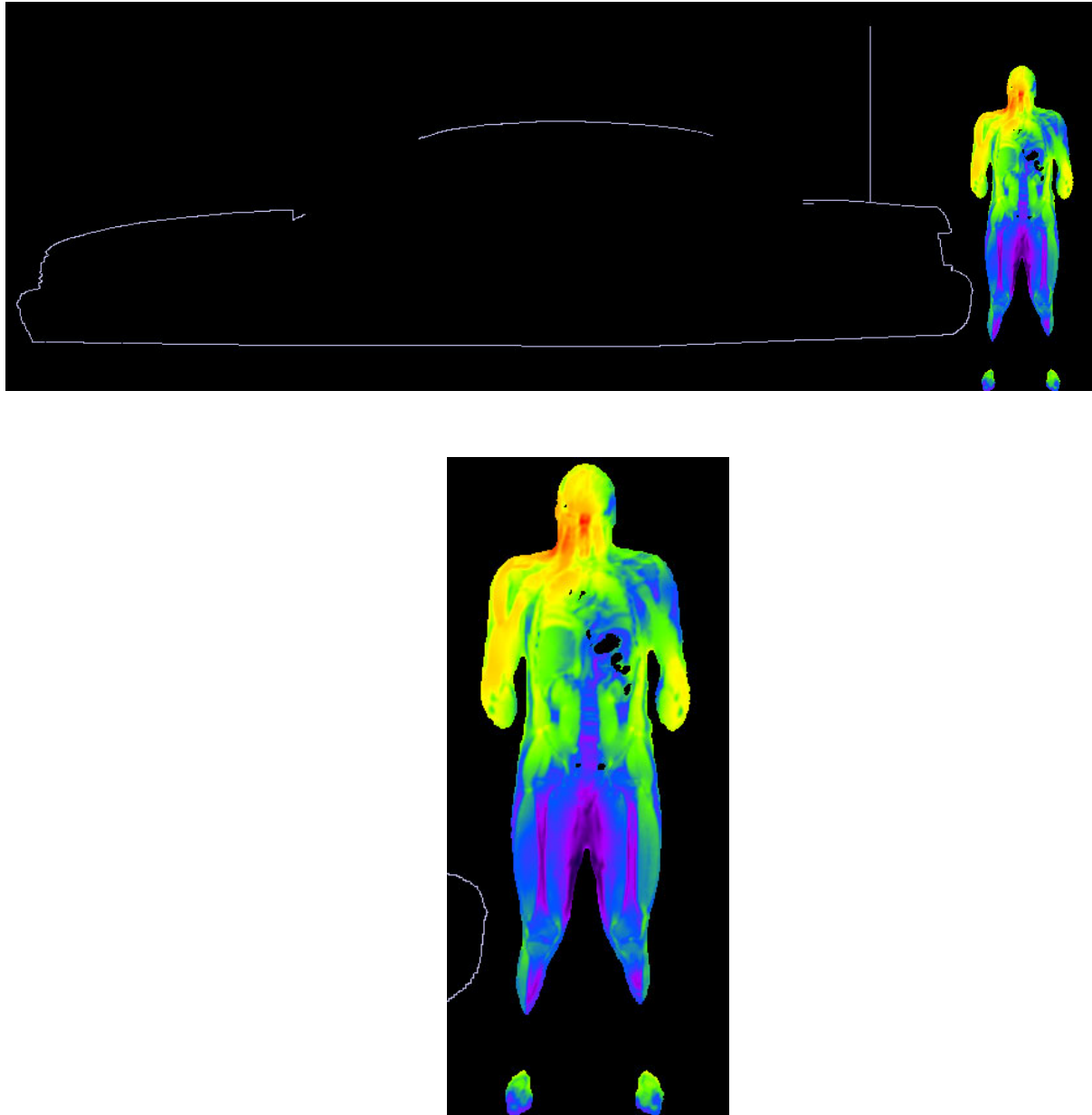
Figure 6. SAR distribution at 165.0125 MHz in the bystander model located at the 45 degree angle of the vehicle trunk, produced by the trunk-mount HAD4022A antenna. The SAR distribution plot is relative to the plane where the peak 1-g average SAR for this exposure condition occurs.
