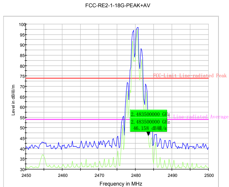
Fig.68. Radiated emission (Power) GFSK, high channel
