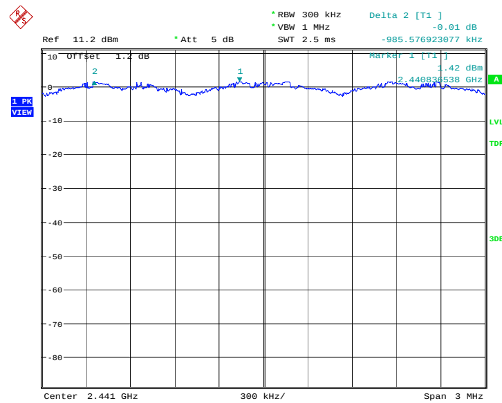
Fig.122. Carrier frequency separation measurement: \pi/4 DQPSK, Channel 39
