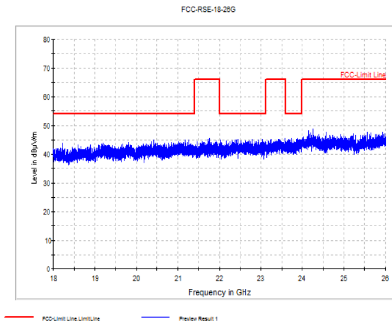
Fig.93. Radiated emission: 8DPSK, 18 GHz - 26 GHz
