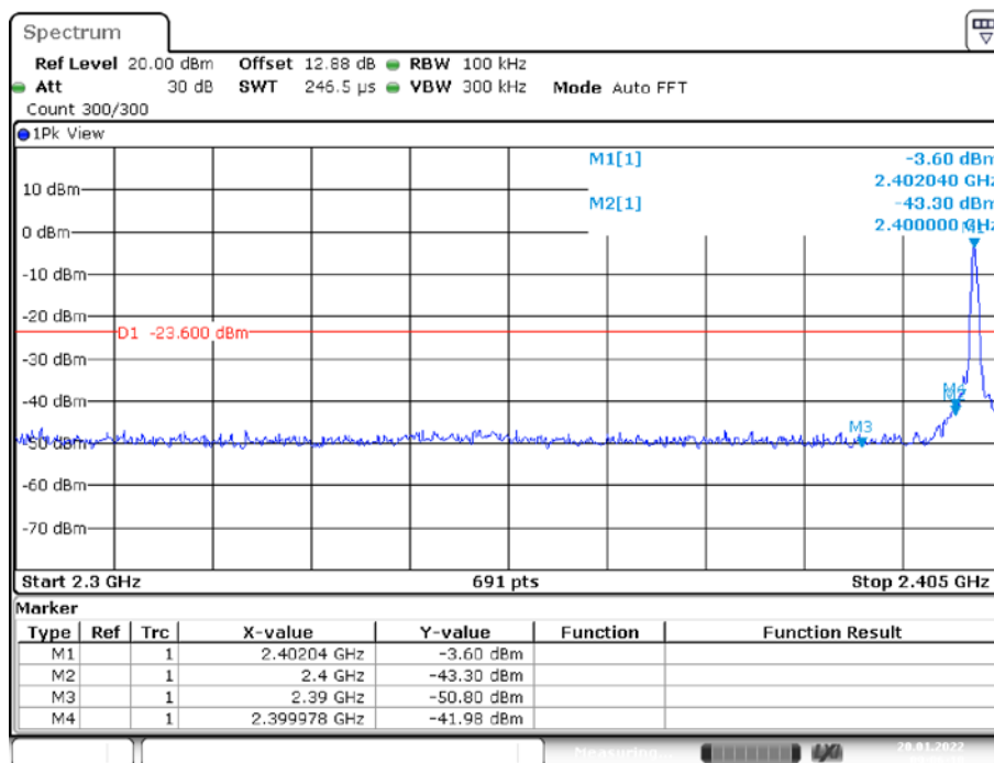
BLE_1M_Ant1_Low_2402
