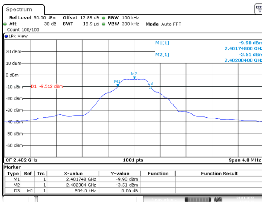
BLE_1M_Ant1_2402
