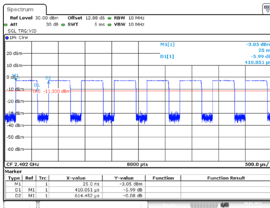
BLE_BT4.0_Ant1_2402
