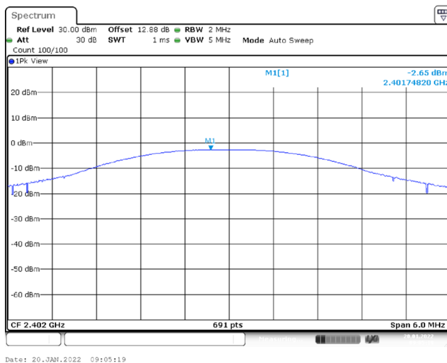
BLE_1M_Ant1_2402
