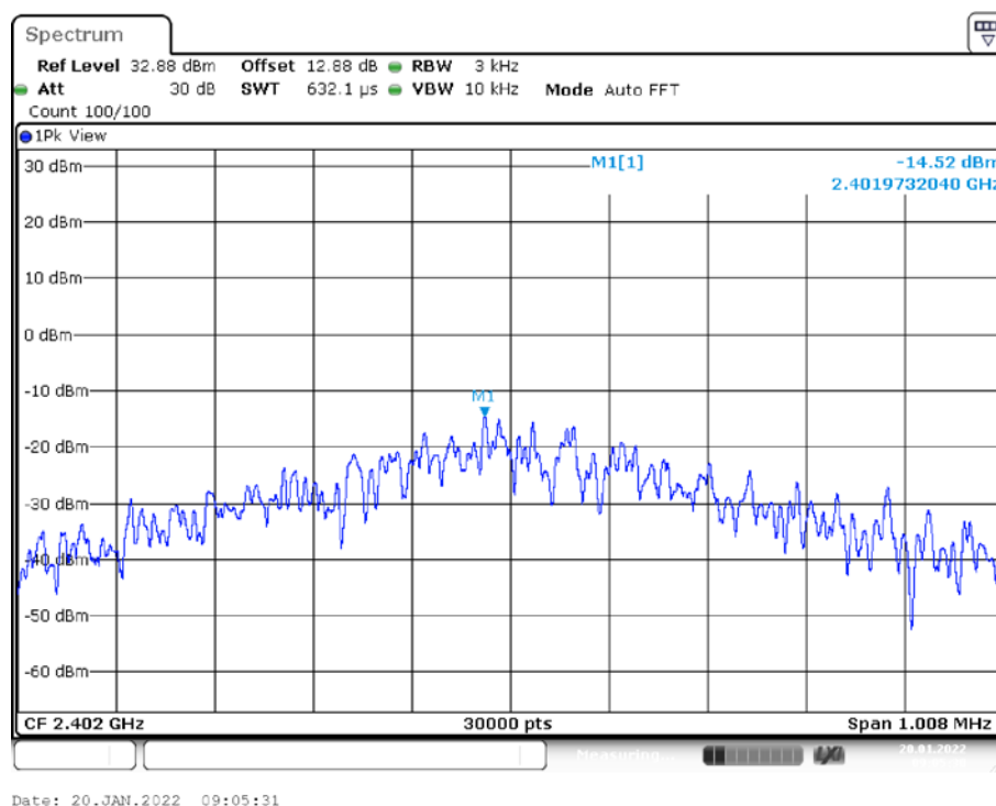
BLE_1M_Ant1_2402
