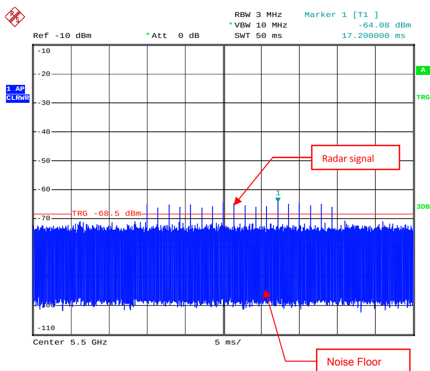
Radar Signal 1
