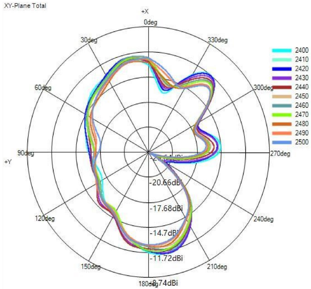
(3) X-Y Plane(unit:dBi):
