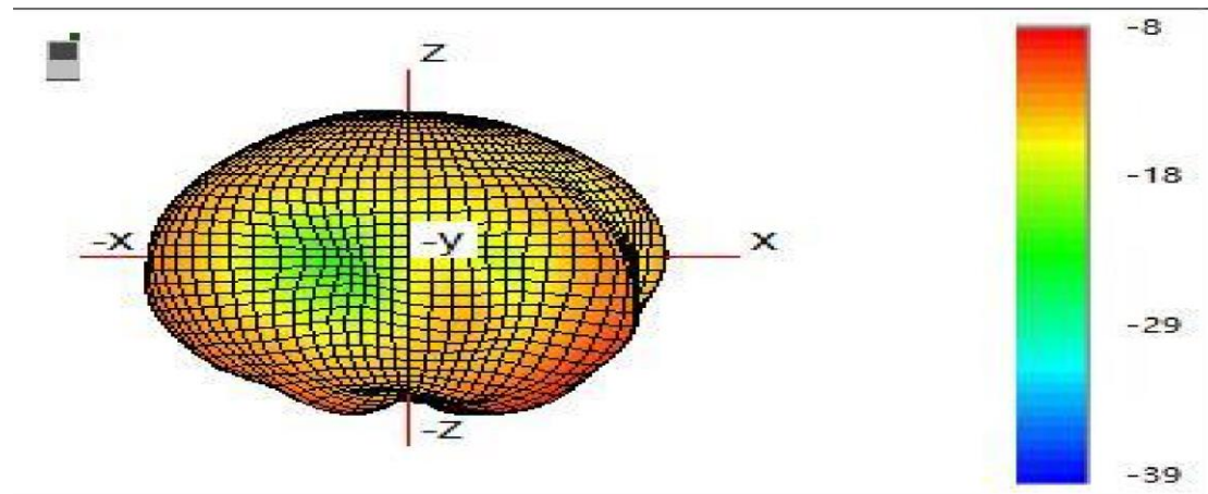
(4) Typical Free Space 3D Radiation Pattern at 2.44GHz(unit:dBi):
