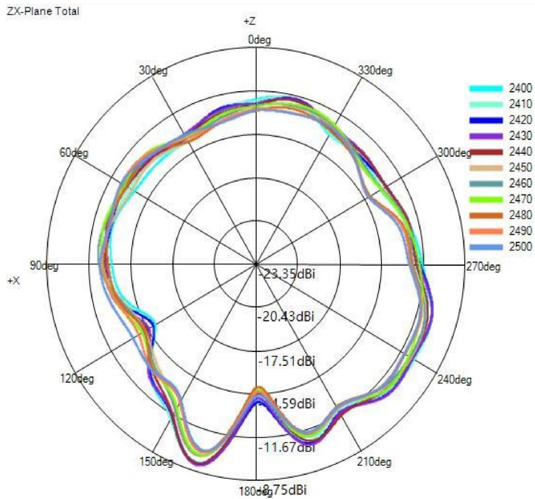
(1) X-Z Plane(unit:dBi):
