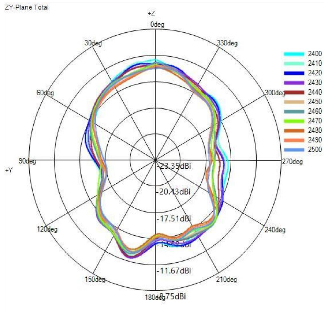
(2) Y-Z Plane(unit:dBi):
