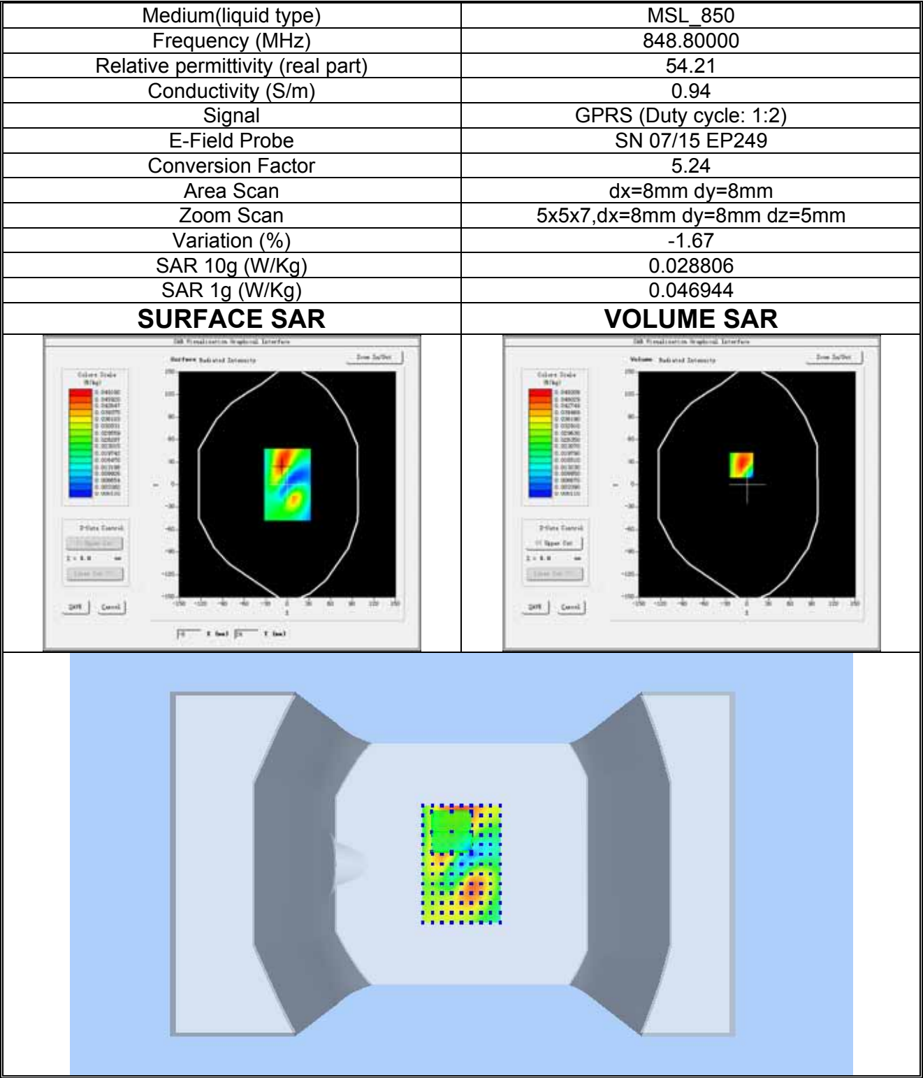
Plot 8: GPRS850MHz, High channel(Body-worn, Bottom edge) Product Description: MOBILE PHONE Test Date: 2018-07-04
