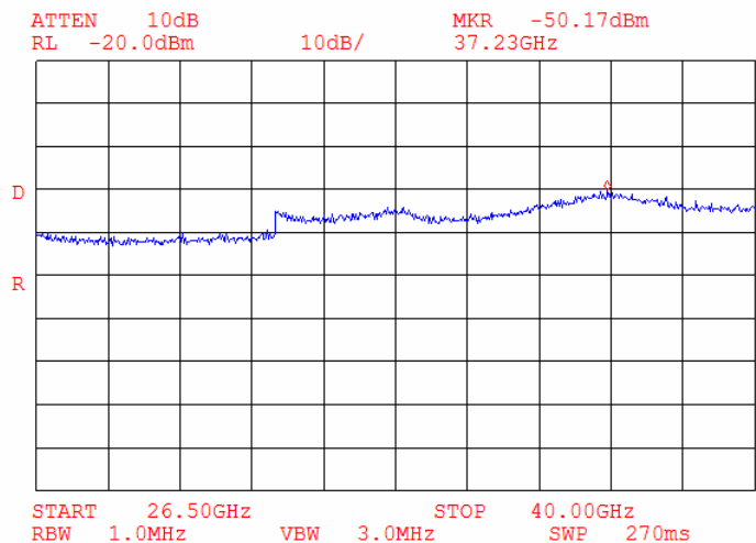
Plot 7.3.30 Spurious emission measurements in 26.5 - 40 GHz range at high carrier frequency
