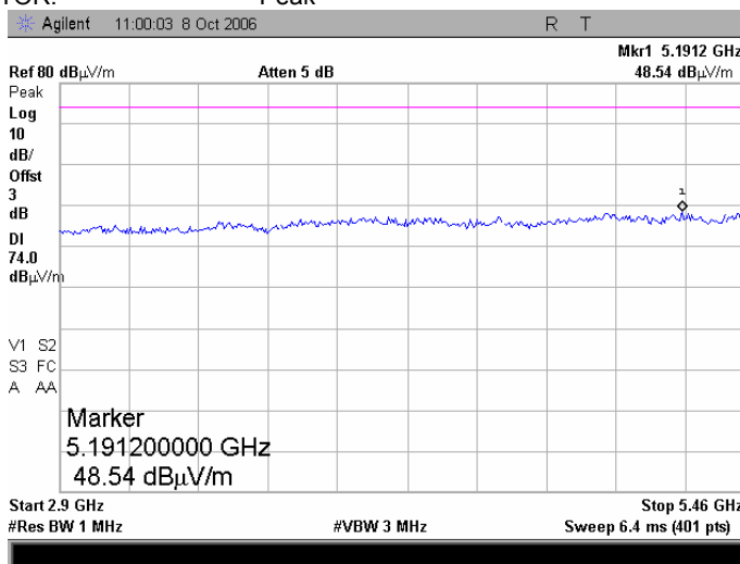
Plot 7.4.17 Radiated emission measurements from 2900 to 5460 MHz at the low carrier frequency, 10 MHz BW
