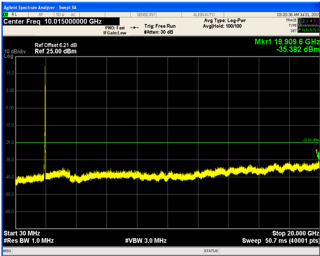
LTE Band1 QAM16 BW=5MHz Channel=18025 RB Size=25 Position=#0
