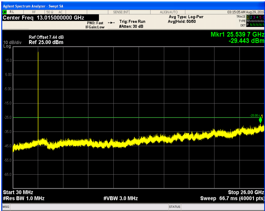
LTE Band41 QAM16 BW=5MHz Channel=41165 RB Size=25 Position=#0
