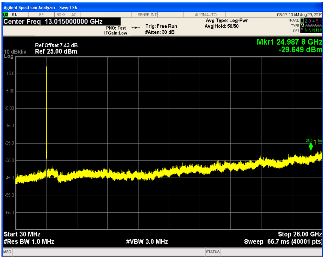
LTE Band41 QAM16 BW=10MHz Channel=41140 RB Size=50 Position=#0
