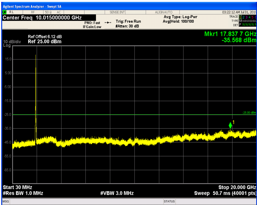
LTE Band1 QPSK BW=5MHz Channel=18575 RB Size=25 Position=#0
