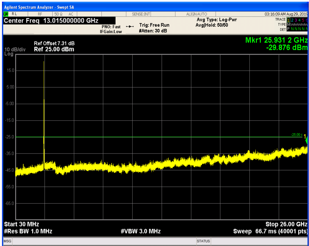
LTE Band41 QAM16 BW=10MHz Channel=40290 RB Size=50 Position=#0
