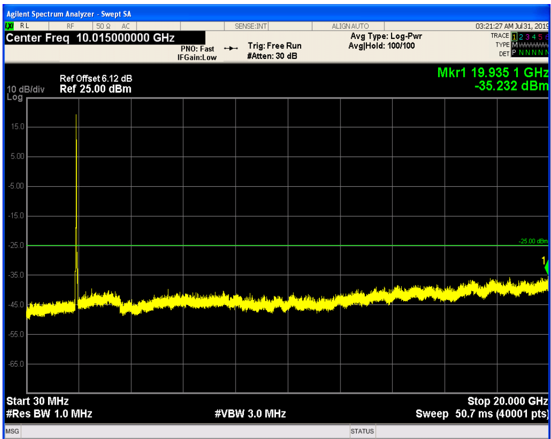
LTE Band1 QPSK BW=15MHz Channel=18525 RB Size=75 Position=#0
