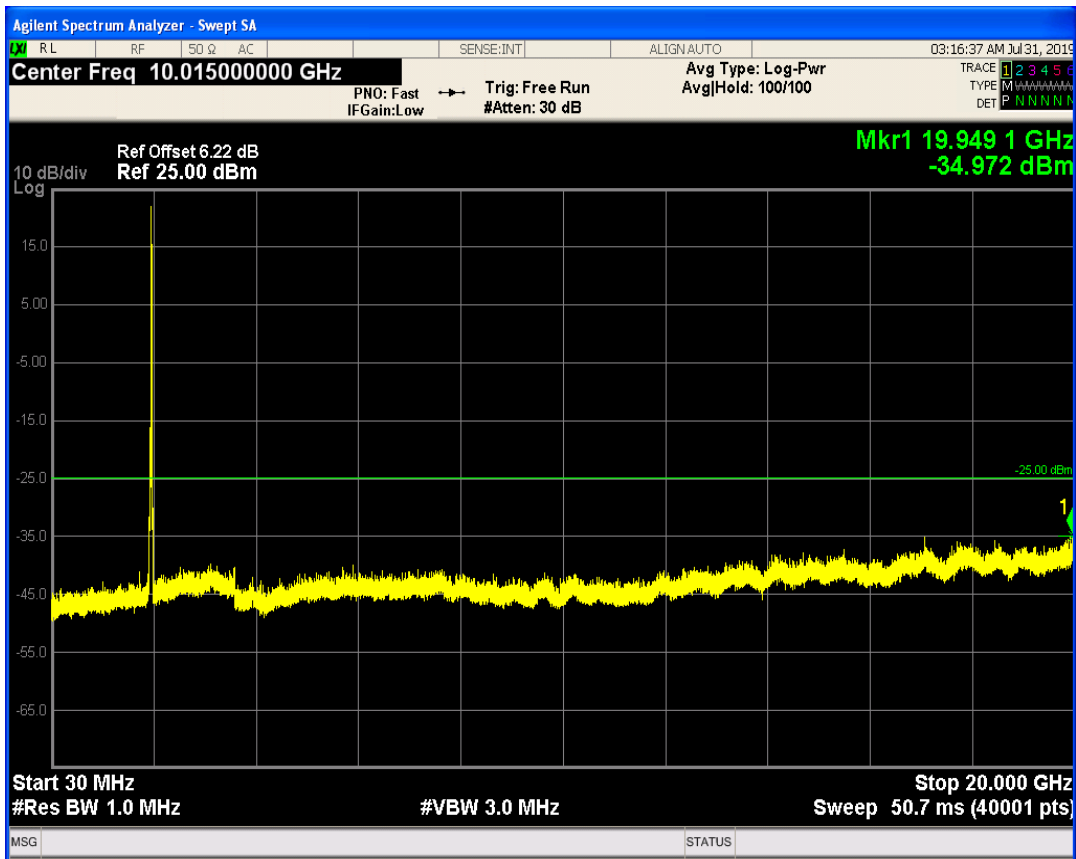
LTE Band1 QPSK BW=10MHz Channel=18050 RB Size=50 Position=#0
