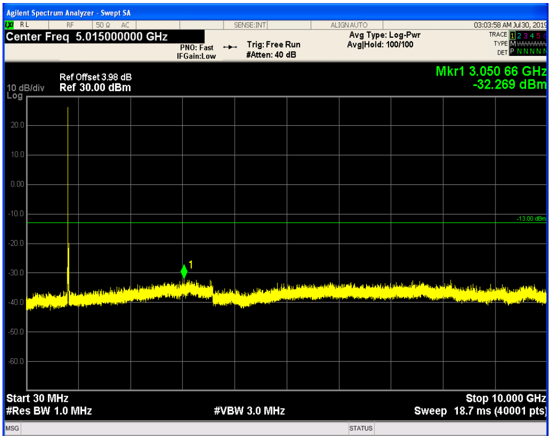
LTE Band1 QPSK BW=10MHz Channel=18550 RB Size=50 Position=#0
