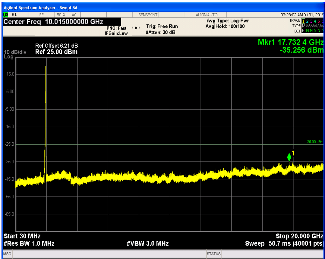
LTE Band1 QPSK BW=20MHz Channel=18100 RB Size=100 Position=#0
