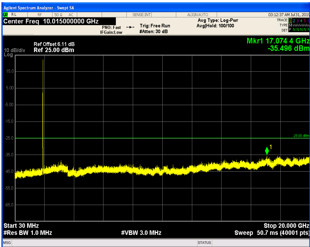
LTE Band1 QAM16 BW=20MHz Channel=18500 RB Size=100 Position=#0
