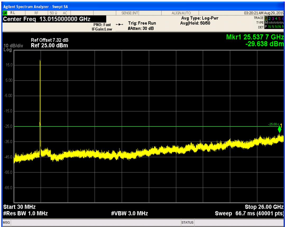
LTE Band41 QAM16 BW=20MHz Channel=40340 RB Size=100 Position=#0
