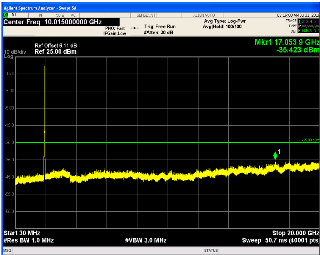
LTE Band1 QAM16 BW=10MHz Channel=18550 RB Size=50 Position=#0
