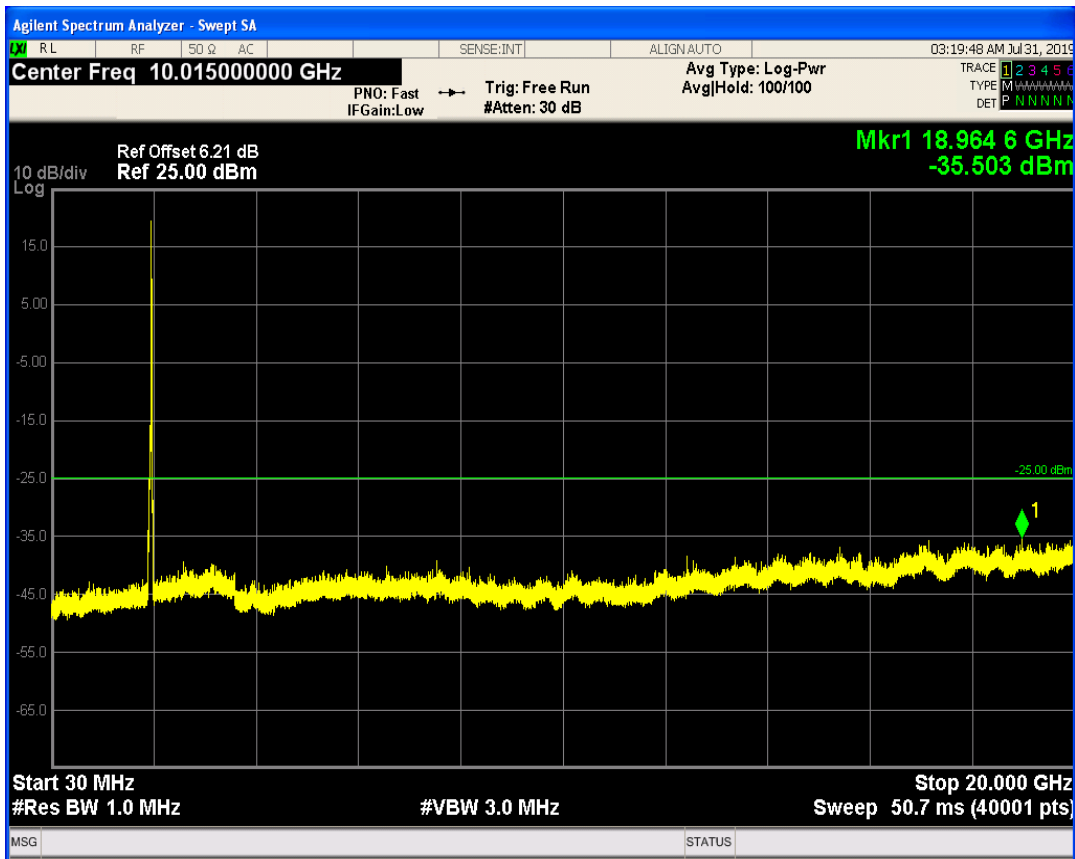
LTE Band1 QAM16 BW=15MHz Channel=18075 RB Size=75 Position=#0
