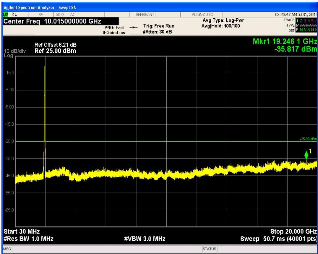
LTE Band1 QAM16 BW=20MHz Channel=18100 RB Size=100 Position=#0
