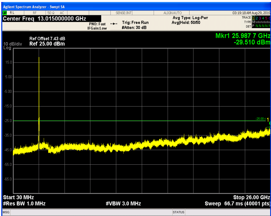
LTE Band41 QPSK BW=20MHz Channel=40340 RB Size=100 Position=#0
