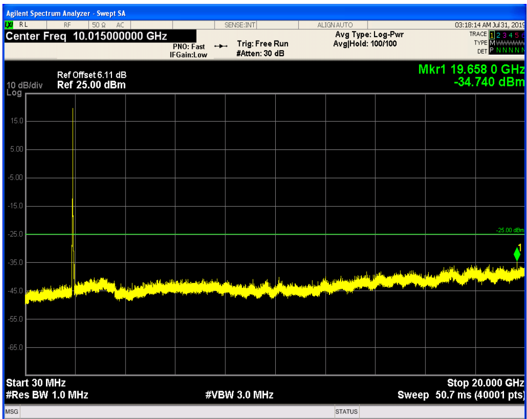
LTE Band1 QPSK BW=20MHz Channel=18500 RB Size=100 Position=#0
