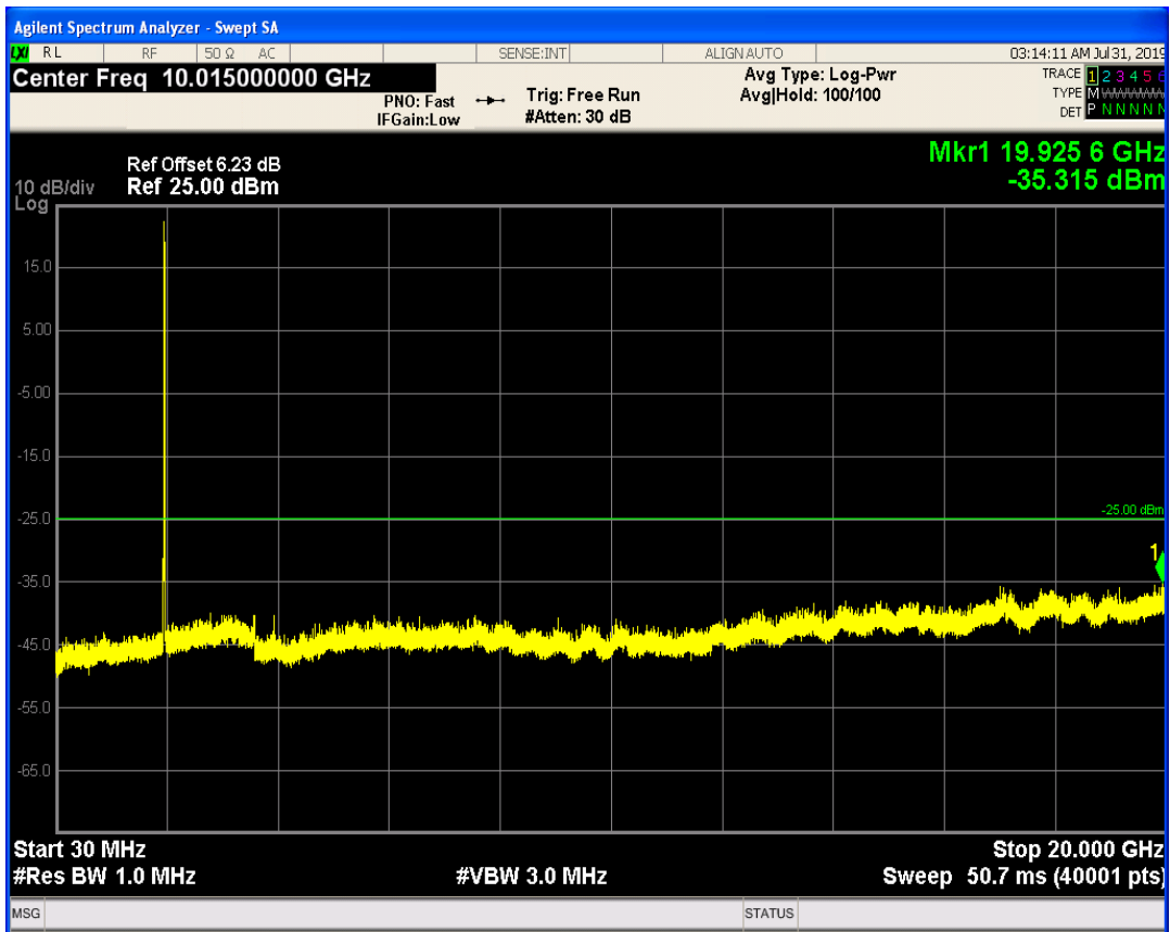
LTE Band1 QPSK BW=15MHz Channel=18075 RB Size=75 Position=#0
