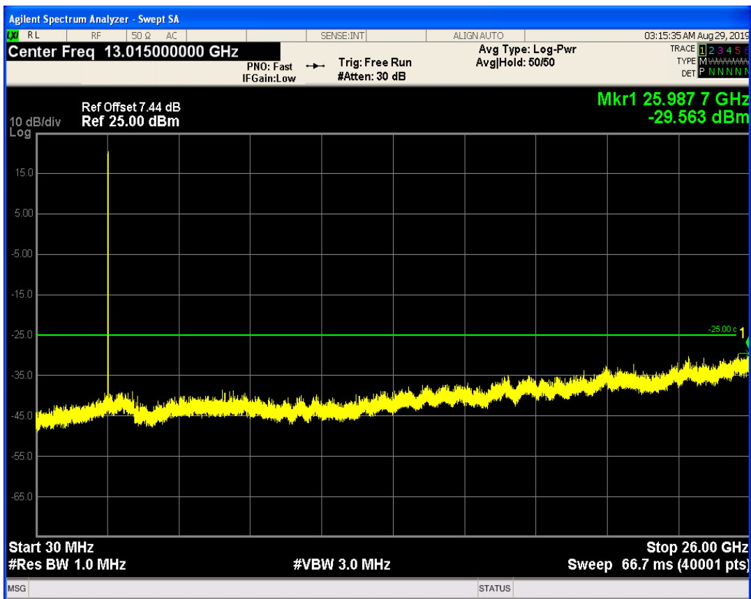
LTE Band41 QPSK BW=10MHz Channel=40290 RB Size=50 Position=#0
