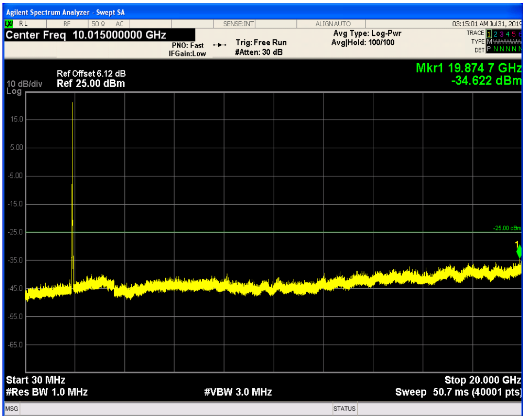
LTE Band1 QAM16 BW=5MHz Channel=18575 RB Size=25 Position=#0
