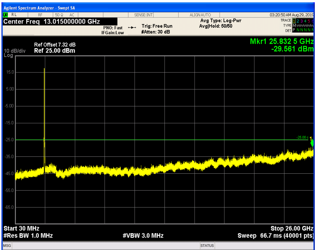
LTE Band41 QPSK BW=20MHz Channel=41090 RB Size=100 Position=#0
