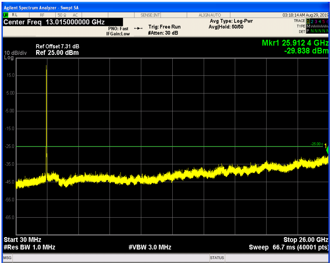
LTE Band41 QAM16 BW=15MHz Channel=40315 RB Size=75 Position=#0
