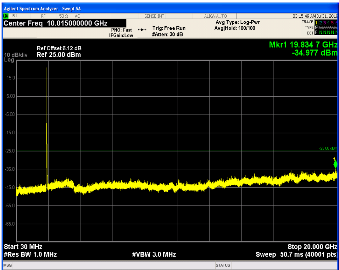
LTE Band1 QAM16 BW=15MHz Channel=18525 RB Size=75 Position=#0
