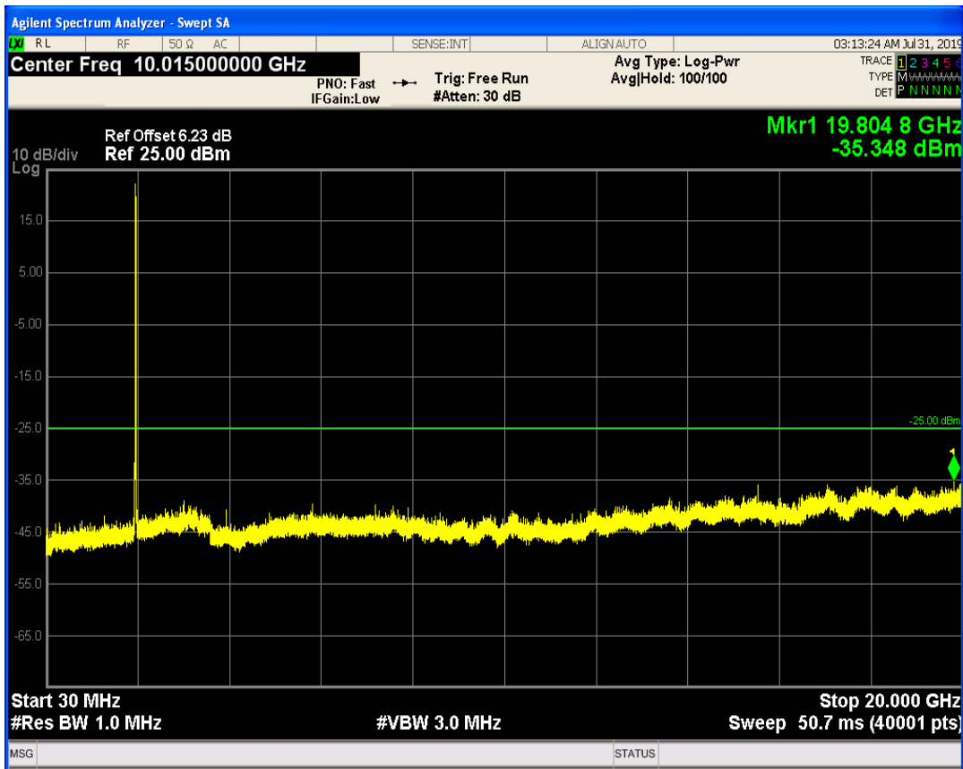
LTE Band1 QPSK BW=5MHz Channel=18025 RB Size=25 Position=#0
