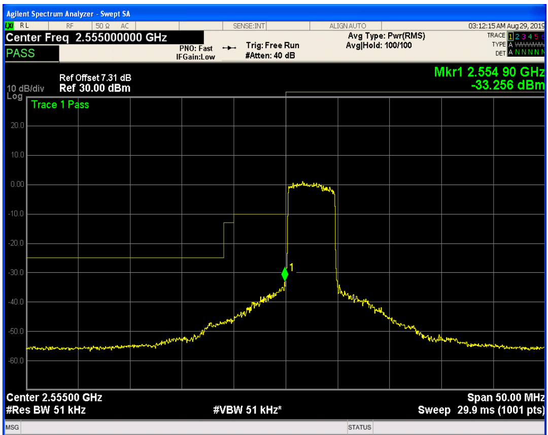
LTE Band41 QAM16 BW=5MHz Channel=40265 RB Size=25 Position=#0
