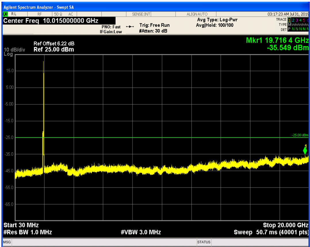
LTE Band1 QAM16 BW=10MHz Channel=18050 RB Size=50 Position=#0
