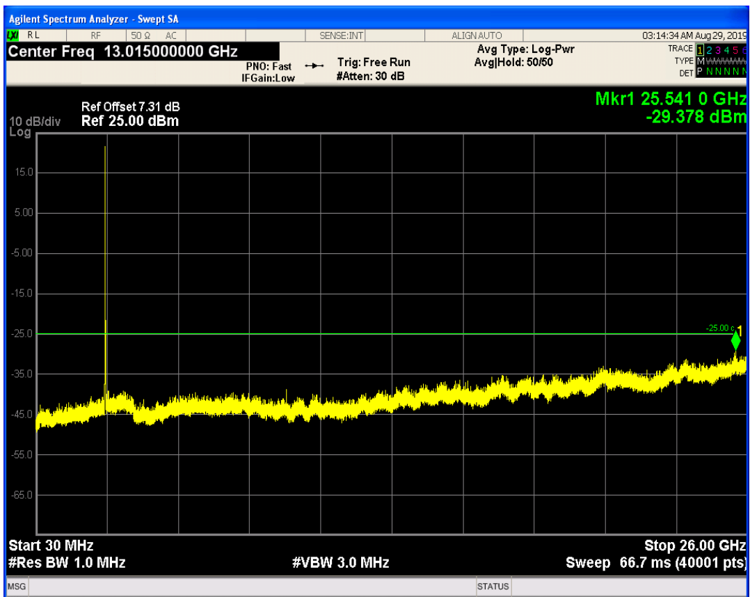
LTE Band41 QPSK BW=5MHz Channel=41165 RB Size=25 Position=#0
