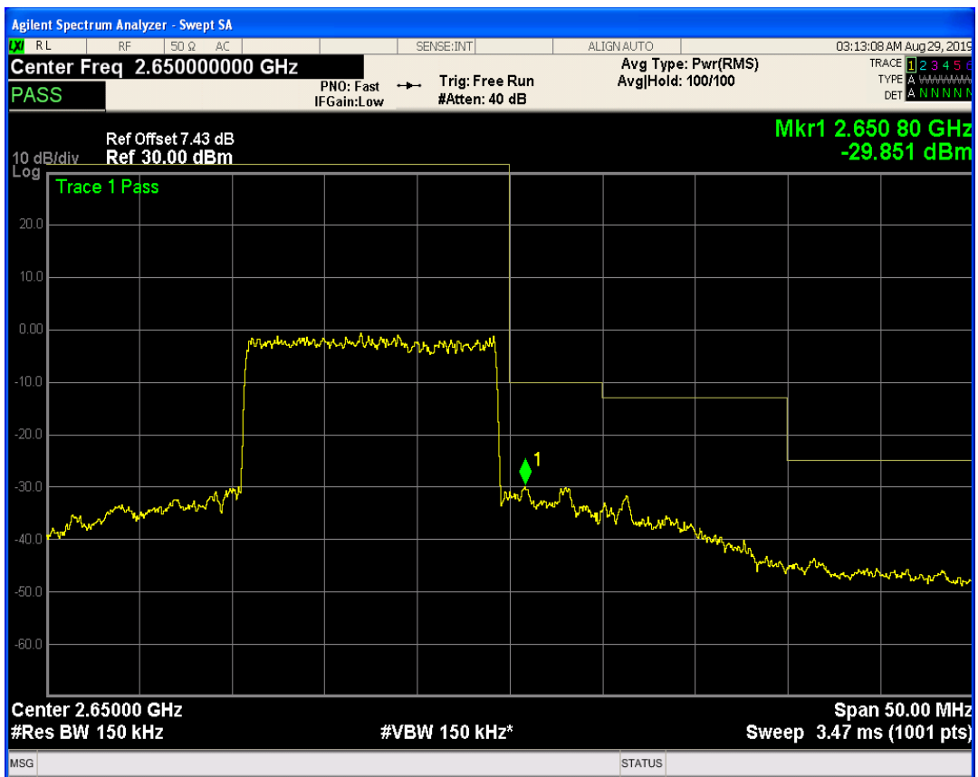
LTE Band41 QAM16 BW=15MHz Channel=41115 RB Size=75 Position=#0
