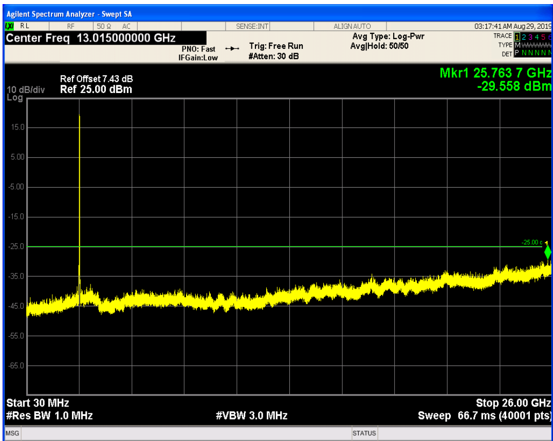
LTE Band41 QPSK BW=15MHz Channel=40315 RB Size=75 Position=#0
