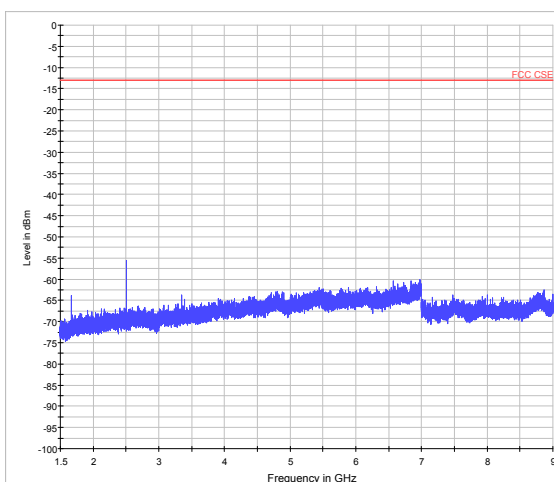
LTE Band 5 1.4MHz CH-High 1.5GHz~9GHz
