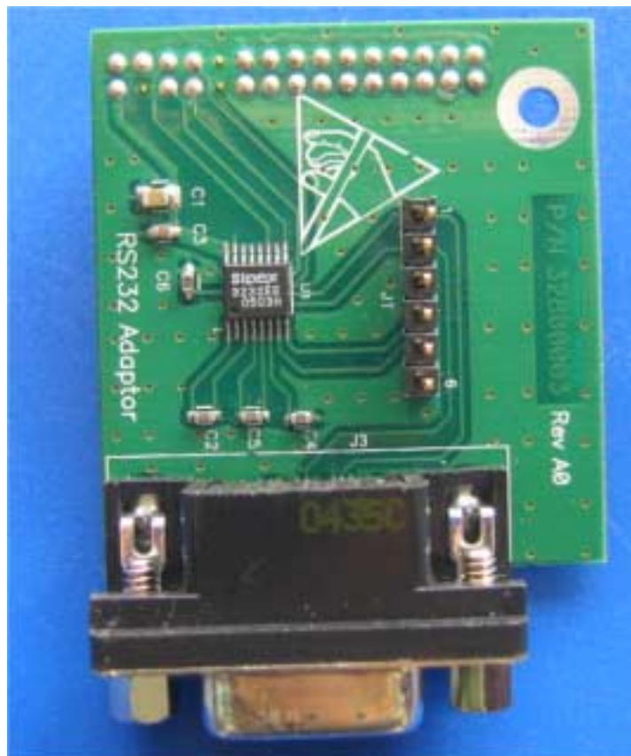
Photograph No.5 EasyST RS232 adapter view
